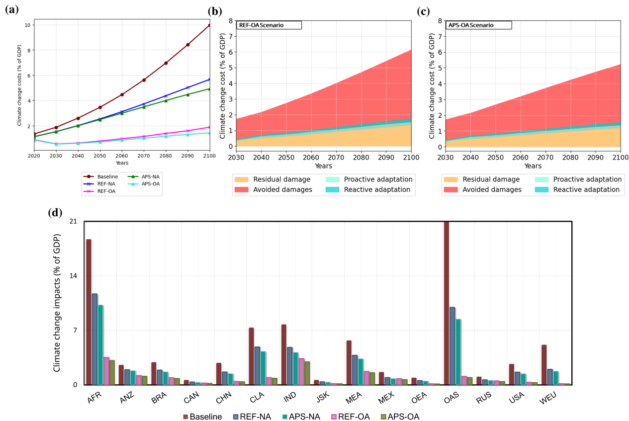
Figure 10. (a) Global total climate change impacts; (b) impacts components in REF-REF-OA and (c) APS-APS-OA scenario; and (d) regional climate impacts in 2100 as a percentage of GDP.
