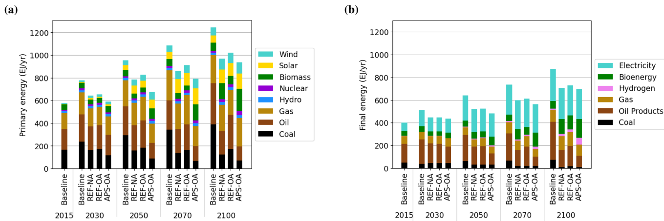
Figure 8. (a) Primary energy supply mixes by sources (b) final energy use by sources for all scenarios.
