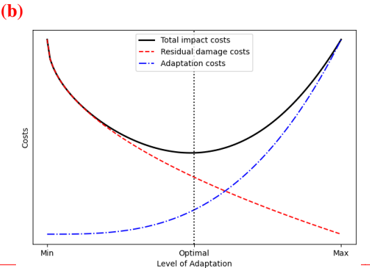
(a) Regional climate change damage curves. (b) Conceptual illustration of an adaptation cost curve adopted from Patt et al. (2010). The shapes of the curves are theoretical and do not reflect specific empirical estimates.
