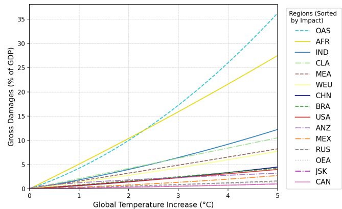
Figure D1. Regional climate change damage curves.
