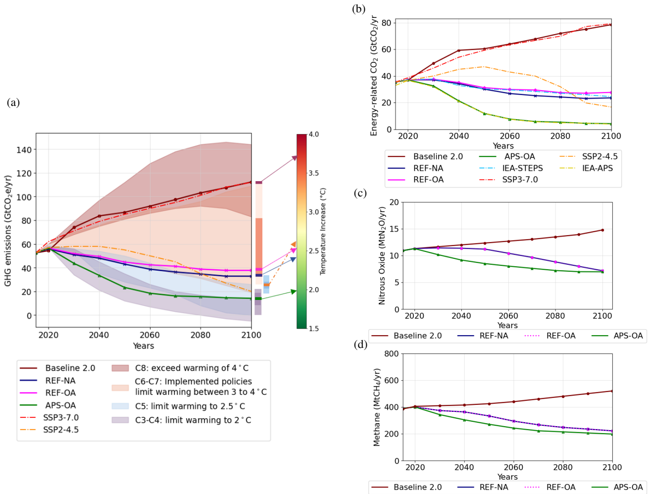
Figure 7. Projected anthropogenic emissions of primary climate change drivers; (a) Total GHG emissions (b) energy-related CO 2 emissions (c) total N 2 O emissions, and (d) total CH 4 emissions comparison across various scenarios: AD-MERGE 2.0 (Baseline 2.0, REF-NA, REF-OA and APS-OA), two IPCC representative pathways (SSP2-4.5 and SSP3-7.0), and IEA scenarios (IEA-STEPS and IEA-APS). Shaded patterns represent the C8 to C3 warming levels based on IPCC (2022a) classifications, providing a comparative context for emission trajectories. The ‘Implemented policies’ ranges show emissions pathways assuming policies implemented by the end of 2020 and pathways assuming implementation of NDCs before COP26. The gradient boxes show the 5th to 95th percentile of the projected warming levels in 2100. The figure also illustrates each scenario’s warming levels relative to the period 1850–1900.
