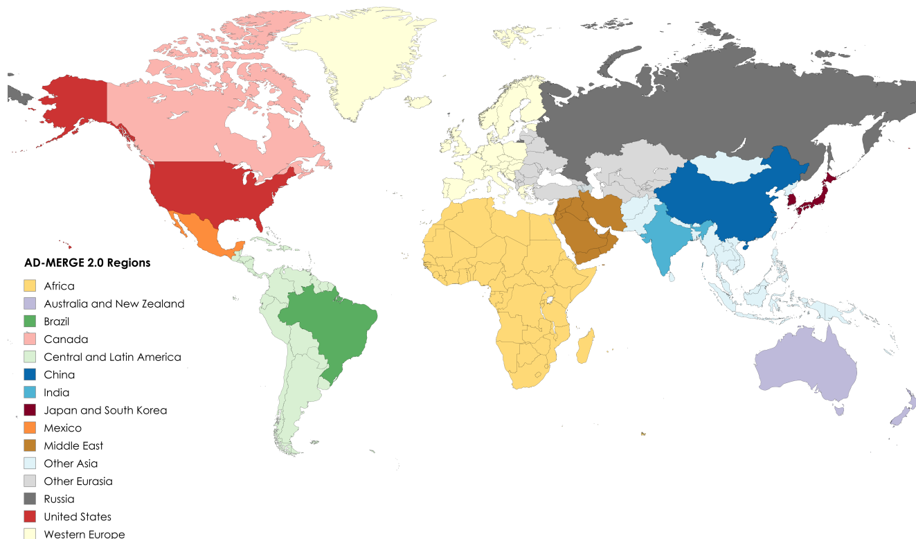
Figure 2. AD-MERGE 2.0 new regional disaggregation that considers 15 regions of individual countries or groups of countries. Created using MapChart ( https://www.mapchart.net/index.html ).
