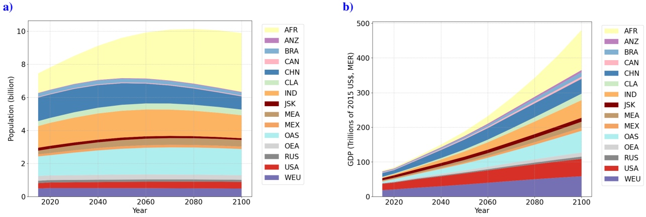
Figure A1. Regional (a) population and (b) GDP trajectories in AD-MERGE 2.0 from 2015 to 2100, based on SSP2 projections (IIASA, 2024).
