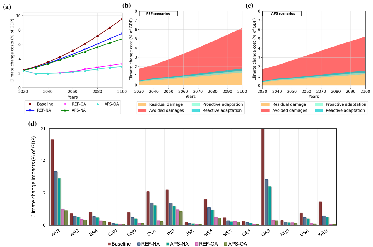
Figure 10. (a) Global total climate change impacts; (b) impacts components in REF-OA-REF and (c) APS-OA-APS scenario; and (d) regional climate damages-impacts in 2100 as a percentage of GDP.
