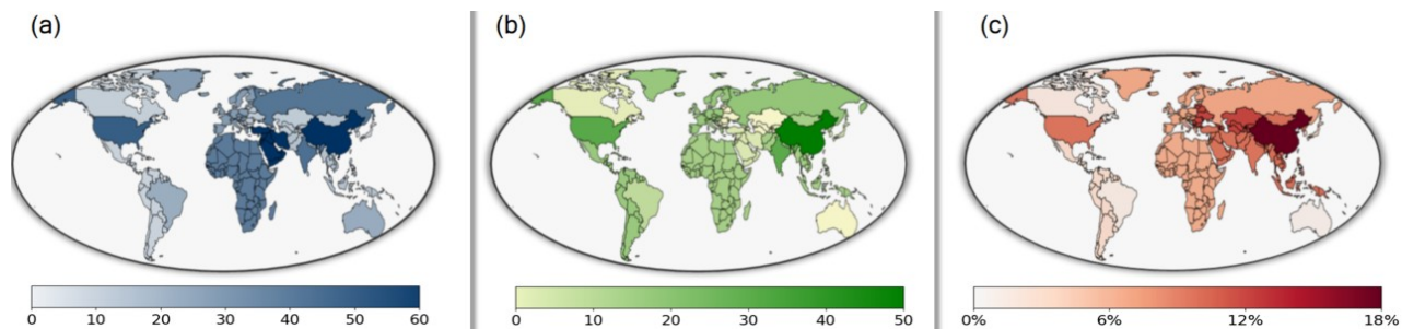
Figure F1. Regional trajectories of cumulative deployment of (a) direct air carbon capture and storage (DACCS) and (b) bioenergy with carbon capture and storage (BECCS), alongside (c) cumulative CO 2 emissions under the Announced Pledges Scenario (APS) for each region from 2015 to 2100.
