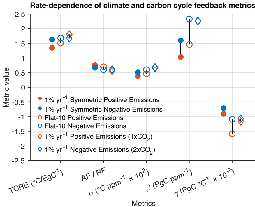
Figure 7: Rate-dependence of climate and carbon cycle feedback metrics in all simulations. Metrics shown include: the transient climate response to cumulative \text{CO}_2 emissions and removals (TCRE and TCRR), airborne fraction for positive emissions (AF) and removal fraction for negative emissions (RF), climate sensitivity parameter \alpha , concentration-carbon feedback parameter \beta and climate-carbon feedback parameter \gamma . Carbon cycle feedback parameters are quantified in units of Pg of carbon per unit ppm and Pg of carbon per unit ^{\circ}\text{C} . The carbon cycle feedbacks represent the total sensitivity of the carbon pools (land plus ocean carbon) to changes in \text{CO}_2 concentration and temperature. Vertical black lines depict the asymmetry under positive and negative emissions.
