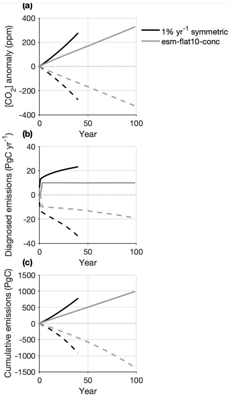
170 Figure 1: Prescribed atmospheric CO 2 concentration, b. diagnosed annual positive and negative CO 2 emissions, and c. diagnosed 175 cumulative positive and negative CO 2 emissions in the fully coupled (FULL) 1% yr -1 symmetric and esm-flat10-conc positive (PE) and negative (NE) emissions simulations. Solid lines represent the positive emissions run; dashed lines represent the negative emissions run. The rate of CO 2 concentration change in panel a. is calculated relative to the 2xCO 2 equilibrium state.
