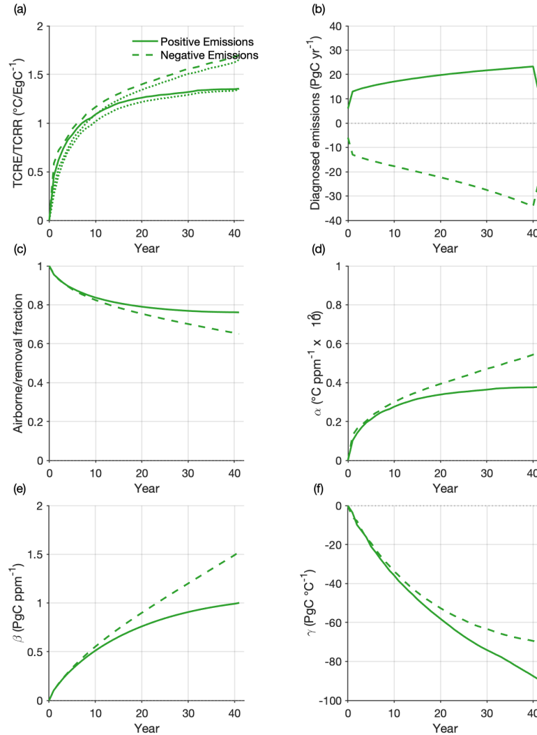
Figure 6: a. Transient climate response to cumulative CO 2 emissions and removals. Solid and dashed lines – calculated from the Jones & Friedlingstein (2020) framework for the 1% yr -1 symmetric positive (PE) and negative emissions (NE) runs respectively; dotted lines – direct calculation (ratio of global mean temperature change to cumulative emissions or removals) b. diagnosed positive or negative emissions c. airborne fraction for positive emissions; removal fraction for negative emissions d. climate sensitivity
