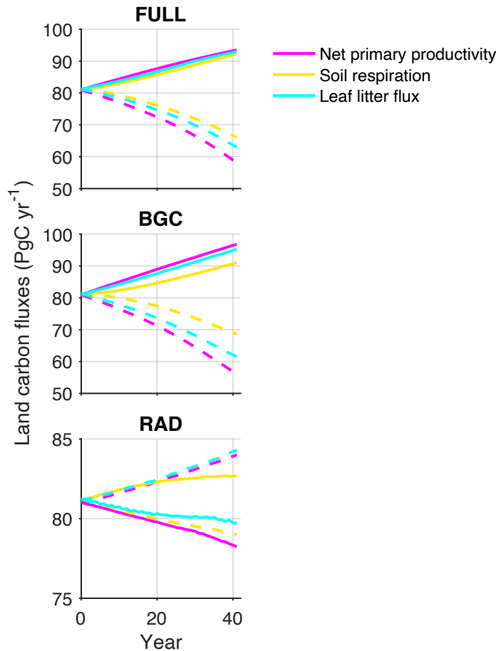
Figure 4: Land carbon fluxes for the three modes of the 1% yr -1 symmetric simulations are shown. NPP = net primary productivity, LLF = leaf litter flux and SR = soil respiration. Fully coupled (FULL); biogeochemically coupled (BGC); radiatively coupled (RAD). Solid lines represent the positive (PE) emissions run; dashed lines represent the negative emissions (NE) run. Note the difference in the vertical scale of the RAD panel (last panel).
