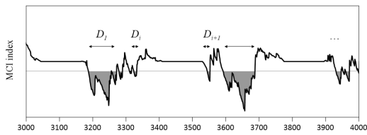
Figure 2. Schematic presentation of drought duration
