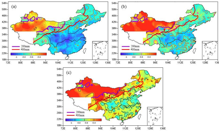
Figure 9. Distribution of parameter k of Moderate drought (a), Severe drought (b) and Extreme drought (c)
