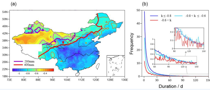
Figure 7. Distribution of parameter k (a) and the relationship between the drought duration and its frequency with different parameters(b)
