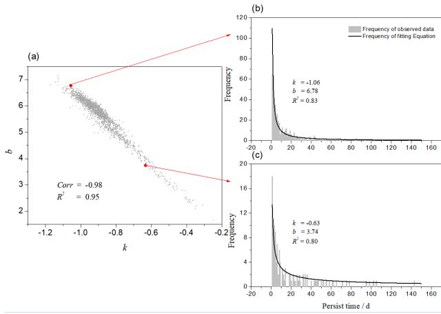
140 Figure 5. Relationship between parameter k and parameter b (a) and the relationship between the drought duration and its frequency with different parameters (b) and (c).
