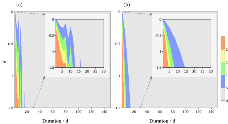
Figure 6. Relationship among the drought duration, the frequency and the parameter k based on the observed data(a) and the numerical equation(b)
