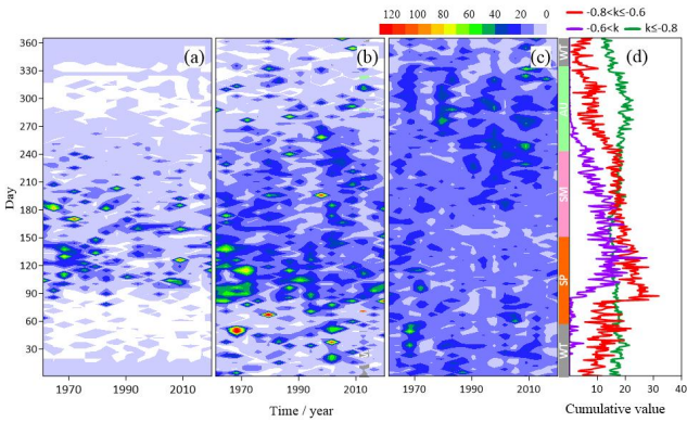
Figure 8. The relationship between the drought duration and the start moment in (a) arid region, (b) semi-arid region, (c) humid-semihumid region. (d) Distribution of drought start moments with days in different regions.
