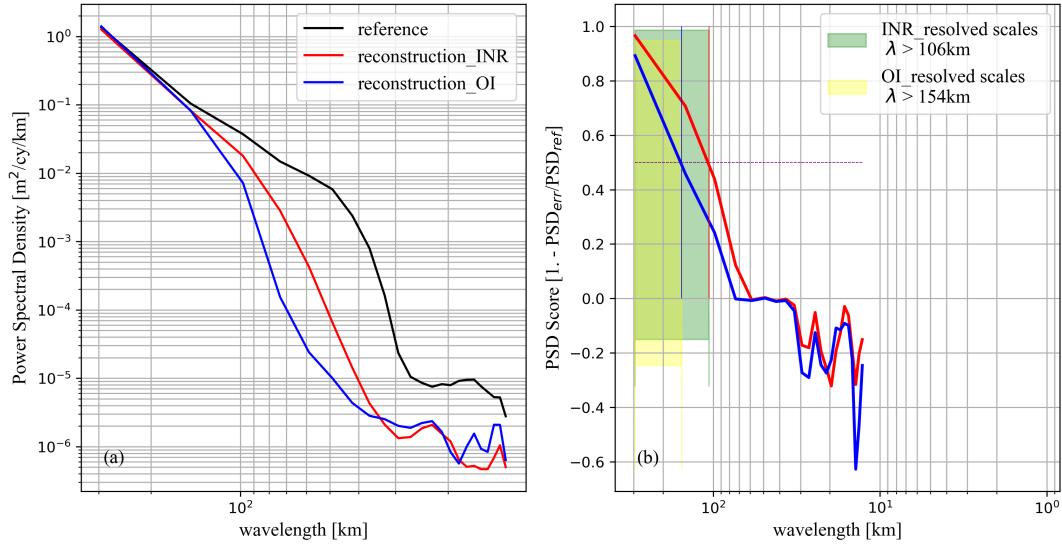
Figure 5. OSE along-track spectral diagnostics. (a) One-dimensional along-track spatial PSDs of the INR reconstruction, withheld CryoSat-2 reference SSH, and OI baseline. (b) Corresponding PSD skill score, 1 - \text{PSD}_{\text{err}}/\text{PSD}_{\text{ref}} , with the 0.5 crossing used to derive the PSD-score-based effective spatial scale. Here, \text{PSD}_{\text{err}} and \text{PSD}_{\text{ref}} are the one-dimensional spatial PSDs of the reconstruction error and CryoSat-2 reference SSH, respectively, computed from the valid CryoSat-2 along-track segments following the SSH MapMed OSE benchmark evaluation procedure (Ocean Data Challenges, 2023). Higher scores indicate smaller relative spectral errors.
