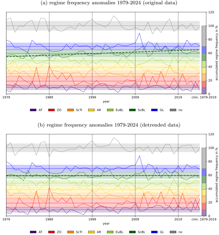
Figure 14. Anomalies of annual regime frequency (solid thin lines in %) relative to the climatological mean occurrence frequency 1979-2019. The climatological mean frequencies are shown on the right as stacked bar as well as stacked thin horizontal lines. These serve as the reference for the illustration of the anomaly. In addition, the significant linear trend for ScBL is shown as a dashed dark green line. Shading denotes \pm 1 standard deviation of annual regime frequencies 1979-2019 centred around the respective climatological mean. (a) data for the original ERA5 regime definition, and (b) for the variant using detrended Z500 (see text for details). Data shown for 1979-2024.
