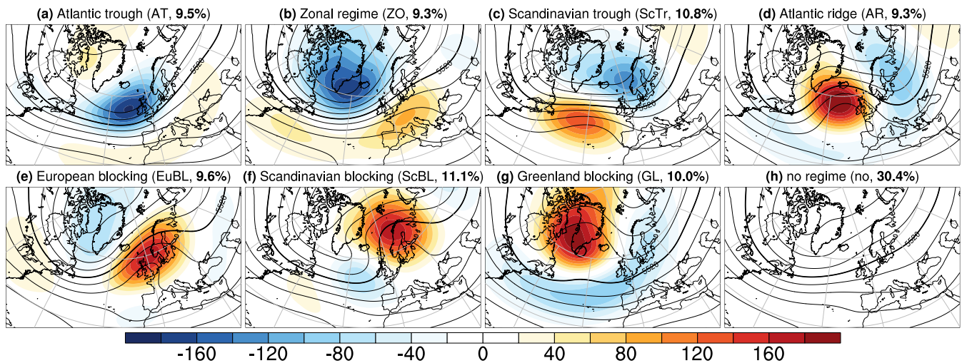
Figure 3. (a-g) Mean composites of 10-day low-pass filtered 500 hPa geopotential height anomalies ( \widehat{Z500'}^{LF}_{wr} , shaded every 20 gpm) and absolute field (black contours every 80 gpm, 5520 gpm in bold) for the seven year-round North Atlantic European weather regimes and “no regime” times (h). The composites are computed as the mean of \widehat{Z500'}^{LF} for all 3-hourly time steps 1979-2019 attributed to a regime wr according to the life cycle definition or “no regime” (see Section 3.2). Numbers in brackets indicate the annual frequency of the shown regime according to the life cycle attribution.
