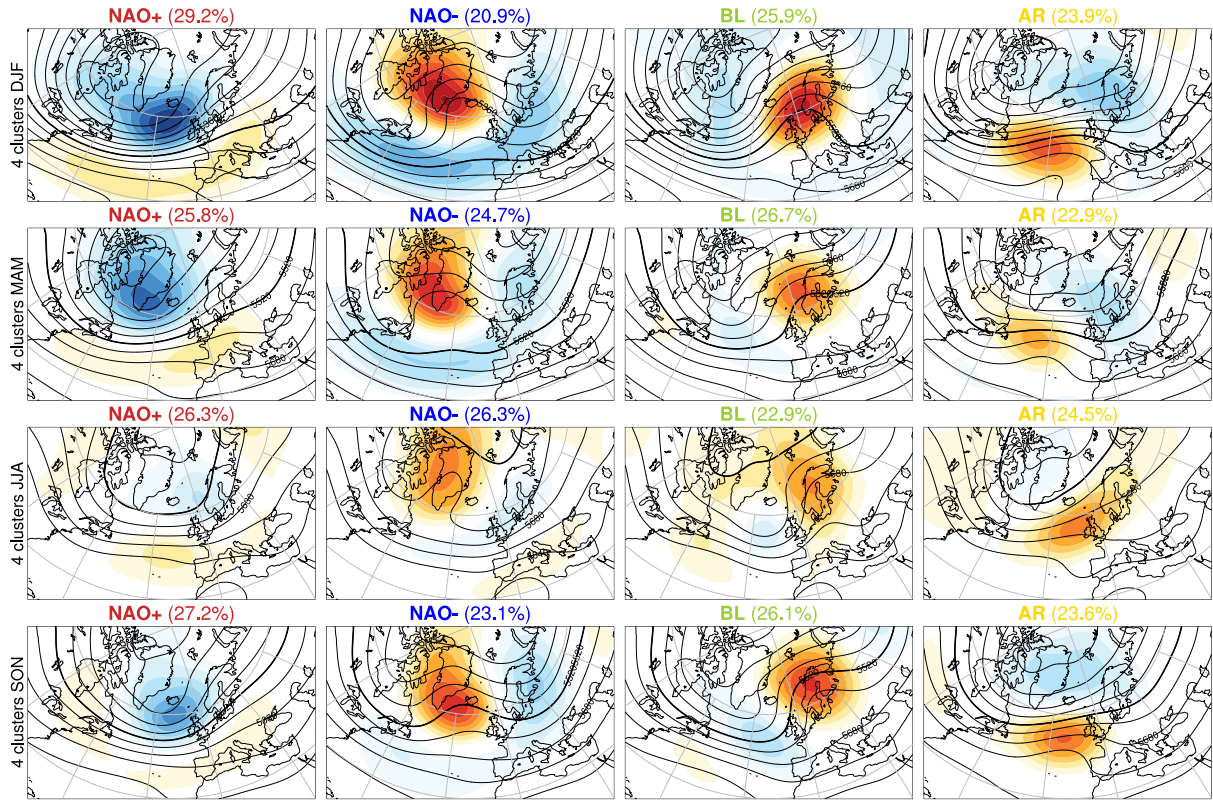
Figure 4. Mean composites of 10-day low-pass filtered 500 hPa geopotential height anomalies ( \overline{Z500'}^{LF}_{wr} , shaded every 20 gpm) and absolute field (black contours every 80 gpm, 5520 gpm in bold) for variants with 4 seasonal North Atlantic European weather regimes and EOF-clustering applied to non-normalised 10-day low-pass filtered 500 hPa geopotential height anomalies ( \widehat{Z500'}^{LF} ) shown for each season. The composites are computed as the mean of \widehat{Z500'}^{LF} for all 6-hourly time steps 1979-2019 attributed to a regime wr according to their contribution to the EOF-clusters without applying the life cycle definition (see Section A2). Labels indicate the regime name abbreviation: NAO+ regime (NAO+), NAO- regime (NAO-), Blocking regime (BL), Atlantic Ridge regime (AR). Numbers in brackets indicate the seasonal frequency of the respective EOF cluster.
