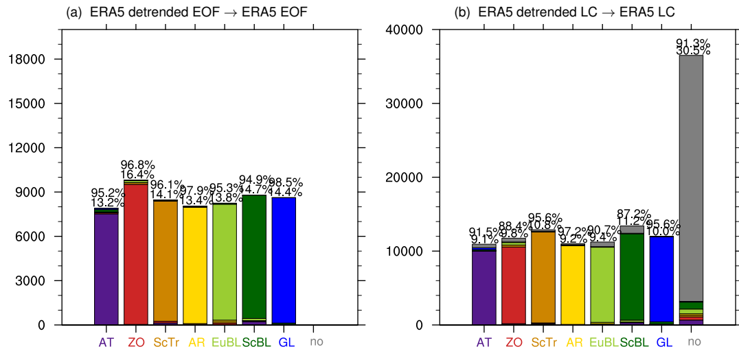
Figure C7. As in Figure 5 frequency of the 7 regimes according to the raw EOF-cluster attribution and (b) frequency of the 7+1 weather regimes including the no regime class according to the life cycle attribution. Each bar shows the number of time steps (6-hourly in (a) for EOF attribution and 3-hourly in (b) for life cycle attribution) for the definition using detrended data on the x-axis. The lower numbers on top of each bar indicate the relative frequency of the regime. Coloured bar segments indicate to which regime these time steps are attributed in the original ERA5 definition using non-detrended data and the fraction of times sharing the same regime with the original ERA5 definition is indicated by the upper number. The data period covers 1979-2019.
