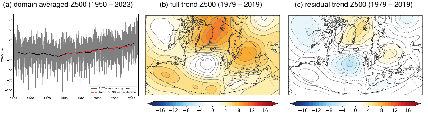
Figure 13. Trends in 10-day low-pass filtered 500 hPa geopotential height anomalies (units are \text{gpm (10yr)}^{-1} ). (a) Time series of spatial average in the EOF domain ( 80^\circ\text{W} - 40^\circ\text{E} , 30^\circ\text{N} - 90^\circ\text{N} ) for 24-hourly time steps from 11 January 1950 until 31 December 2023 (grey) and 5-year running mean (black bold), as well as linear trend (red dashed) in the period 1 January 1979 – 31 December 2019. (b) Grid point based full trend (shaded every 1 \text{ gpm (10yr)}^{-1} ) during the period 1 January 1979 – 31 December 2019. (c) Residual trend (shaded every 1 \text{ gpm (10yr)}^{-1} ) computed by subtracting the area-averaged trend from (a) of 5.398 \text{ gpm (10yr)}^{-1} from the full trend in (b).
