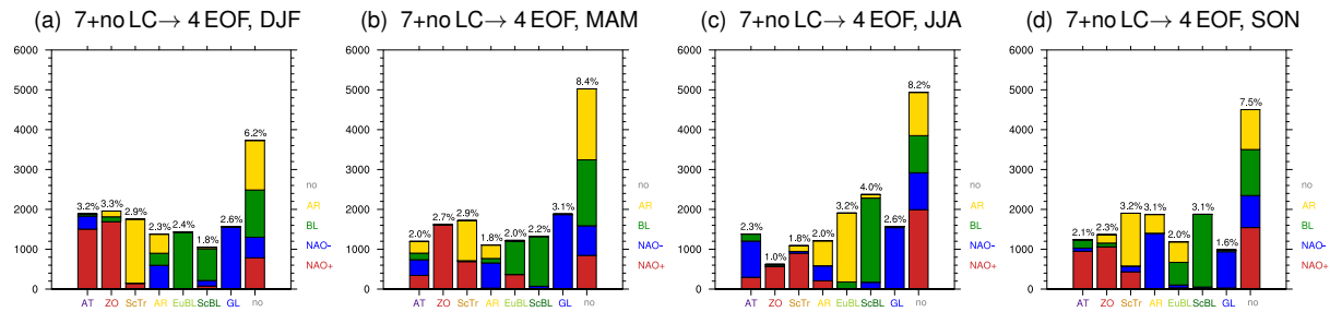
Figure C1. As Figure 5 but vice-versa frequency of the year-round 7+1 regimes in each season and coloured bar segments indicate how these time steps correspond to the 4 seasonal regimes based on non-normalized data (1979-2019) for different seasons. Labels on x-axis indicate the regime name and colour code for the 7+1 regimes, labels to the right of each sub-figure indicate the name and colour-code for the 4 seasonal regimes.
