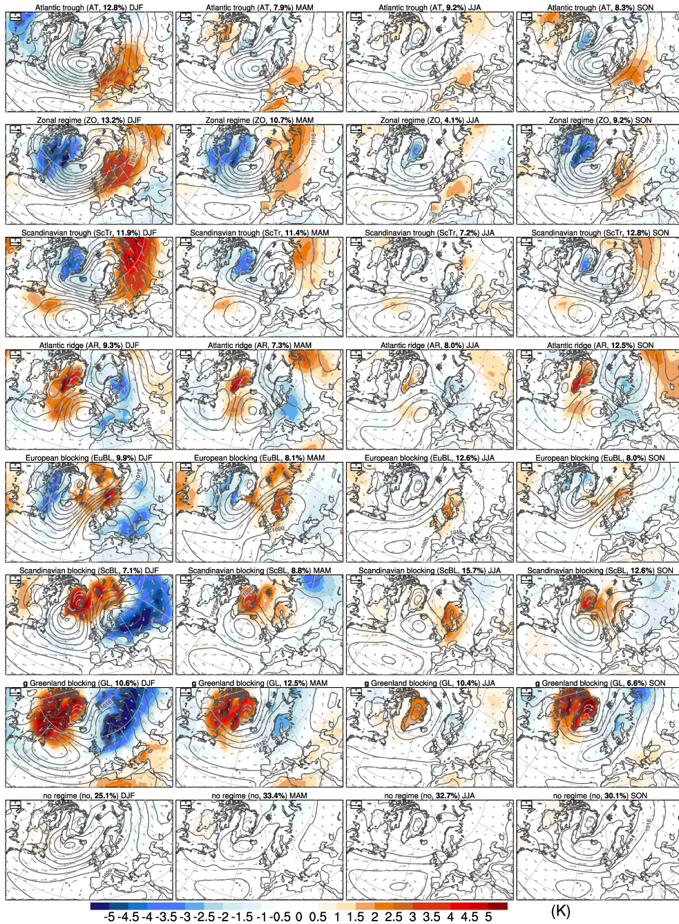
Figure 8. Composites of mean 2 m temperature anomalies (shaded every 0.5 K) during each of the regimes (rows) stratified according to season (columns). Anomalies are computed with respect to a 90-day running mean climatology and averaged for all days attributed to one of the seven or “no regime” in the respective three-months season (see Section 2). Contours show composite mean sea level pressure (every 4 hPa) and vectors 100 m wind with a reference arrow whose length corresponds to 8 \text{ m s}^{-1} wind speed to the top left. The regime name, abbreviation, seasonal regime frequency, and season are indicated in each panel caption.
