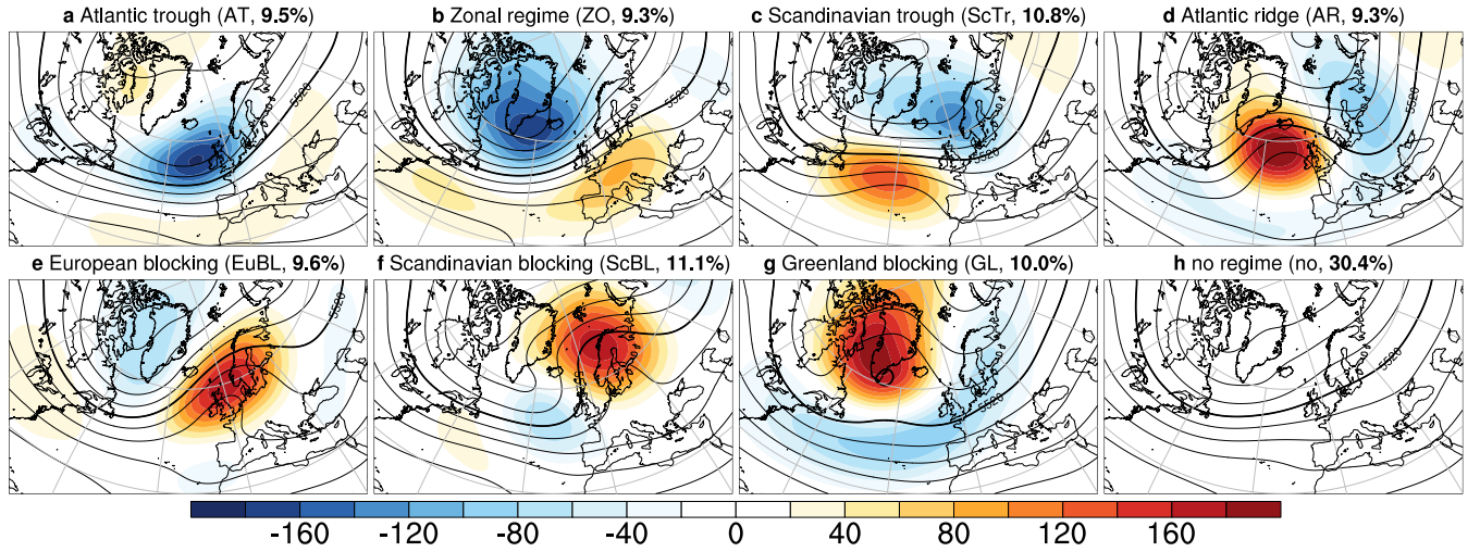
Figure 3. (a-g) Mean composites of 10-day low-pass filtered 500 hPa geopotential height anomalies ( \widehat{Z500'}^{LF}_{wr} , shaded every 20 gpm) and absolute field (black contours every 80 gpm, 5520 gpm in bold) for the seven year-round North Atlantic European weather regimes and “no regime” times (h). The composites are computed as the mean of \widehat{Z500'}^{LF} for all 3-hourly time steps 1979-2019 attributed to a regime wr according to the life cycle definition or “no regime” (see Section 3.2). Numbers in brackets indicate the annual frequency of the shown regime according to the life cycle attribution.
