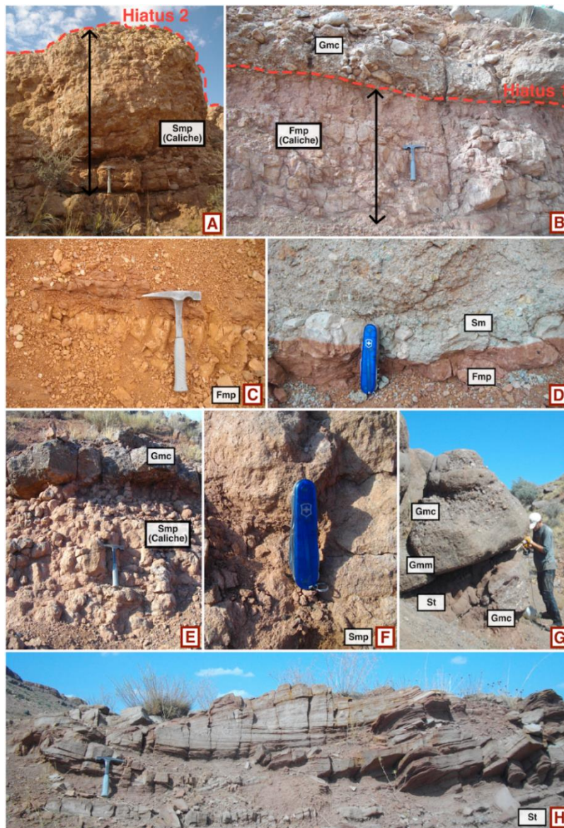
Figure 3: Examples of sedimentary facies described in Table 1. (A) Well-developed caliche (facies Smp); Hiatus 2, marked by red dotted lines, corresponds to the stratigraphic level at 292 m; hammer for scale. (B) Well-developed caliche (facies Fmp), eroded at the top by channelized conglomerates (facies Gmc); this surface corresponds to Hiatus 1 at 263 m; hammer for scale. (C) Massive clayish red beds (facies Fmp); hammer for scale. (D) Massive greenish sandstones containing gravel-sized clasts up to 2 cm (facies Sm), overlying red beds (facies Fmp); knife for scale. (E) Clast-supported conglomerates overlying caliche developed in sandstones (facies Smp); hammer for scale. (F) Massive sandstone with diffuse carbonate development (facies Smp); knife for scale. (G) Alternation of matrix-supported (facies Gmm) clast-supported conglomerates (facies Gmc) and the channelized sandstones (facies St); Leny Montheil (180 cm) for scale. (H) Trough cross-bedded sandstones (facies St); hammer for scale.
