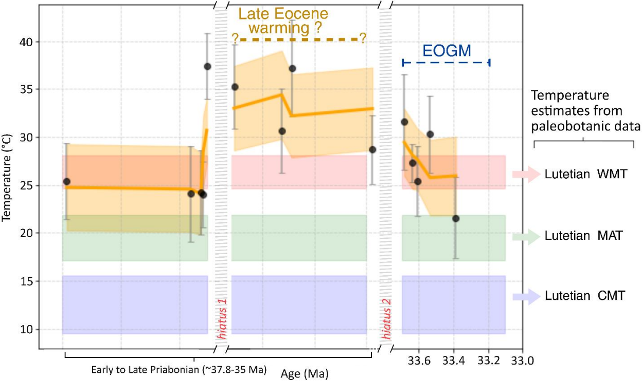
608 609 Figure 8: Clumped isotope ( \Delta_{47} ) paleotemperatures from pedogenic carbonates in the Büyükteflek section (Çiçekdagi Basin, 610 Turkey), spanning the Early to Late Priabonian (~37.8–35 Ma) to the Early Rupelian (~33.4 Ma). The orange line shows the moving 611 average; error bars = 1 standard error (SE). Temperature estimates for the Lutetian (48–41 Ma), derived from paleobotanical data 612 reported by Raynaud et al. (2025). (WMT: Warm Month Temperatures; MAT = Mean Annual Temperatures; CMT = Cold Month 613 Temperatures).
