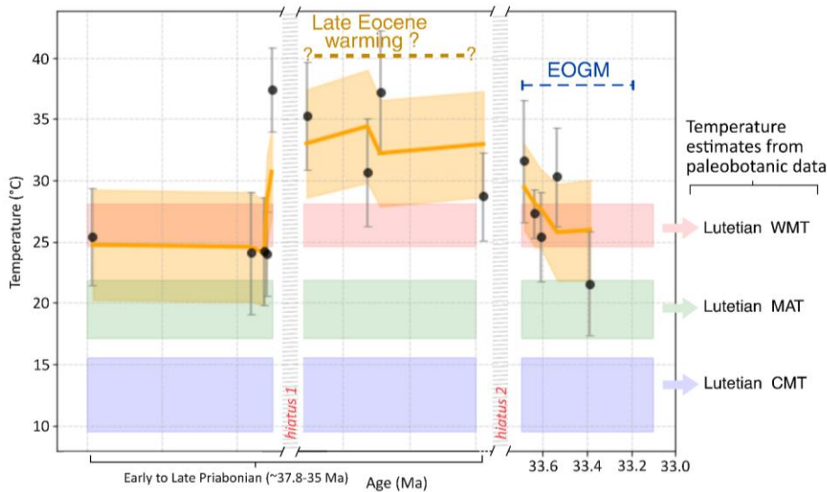
Figure 8: Clumped isotope ( \Delta_{47} ) paleotemperatures from pedogenic carbonates in the Büyükteflek section (Çiçekdağı Basin, Turkey), spanning the Early to Late-Middle Priabonian (~37.8–35.6 Ma) to the Early Rupelian (~33.4 Ma). The orange line shows the moving average; error bars = 1 standard error (SE). Temperature estimates for the Lutetian (48–41 Ma), derived from paleobotanical data reported by Raynaud et al. (2025). (WMT: Warm Month Temperatures; MAT = Mean Annual Temperatures; CMT = Cold Month Temperatures).
