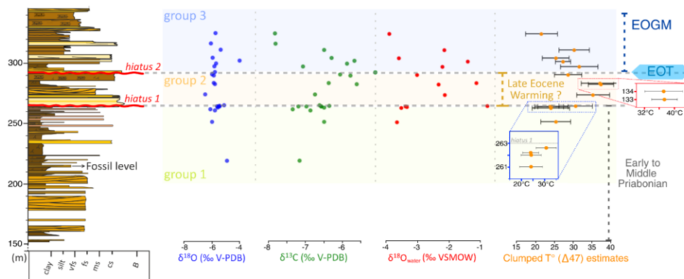
Figure 6: Scaled stratigraphic log highlighting the pedogenic carbonate sampling interval. From left to right are plotted \delta^{18}\text{O} , \delta^{13}\text{C} , \delta^{18}\text{O}_{\text{waters}} , and \Delta 47 ( \pm 1\text{se} ) values from pedogenic carbonates. Coloured fields (light green, light orange, light blue) indicate distinct groups, interpreted as reflecting differences separated by the hiatuses. Horizontal grey dotted lines delineate the hiatus 1 and hiatus 2.
