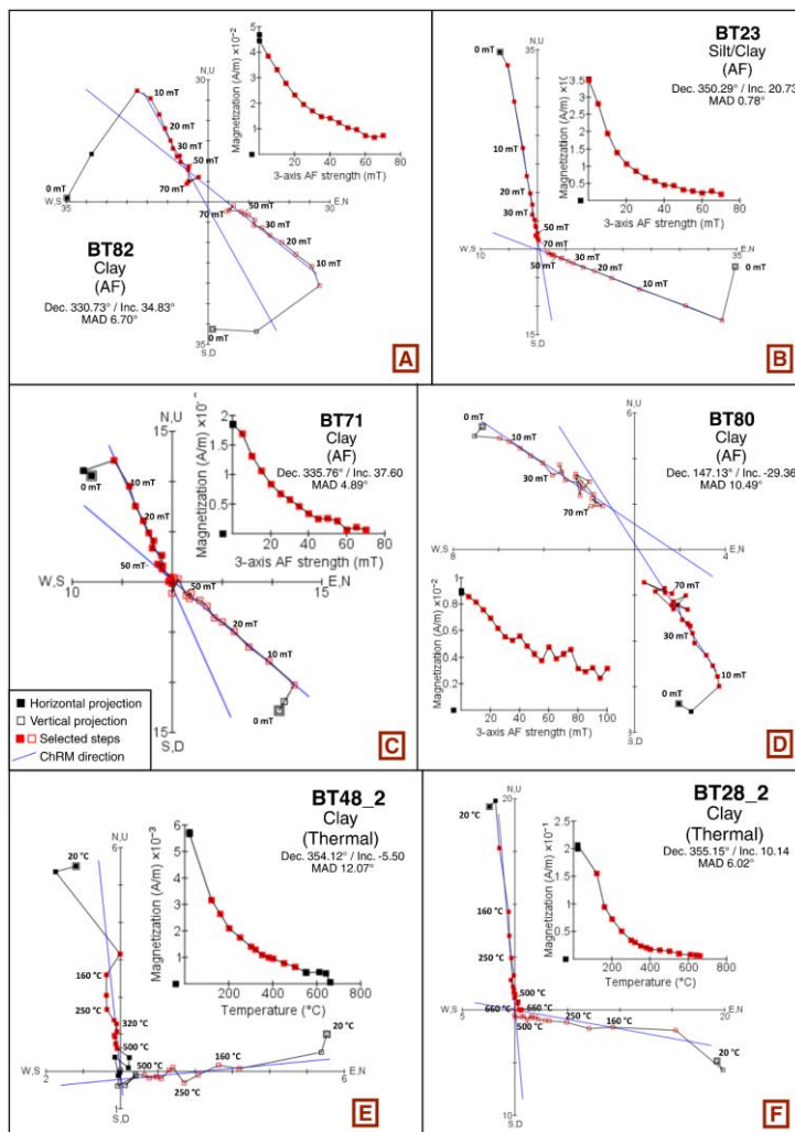
Figure 5: Representative intensity plots and Zijderveld-orthogonal demagnetization diagrams obtained after Alternating Field (AF) and Thermal demagnetization.
