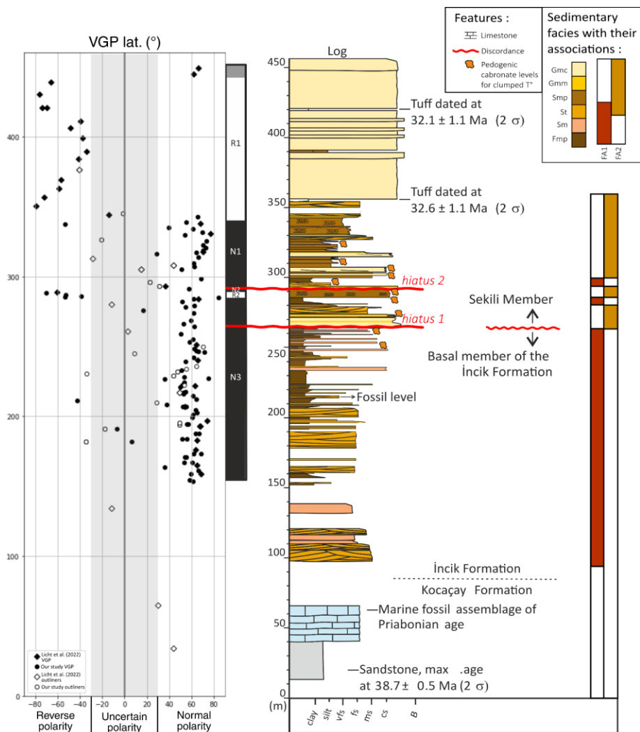
Colour coding illustrates the different facies and facies associations. The VGP latitude diagram shows the paleomagnetic data and the corresponding magnetozones (R1, N1, N2, R2, N3, N4).
