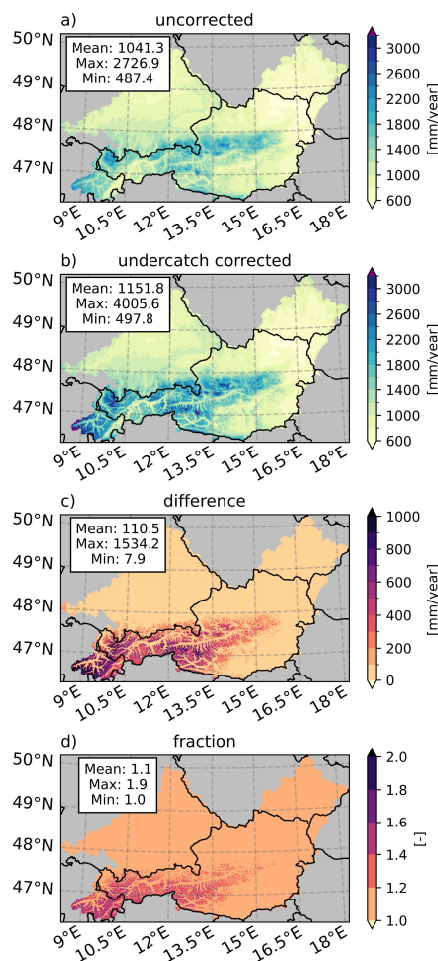
Figure 8. Precipitation climatologies (1991-2020) of a) uncorrected b) undercatch corrected and precipitation amounts. Panel c) shows their absolute difference and d) their fraction. The first three panels are given in mm/year, the last is dimensionless. The mean, maximum and minimum values per panel are given in the text boxes.
