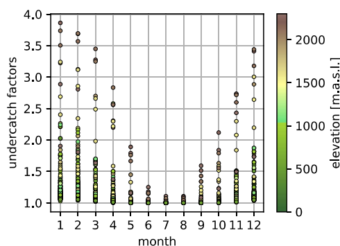
Figure 5. Station-derived monthly undercatch factors. The color-coding refers to the station elevation of the data entries in [m.a.s.l.], where green colors show stations with low and brown and yellow colors stations with high elevation.
