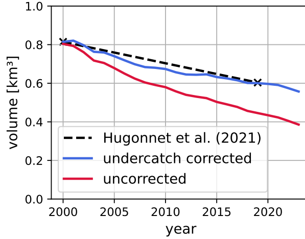
Figure 14. Simulated total glacier volume change for glaciers with a surface area above 1 km 2 in the Schlegeis study region in km 3 from 2000-2023. The undercatch corrected (blue) and uncorrected (red) Alpine3D simulation is compared to the average volume change of the selected glaciers between 2000-2019 as published by Hugonnet et al. (2021), which amounts to a loss of -0.011 km 3 /year between 2000 and 2019.
