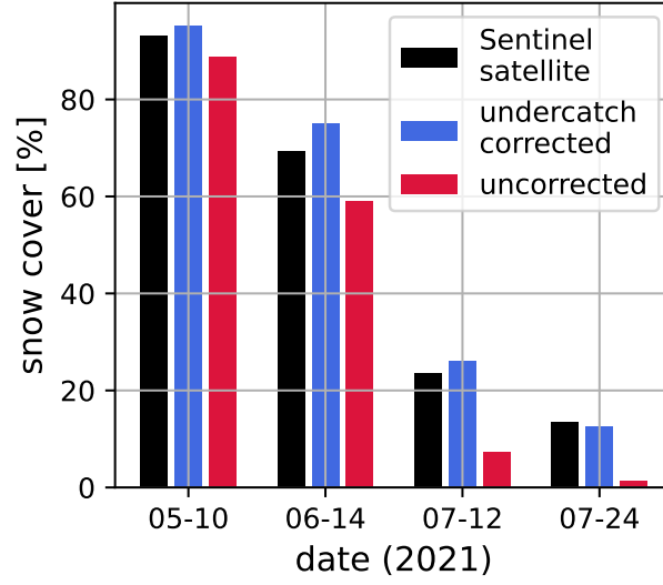
Figure 13. Comparison of SCA (%) in the Kölnbrein catchment derived from Sentinel-2 satellite observations and Alpine3D simulations for different dates in the snow-melting period 2021. Compared are Sentinel satellite observations (black), undercatch corrected simulations (blue) and uncorrected simulations (red).
