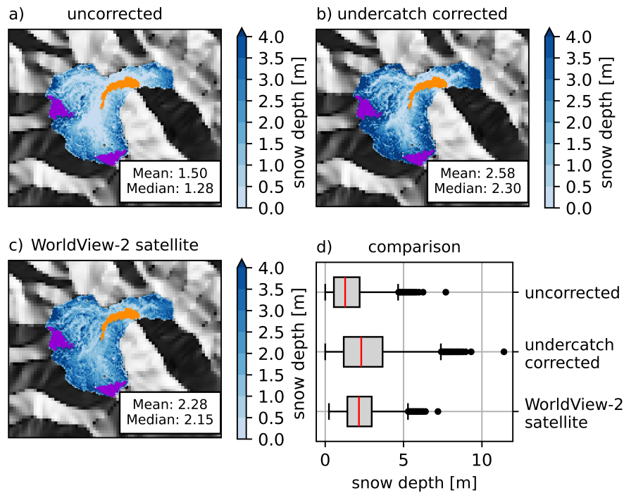
Figure 12. Comparison of satellite-derived and modeled snow depths on May 10 th 2021 in the Kölnbrein study region. Displayed is the snow depth in m from Alpine3D modeling results using a) uncorrected precipitation and b) undercatch corrected input data and c) derived from the WorldView-2 stereo satellite image. Spatial mean and median are given in the text boxes. Shaded reliefs are used as background. The violet (orange) area shows the grid cells covered by glaciers (the reservoir). Panel d) shows a comparison of the spatial variability. The whiskers correspond to the 5 th and 95 th percentile. Outliers are displayed as dots.
