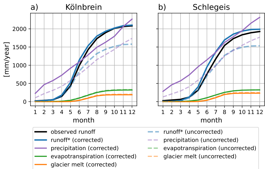
Figure 11. COSERO runoff simulation results, as well as observed runoff, displayed as the cumulative water balance for the high-alpine study regions a) Kölnbrein and b) Schlegeis. Solid lines refer to the simulation results using undercatch corrected data, while dashed lines refer to results using uncorrected precipitation input. *The runoff is only considered for timesteps with valid runoff observations.
