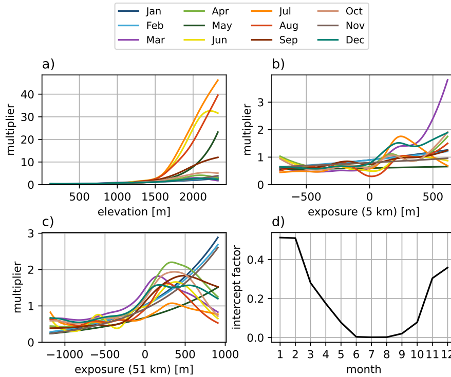
Figure 6. GAM smooth functions, color-coded for every month. Panel a)-c) show the back-transformed multiplier to the undercatch factors, dependent on the three selected geographical features elevation, exposure (5 km) and exposure (51 km). Panel d) shows the constant intercept, which varies per month.
