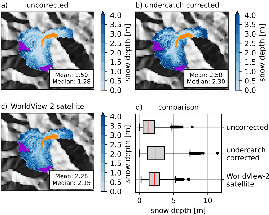
Figure 12. Comparison of satellite-derived and modeled snow depths on May 10 th 2021 in the Kölnbrein study region. Displayed is the snow depth in m from Alpine3D modeling results using a) uncorrected precipitation and b) undercatch corrected input data and c) derived from the WorldView-2 stereo satellite image. Spatial mean and median are given in the text boxes. Shaded reliefs are used as background. The violet (orange) area shows the grid cells covered by glaciers (the reservoir). Panel d) shows a comparison of the spatial variability. The whiskers correspond to the 5 th and 95 th percentile. Outliers are displayed as dots.
