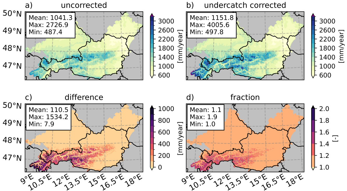
Figure 8. Precipitation climatologies (1991-2020) of a) uncorrected b) undercatch corrected and precipitation amounts. Panel c) shows their absolute difference and d) their fraction. The first three panels are given in mm/year, the last is dimensionless. The mean, maximum and minimum values per panel are given in the text boxes.
