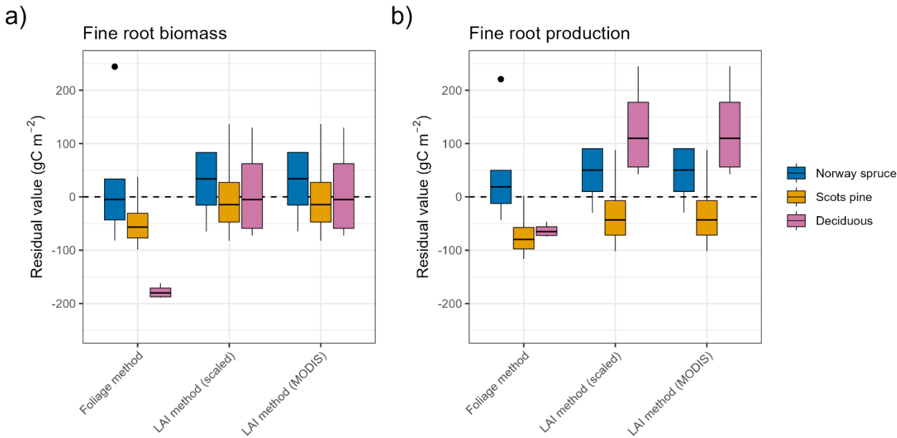
Figure 2: Residuals for fine root biomass (a) and fine root production (b) across tree species and methods for estimating foliage biomass and related fine root biomass and production. For each species, five foliage-to-fine-root biomass ratios were assumed (Table 1). The foliage-based method used allometric foliage biomass, while the two LAI-based methods estimate foliage biomass from LAU and specific leaf area. LAI data were obtained from MODIS (MODIS LAI) or from optically scaled SR16 values (SR16 LAI). Each boxplot shows the interquartile range (Q1–Q3), with whiskers extending to the smallest and largest values within 1.5 \times \text{IQR} from Q1 and Q3.
