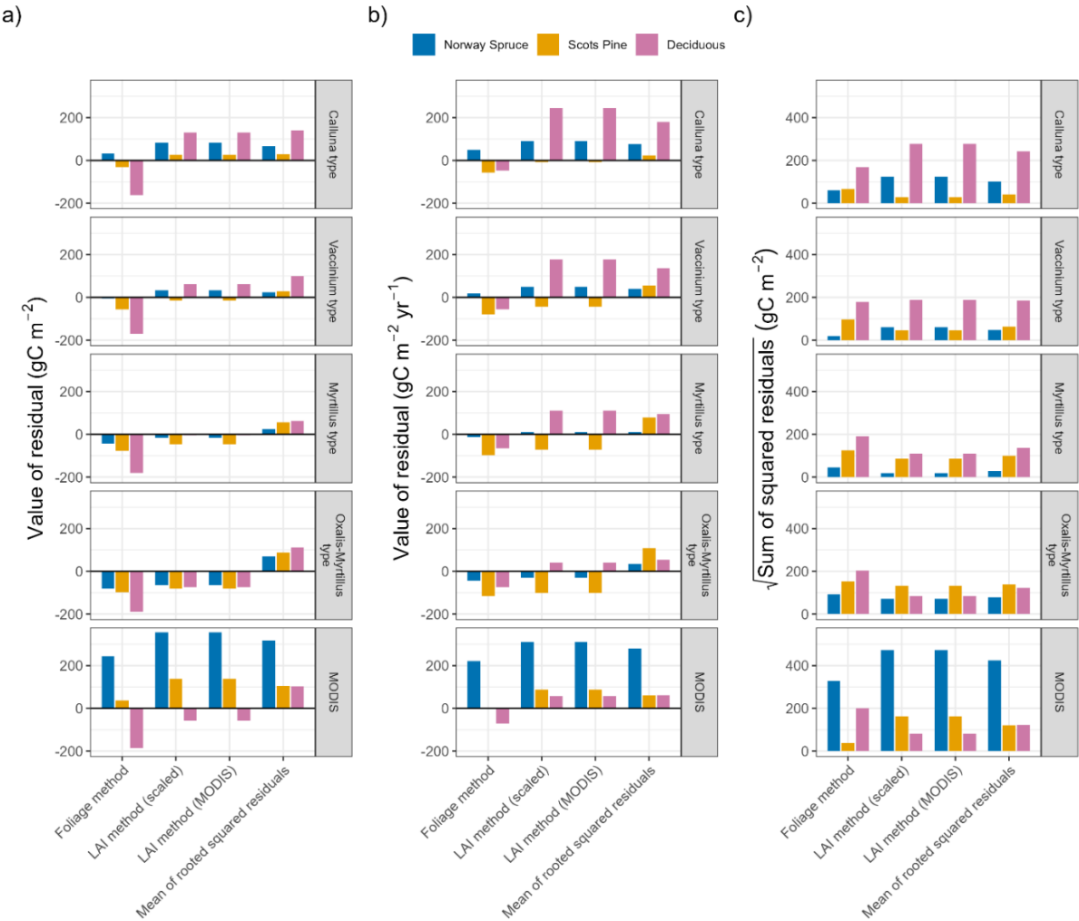
280 Figure 1: Residuals for estimated fine root biomass (a) and production (b), and the combined residuals of biomass and production (c) in Norwegian forests dominated by Norway spruce, Scots pine, or deciduous trees (primarily Betula spp.). Residual are calculated based on the difference between fine root estimates in the meta-analysis by Yuan and Chen (2010) and our values of fine root biomass and production, derived from three different methods for estimating foliage biomass and related fine root biomass and production. The vegetation types represent a gradient from dry, nutrient-poor sites ( Calluna type) to moist, nutrient-rich sites ( Oxalis-Myrtillus type).
