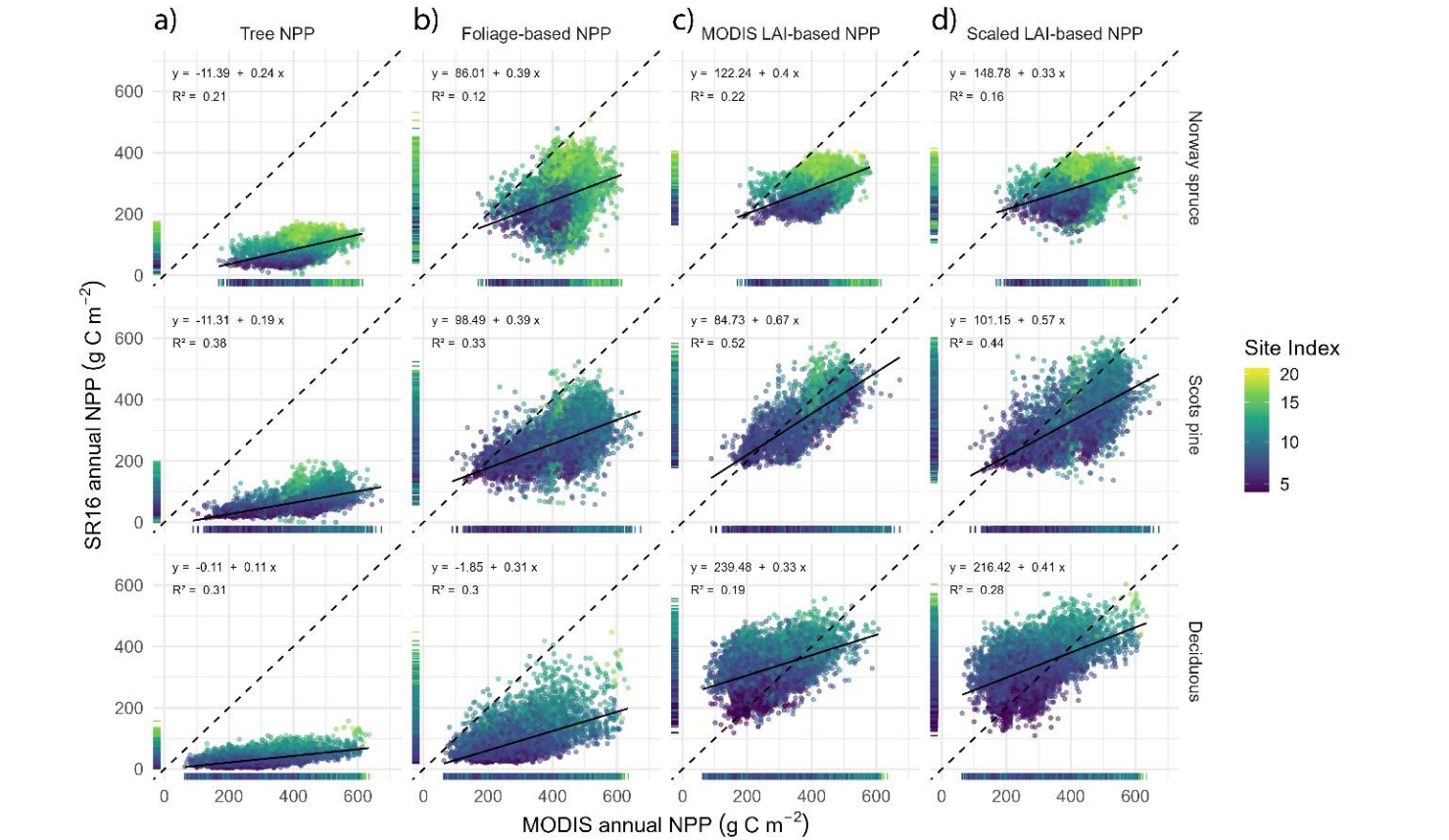
Figure 3: Relationships between tree NPP (column a) and total NPP (columns b–d) derived from different methods for estimating foliage biomass, and associated fine root biomass and production, compared with MODIS Euro NPP, for forests dominated by Norway spruce, Scots pine, or deciduous trees (primarily Betula spp.). All values are based on species-specific foliage-to-fine-root biomass ratios. The foliage-based method uses allometric estimates of foliage biomass, while the two LAI-based methods derive biomass from LAI and specific leaf area. Column (c) incorporates LAI from MODIS, and column (d) uses LAI from the Norwegian forest resources map, SR16, scaled using quantile mapping to match MODIS optical LAI. The colour gradient represents site index (a proxy for site fertility). Vertical and horizontal bars along the axes show the distribution of site index values. All site index values are log10-transformed.
