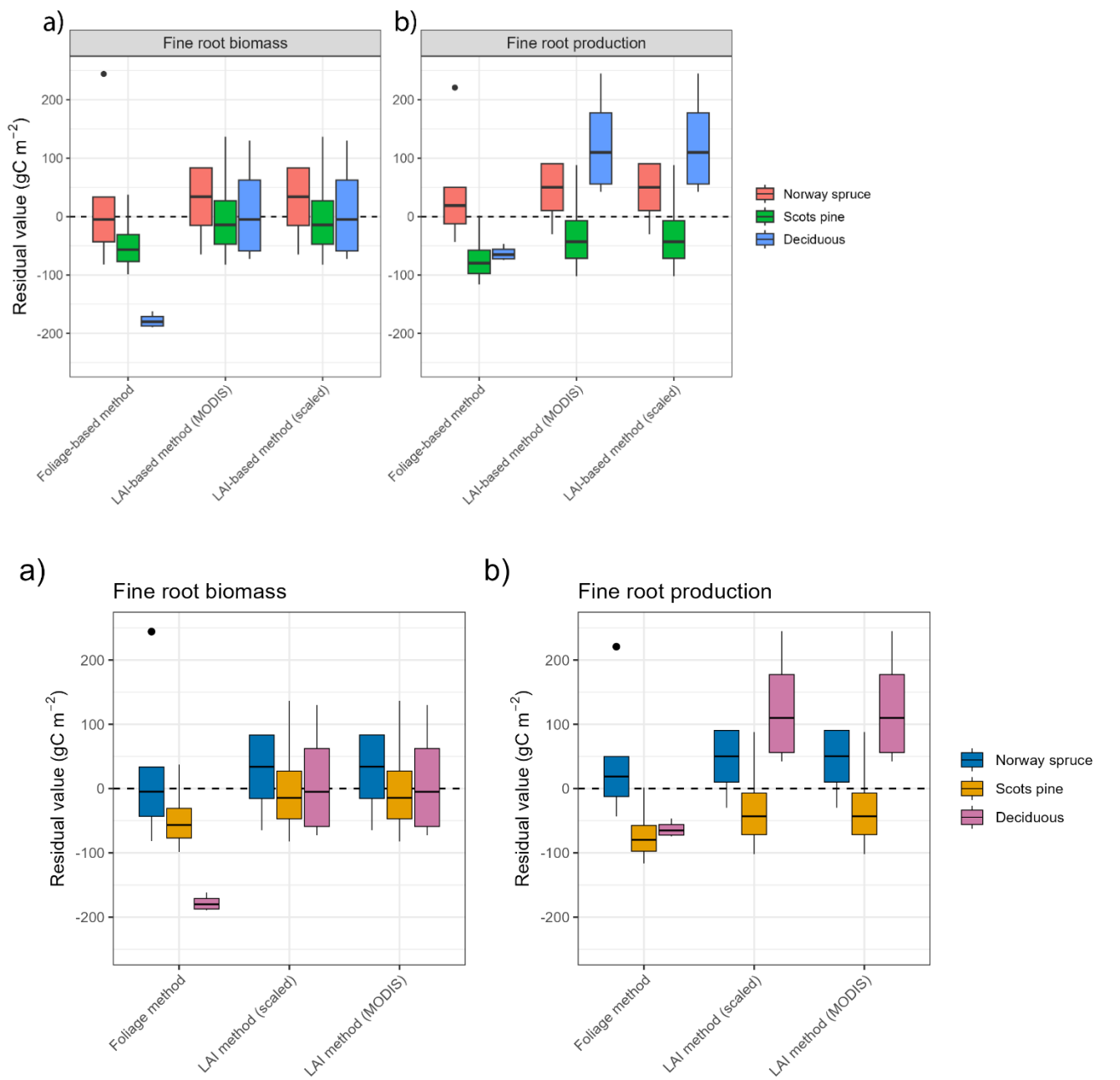
Figure 2: Residuals for fine root biomass (a) and fine root production (b) across tree species and methods for estimating foliage biomass and related fine root biomass and production. For each species, five foliage-to-fine-root biomass ratios were assumed (Table 1). The foliage-based method used allometric foliage biomass, while the two LAI-based methods estimate foliage biomass from LAU
