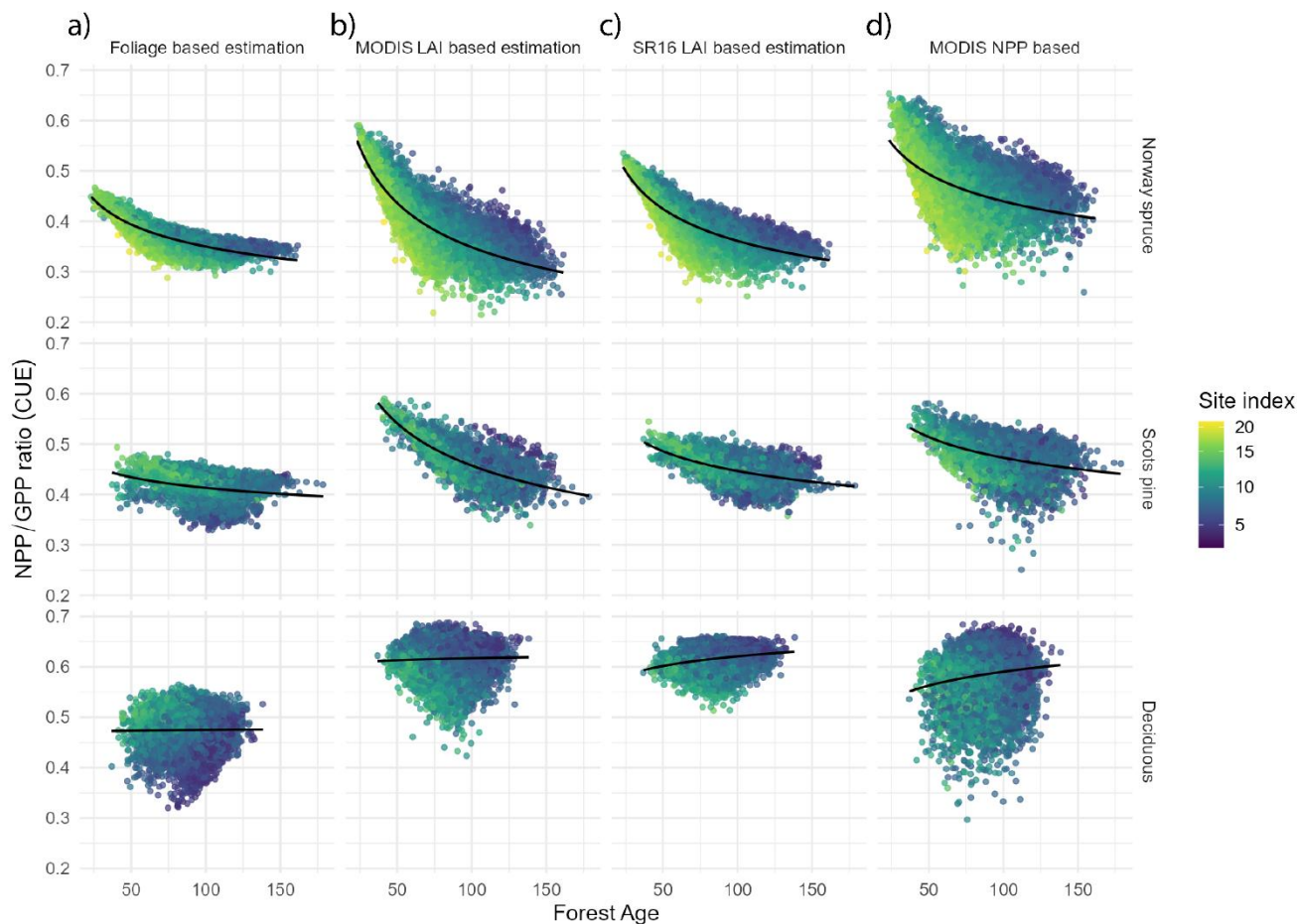
Figure 65: Relationships between the ratio of net primary production (NPP) to gross primary production (GPP) and forest age in Norwegian forest areas dominated by Norway spruce, Scots pine, or deciduous trees (primarily Betula spp.). The NPP/GPP ratio reflects carbon use efficiency (CUE) of the forest, indicating the proportion of C fixed by photosynthesis that is converted into biomass. Panels (a-c) show CUE derived from SR16 NPP, using three fine root estimation methods (foliage-based, MODIS LAI-based, and SR16 LAI-based). Panels (b) uses LAI data from MODIS, while panels (c) uses LAI data from the Norwegian Forest Resources Map SR16 scaled to optical LAI. Column (d) shows MODIS NPP-based CUE estimation, whereas SR16 data is used for biomass estimation in all GPP calculations for ecosystem respiration. Solid lines represent a power-law function fitted to the data, showing CUE development with forest age. Point colours reflect site index (fertility), with site index values log 10 -transformed.
