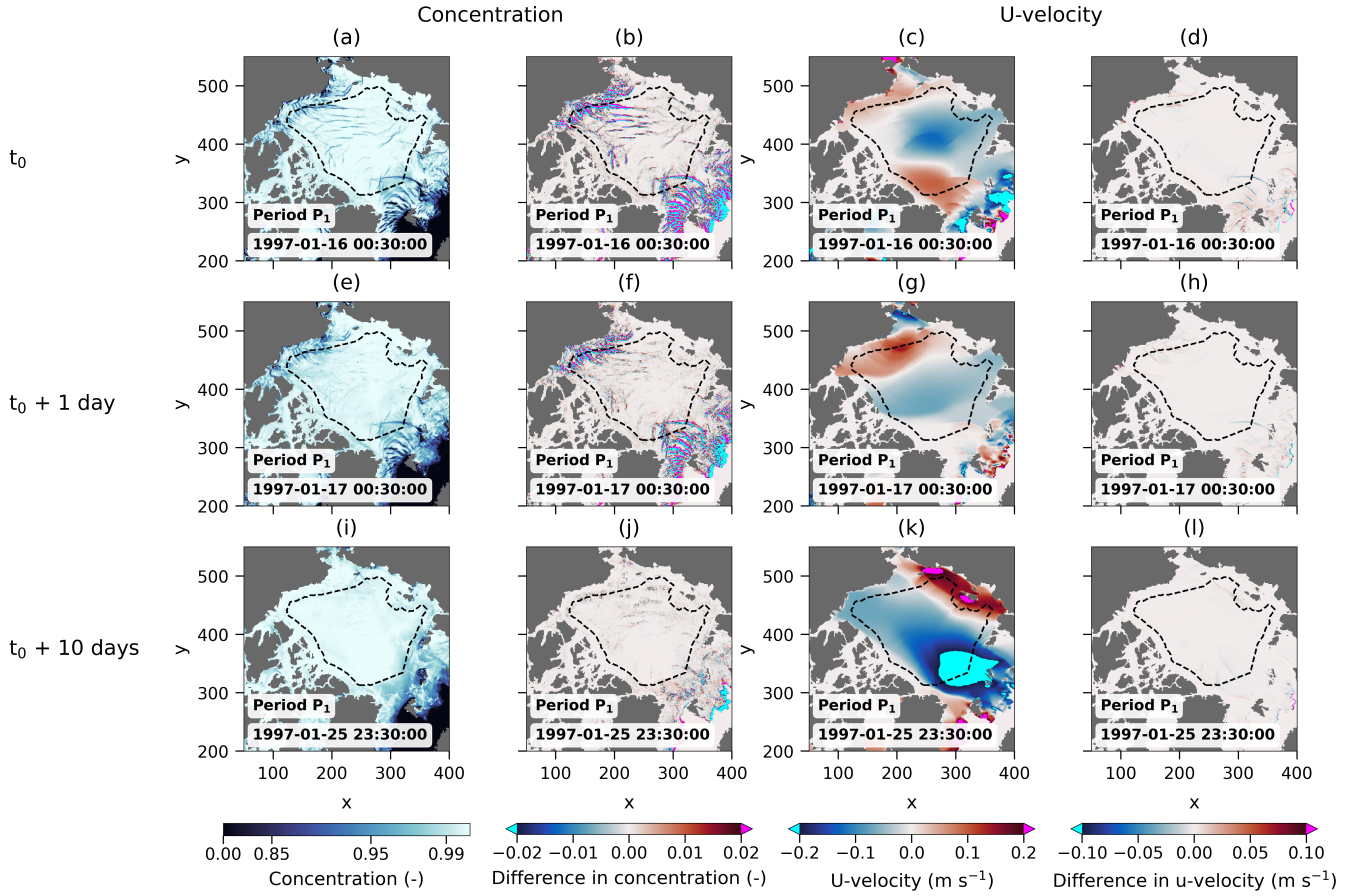
Figure 12. Same as Fig. 10 but from the aEVP forecasts initialized with the 10-km perturbation.
