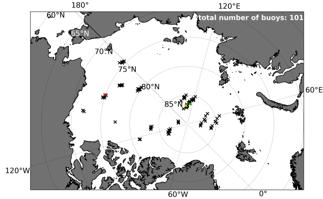
Figure 3. Location of the observed IABP buoys at initial time of the P_1, \dots, P_8 forecast periods (start dates from the 16th of January to the 27th of March 1997, see Table 1). 101 IABP buoys are considered in total. The colored "x" markers highlight the initial position of the few buoys taken as examples in the following (Figs. 5 and 14).
