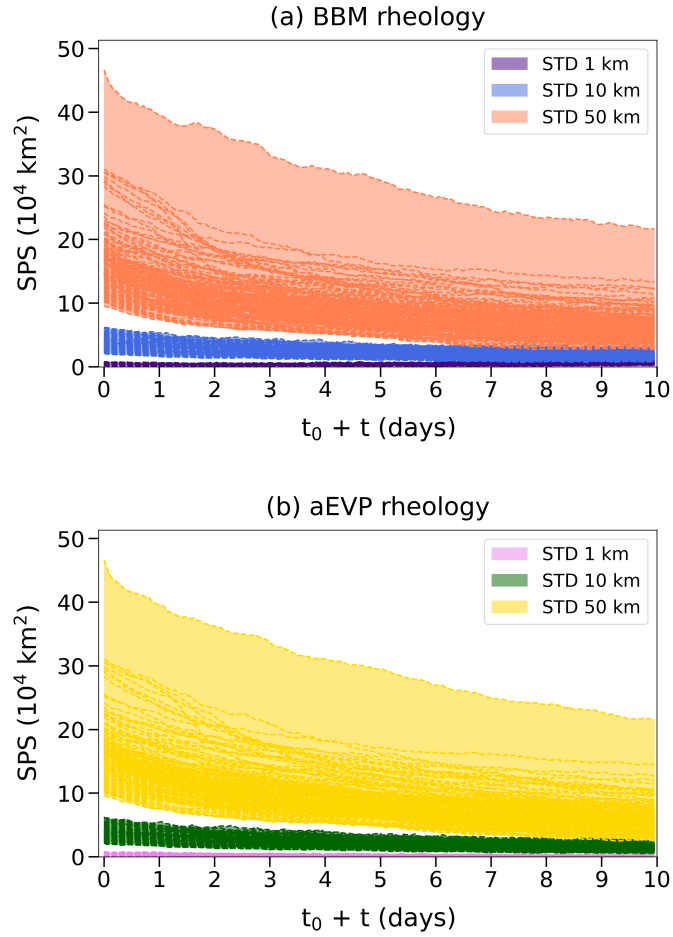
Figure 8. Temporal evolution of the SPS score computed over the whole Arctic, for BBM and aEVP forecasts (a,b resp.). The plotted curves correspond to the SPS scores computed for each of the eight forecast periods, and for each ensemble member taken alternatively as the pseudo-truth, resulting in total in 8 \text{ Periods} \times 20 \text{ scores} = 160 curves. The colors correspond to the three different amplitudes of initial perturbation.
