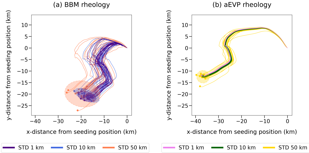
Figure 14. Example of virtual buoy trajectories simulated from the BBM and aEVP ensemble forecasts (a,b, respectively) initialized from a seeding on 7th March 1997 at midnight at -154.552^\circ E and 74.886^\circ N (red cross in Fig. 3). The colored circles highlight the final positions after 10 days and the shaded ellipses represent the 95% confidence regions of the final positions, assuming a bivariate normal distribution. The colors correspond to the rheology and amplitude of the initial perturbation of the experiments.
