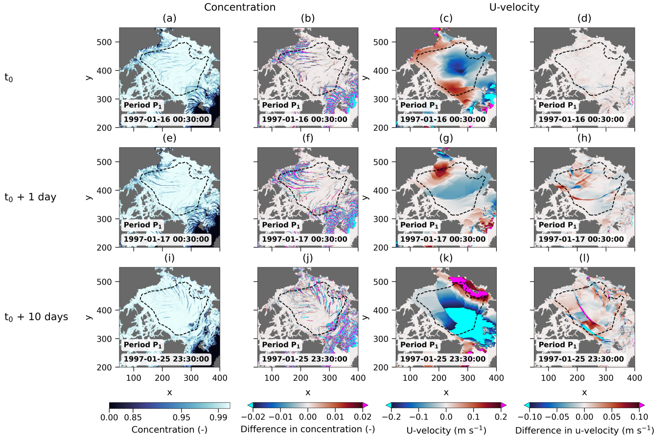
Figure 10. Sea-ice concentration and U-component of sea-ice velocity (a,e,i and c,g,k, resp.) from the BBM forecasts initialized with the 10-km perturbation at three lead times during period P_1 : (a–d) initial time, (e–h) after one day, and (i–l) after ten days. Panels (b,f,j) and (d,h,l) show, respectively, the differences in concentration and in the U-component of velocity between two perturbed ensemble members. The black dashed line defines the boundaries of the region over which the CRPS metric is computed. Axes indicate grid point indices on the model’s native grid.
