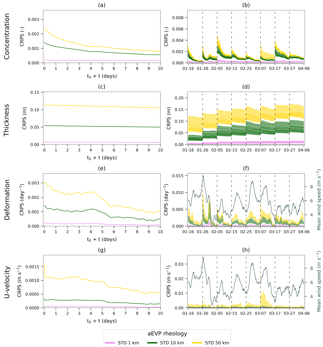
Figure 11. Same as Fig. 9 but for the CRPS metric from the aEVP forecasts.
