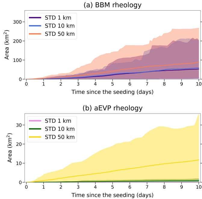
Figure 15. Temporal evolution of the spread of the virtual buoys from the BBM and aEVP ensemble forecasts (a,b, resp.), as measured by the area of the ellipse defined by the 95% confidence contour of the distribution (assumed to be bivariate normal). The colors correspond to the rheology and amplitude of the initial perturbation of the experiment. The thick lines show the ensemble mean of all the buoys over all the eight 10-day periods, while the shaded envelopes indicate the 5%-to-95% percentile ensemble distribution. Panel (a) uses a y-axis range 10 times larger (area in \text{km}^2 ) than panel (b).
