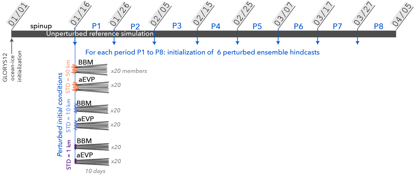
Figure 1. Summary of the experimental design, representing the unperturbed reference simulation from which are initialized, every 10 days, the 20-member ensemble forecasts with perturbed ensemble conditions for both rheologies (BBM and aEVP) and three different magnitudes of the initial perturbation each.
