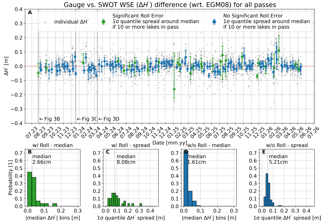
Figure 6. A: \Delta H' (SWOT vs. gauges) over time for all passes and all lakes in Denmark. For timestamps with \geq 10 observed lakes, the median and 1\sigma quantile spread (0.1585 to 0.8415) are shown. If \Delta H' significantly correlates with distance to SWOT's ground track ( d ), it is shown in green, otherwise in blue. The three vertical lines indicate the timestamps with detailed correlation plots in Figure 5B-D. B: distribution of the absolute median \Delta H' for timestamps with significant roll error. C: distribution of the 1\sigma quantile spread for timestamps with significant roll error. D: distribution of the absolute median \Delta H' for timestamps without significant roll error. E: distribution of the 1\sigma quantile spread for timestamps without significant roll error.
