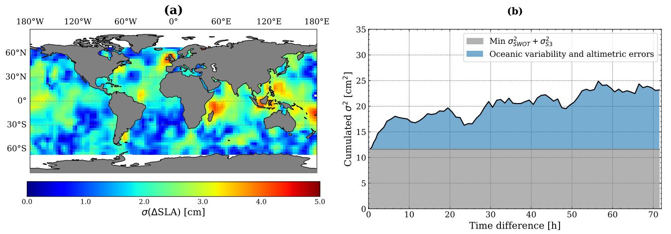
Figure 1. (a) Map of variability in 4-hours time interval, from SWOT KaRIn and S3A and S3B dual-crossovers and (b) Time series of the cumulated variance of \Delta\text{SLA} ; decomposition between instrumental errors (grey) and oceanic variability (blue).
