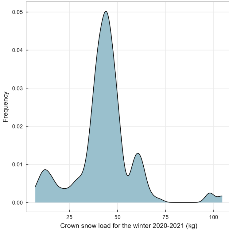
Figure A 3. Frequency distribution of the maximum calculated crown snow load (kg) for the winter 2020-2021 for the 25 individual powerline strips and 180 recorded damaged trees. Briefly, crown snow load was calculated hourly for the 2013-2023 timeseries using (Lehtonen et al., 2014) on the hourly meteorological data from the long-term stable post-processed products of the Norwegian Meteorological Institute MET ( https://thredds.met.no/thredds/metno.html ) at a 1km resolution. The maximum for the winter season 2020- 625 2021 was then extracted for the grid cells corresponding to each of the 205 locations (25 powerline strips and 180 fallen trees).
