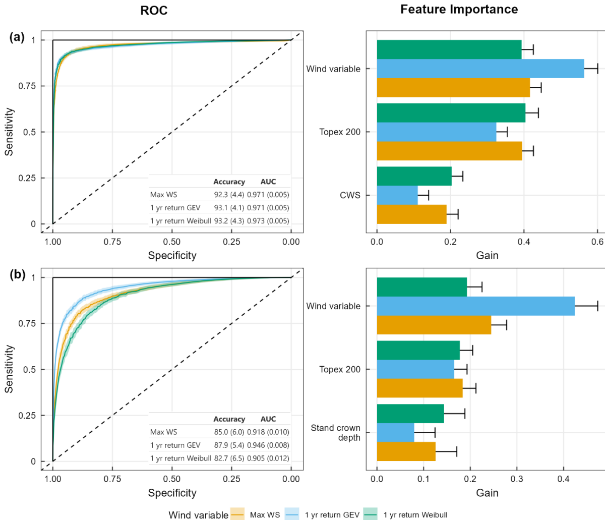
Figure 4. Summary of the XGBoost algorithms performance (ROC curve; left) and feature importance for the top three contributing variables (right) when using the “ForestGALES-ML” dataset (panels a) and the “TreeChar-ML” dataset (panels b) for the 100 repetitions across the three alternatives for the wind variables. The three alternatives are: Max WS (in orange), the 1-yr return GEV (blue) and the 1-yr return Weibull (green). The mean (and sd) AUC and accuracy across the 100 repetitions of the 10-folds cross-validation procedure for each alternative of the wind variables are shown as a table in the two left panels.
