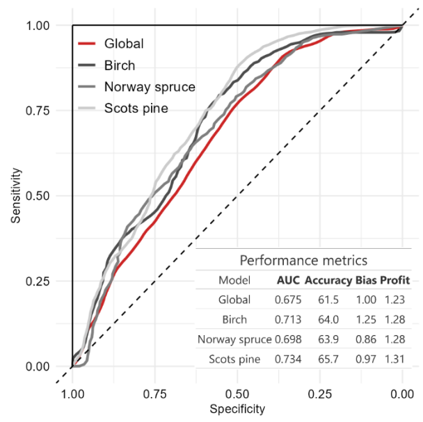
460 Figure 33. Receiver Operator Characteristic (ROC) curve and performance metrics for the prediction of the probability of tree damage during the winter 2020-2021 using the best global and species-specific model options (see Table 2 Table 2). All samples were used in this figure (The average of the 100 repeated assessments using balanced sample of N_{damaged} damaged = N_{standing} = 180; N_{standing} = 18,189 ), was used for the figure. The AUC is shown in the table, along with the summary of the average performance metrics (Accuracy in percentage, Bias, and Profit scores) for the cutpoint at which Sensitivity = Specificity.
