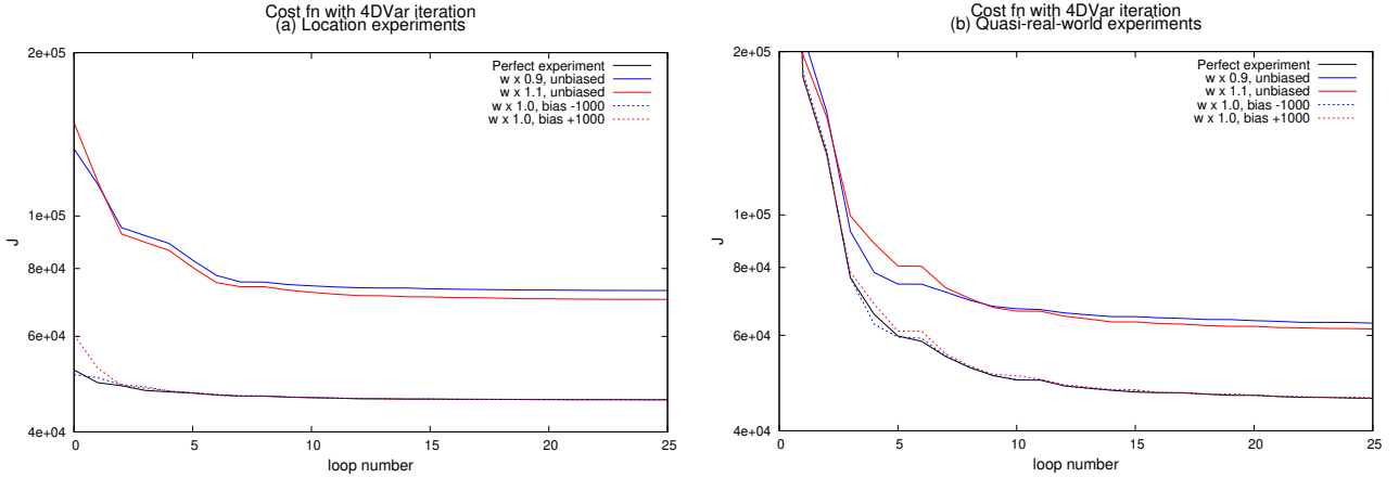
Figure F1. Variation of the cost function, J , Eq. (5), with the 4D-Var loop number. Panel (a) is for a selection of experiments in the weakly Bayesian location regime (Sect. 4) and (b) in the Bayesian quasi-real-world regime (Sect. 5). The black lines are for the perfect experiments (no model error, no observation biases), the coloured continuous lines are for the model error experiments, and the dotted lines are for the observation bias experiments.
