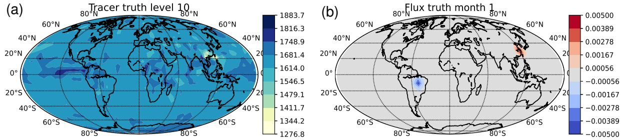
Figure 4. The true state chosen for the source/sink location detection experiments. Panel (a) is for \chi^t(0) at level 10 (850m above the ground, units \mu\text{gkg}^{-1} ) and panel (b) is for \rho^t(0) (corresponding to the first 30 days, units \mu\text{gm}^{-2}\text{s}^{-1} ). In (b), red is a source and blue is a sink.
