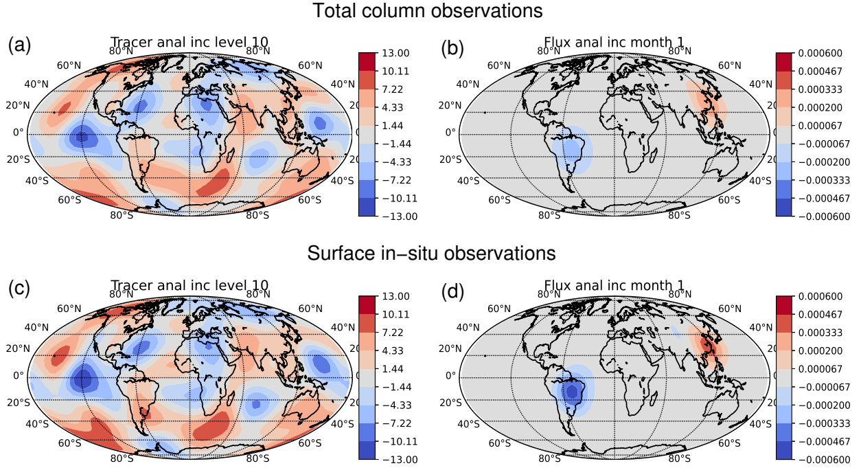
Figure 5. Analysis increments, \delta\chi^a(0) (units \mu\text{gkg}^{-1} ) and \delta\rho^a(0) (units \mu\text{gm}^{-2}\text{s}^{-1} ), found by assimilating either TCA (top row) or SIS observations (bottom row) for the near perfect source/sink location detection experiments. Panels (a) and (c) are for \delta\chi^a(0) at level 10, and panels (b) and (d) are for \delta\rho^a(0) . These plots should be compared to the true fields in Fig. 4. Red increments are positive and blue increments are negative. When comparing panels (b) and (d) to Fig. 4(b), note the different colour scales.
