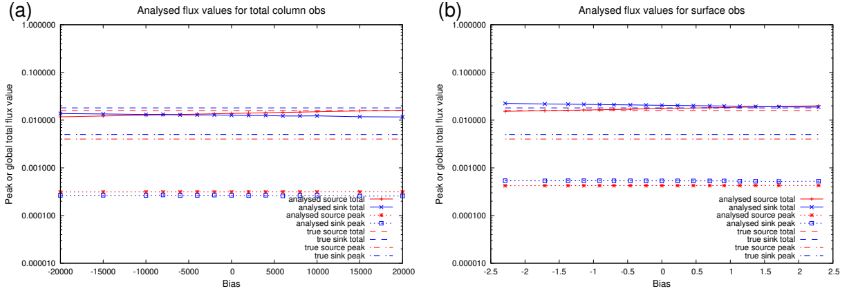
Figure 8. As Fig. 7(a) and (c) but for how the analysed global total, and the peak sources and sinks vary with observation bias. Panel (a) is for the TCA observations and (b) is for the SIS observations. The units are: global total values \text{Tg month}^{-1} and peak fluxes \mu\text{gm}^{-2}\text{s}^{-1} .
