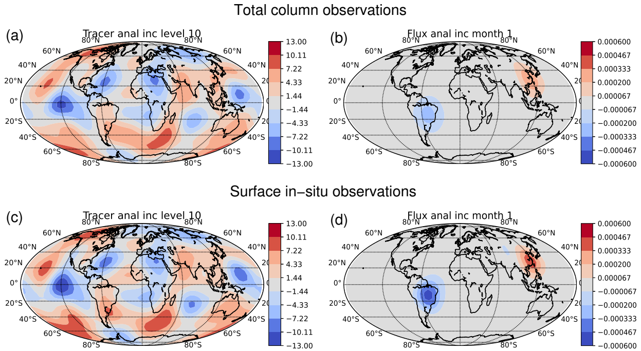
Figure 5. Analysis increments, \delta\chi^a(0) (units \text{ppb}\mu\text{gkg}^{-1} ) and \delta\rho^a(0) (units \mu\text{gm}^{-2}\text{s}^{-1} ), found by assimilating either TCA (top row) or SIS observations (bottom row) for the near perfect source/sink location detection experiments. Panels (a) and (c) are for \delta\chi^a(0) at level 10, and panels (b) and (d) are for \delta\rho^a(0) . These plots should be compared to the true fields in Fig. 4. Red increments are positive and blue increments are negative. When comparing panels (b) and (d) to Fig. 4(b), note the different colour scales.
