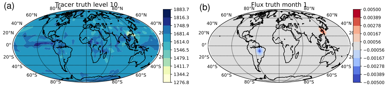
Figure 4. The true state chosen for the source/sink location detection experiments. Panel (a) is for \chi^t(0) at level 10 (850m above the ground, units \text{ppb} \mu\text{gkg}^{-1} ) and panel (b) is for \rho^t(0) (corresponding to the first 30 days, units \mu\text{gm}^{-2}\text{s}^{-1} ). In (b), red is a source and blue is a sink.
