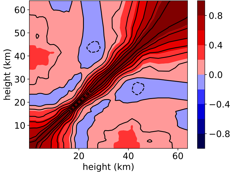
Correlation matrix: Global average vertical cor matrix
