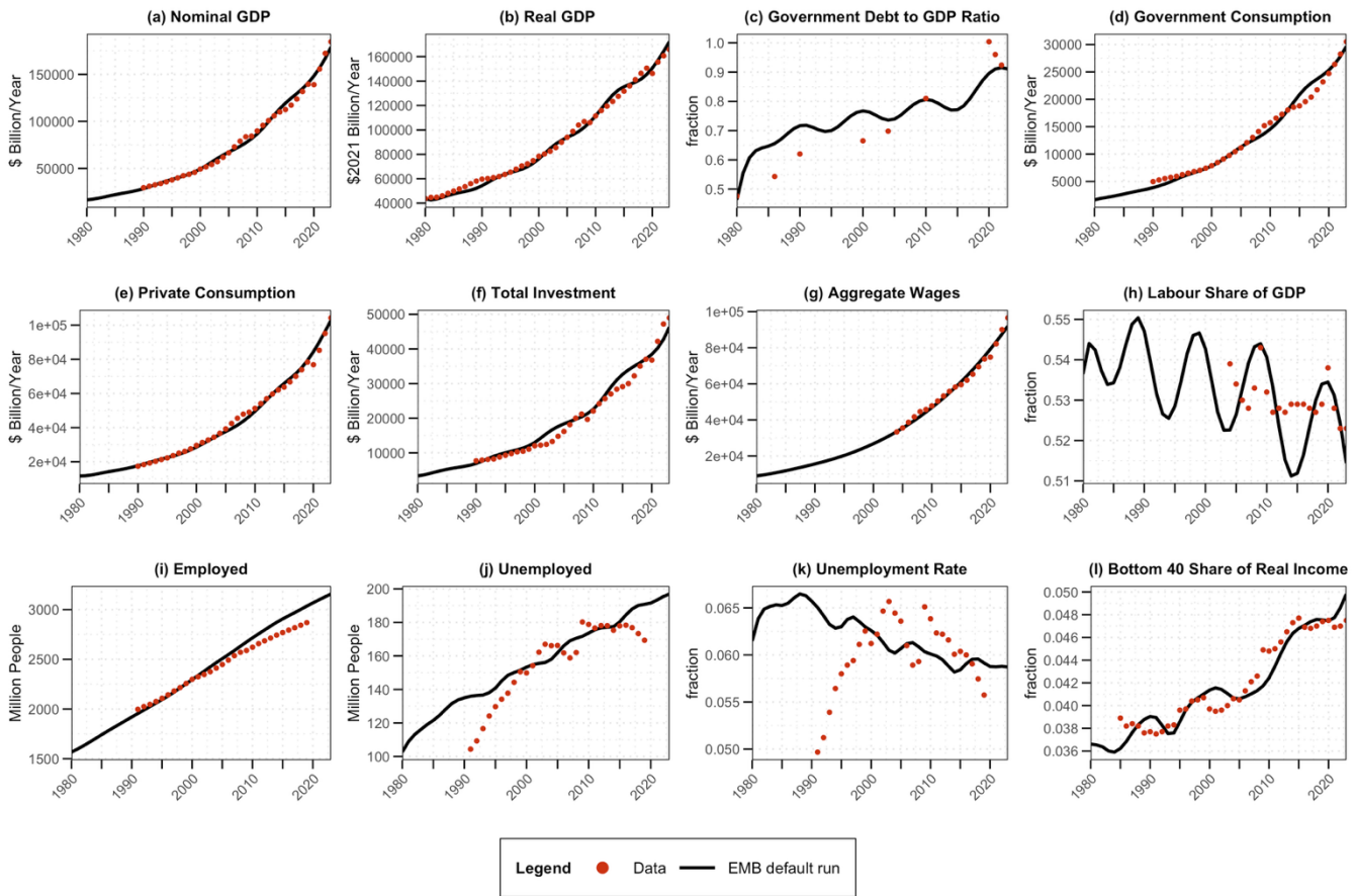
Figure 6: Best fit FRIDA results for key macroeconomic indicators against observed data.
