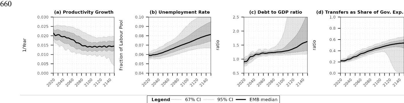
Figure 10: Changes in labour productivity, unemployment rate, government debt to GDP, and the share of government expenditure spent on transfers across the 100,000-member ensemble. Solid lines show the median, darker shaded areas show the 67% confidence intervals, and lighter shaded areas show the 95% confidence intervals.
