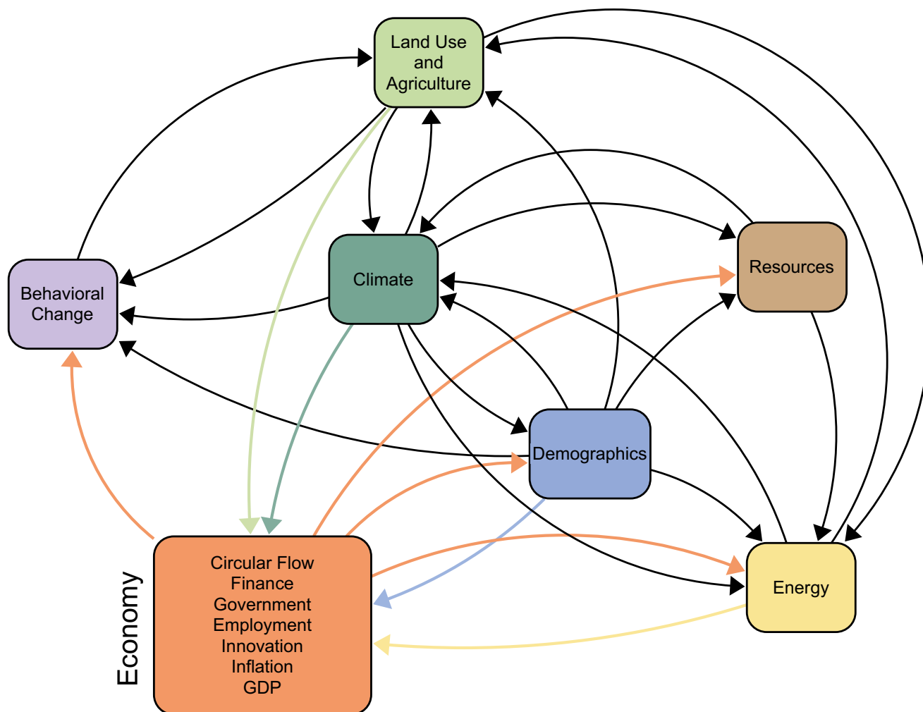
225 Figure 1: The seven high-level modules comprising the FRIDA model, the connections between them, and the Economy module's 230 component submodules.
