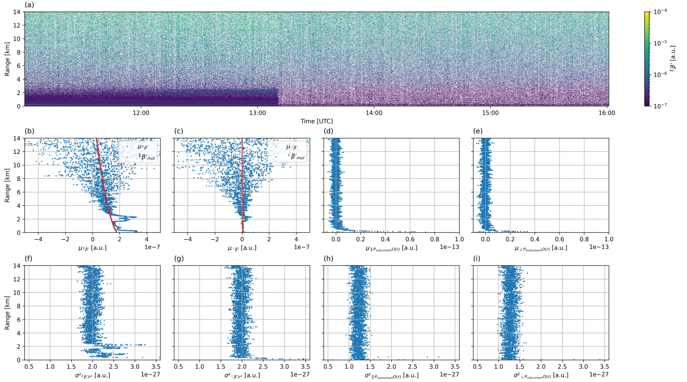
Figure 3. Measurements at Kenttäröva on 5 March 2024. (a) the time series of \parallel \beta' . Panels b, c, f, g, display the averaged profiles in time at each range gate before the termination hood measurement (from 11 to 13 UTC): (b) \mu_{\parallel \beta'} and \parallel \beta'_{\text{mol}} , (c) \mu_{\perp \beta'} and \perp \beta'_{\text{mol}} , (f) \sigma^2_{\parallel \beta' / r^2} , (g) \sigma^2_{\perp \beta' / r^2} . Panels d, e, h, i, display the averaged profiles in time at each range gate during the termination hood measurement at 19 °C (from 14 to 15 UTC): (d) \mu_{\parallel P_{\text{instrument}} O(r)} , (e) \mu_{\perp P_{\text{instrument}} O(r)} , (h) \sigma^2_{\parallel P_{\text{instrument}} O(r)} , (i) \sigma^2_{\perp P_{\text{instrument}} O(r)} .
