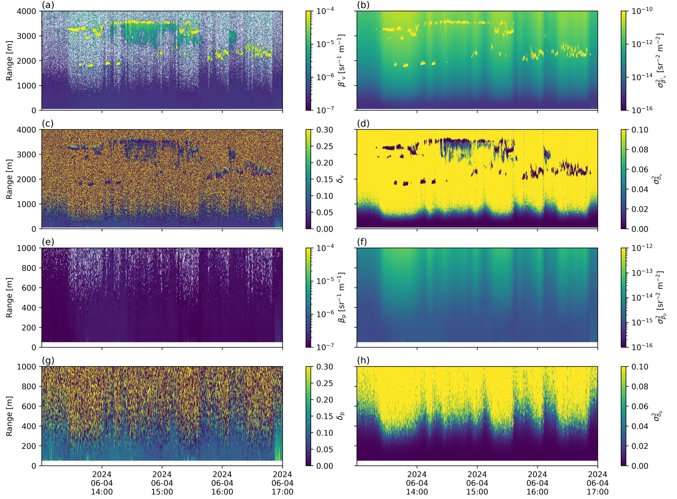
Figure 11. An example of corrected and calibrated profile in Kenttäröva on 4 June 2024 13:00 - 17:00 UTC (same day as Fig. 10). (a) \beta'_v , (b) \sigma_{\beta'_v}^2 , (c) \delta_v , (d) \sigma_{\delta_v}^2 , (e) \beta_p , (f) \sigma_{\beta_p}^2 , (g) \delta_p , and (h) \sigma_{\delta_p}^2 . For particle properties in panels e-h, profiles are shown only up to 1 km range.
