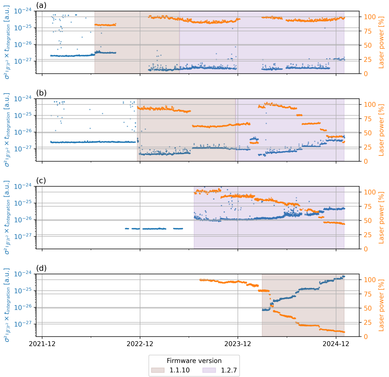
Figure 4. Time series of nighttime background signal variance normalized by the integration time ( \sigma^2_{\parallel \beta' / r^2} \times t_{\text{integration}} ), and the laser power are shown for (a) Vehmasmäki, (b) Hyytiälä, (c) Kenttäröva, and (d) Lindenberg. Shaded regions denote different firmware versions; unshaded areas represent periods with no recorded firmware version and laser power.
