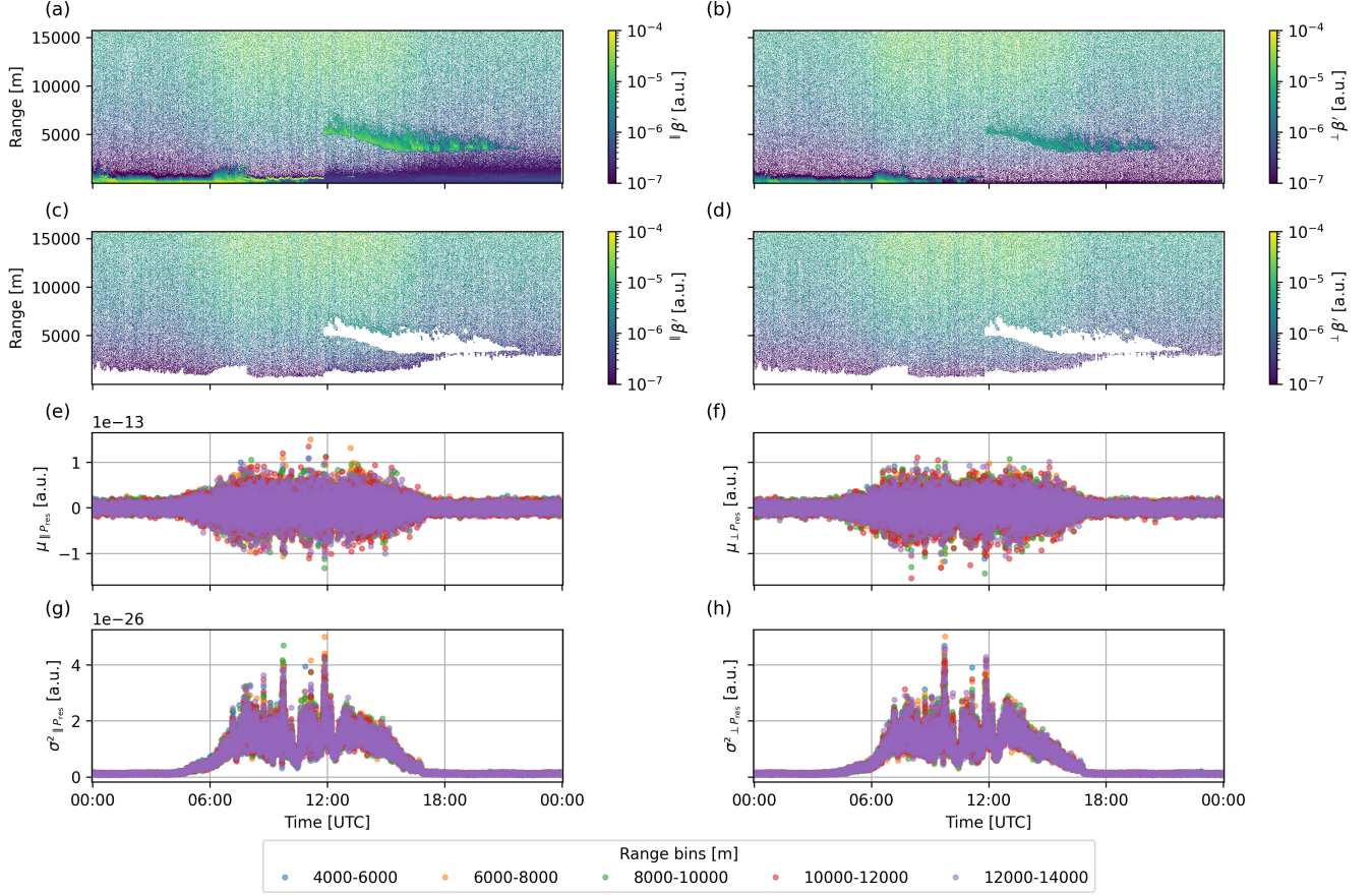
Figure 1. Time series from Kenttäröva on 28 March 2024 showing: (a) |\beta'| , (b) |\beta'| , (c) background |\beta'| , and (d) background |\beta'| . Subplots (e) to (h) display the background at different range bins from 4000 to 6000 m, 6000 to 8000 m, 8000 to 10000 m, 10000 to 12000 m, and 12000 to 14000 m, with color indicating the range bin: (e) \mu_{||P_{res}} , (f) \mu_{\perp P_{res}} , (g) \sigma^2_{||P_{res}} , and (h) \sigma^2_{\perp P_{res}} . These parameters are computed at a 10-second temporal resolution using all data within each range bin.
