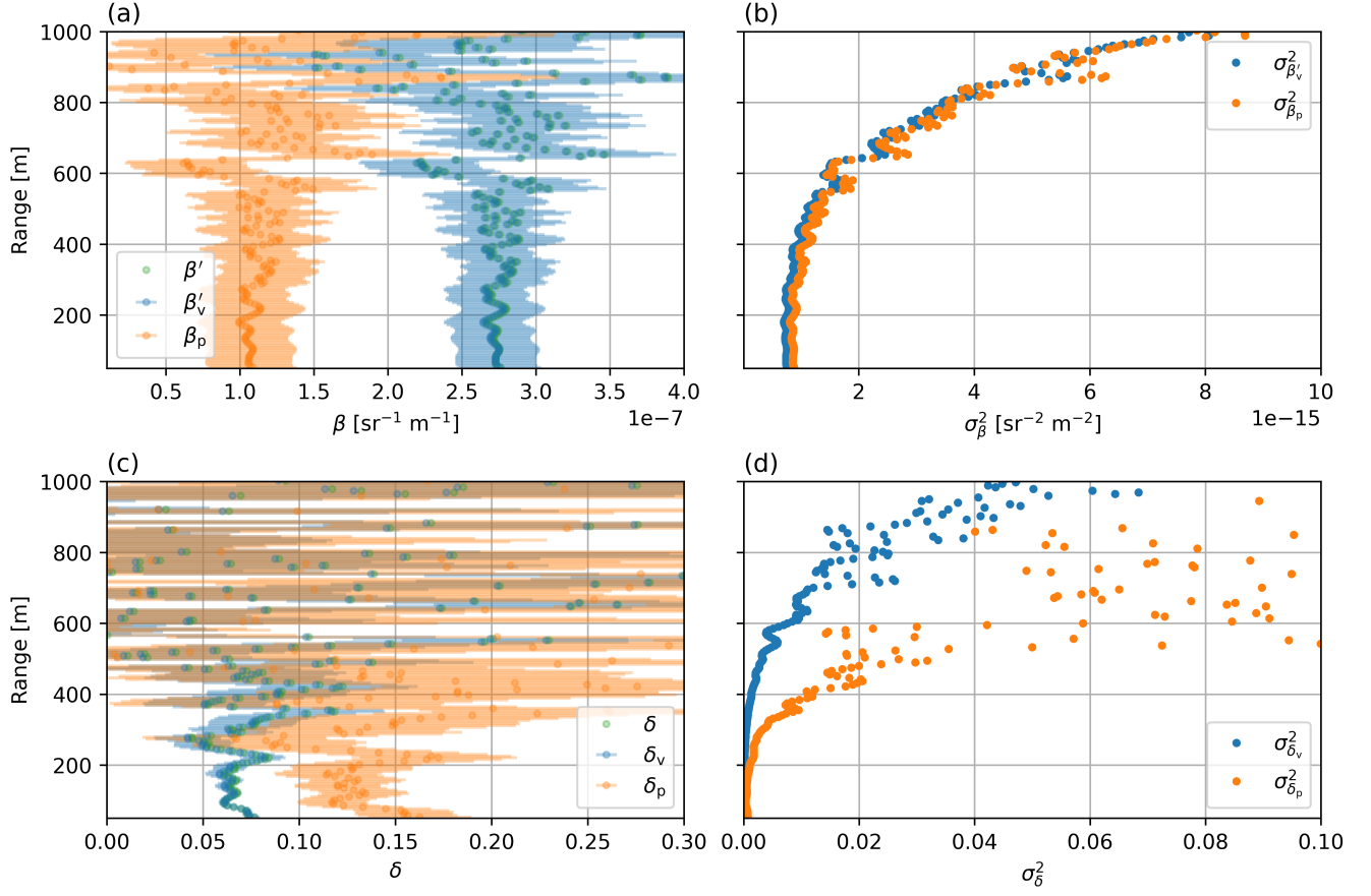
Figure 10. Example of uncorrected and corrected profiles in Kenttäröva measured at 4 June 2024 13:01 UTC. (a) \beta' (instrument provided), \beta'_v (bias corrected and calibrated), \beta_p , (b) \sigma_{\beta'_v}^2 , \sigma_{\beta_p}^2 , (c) \delta (instrument provided), \delta_v (bias corrected and calibrated), \delta_p , (d) \sigma_{\delta_v}^2 , \sigma_{\delta_p}^2 . Error bars represent one standard deviation ( \sigma ) of the measurements.
