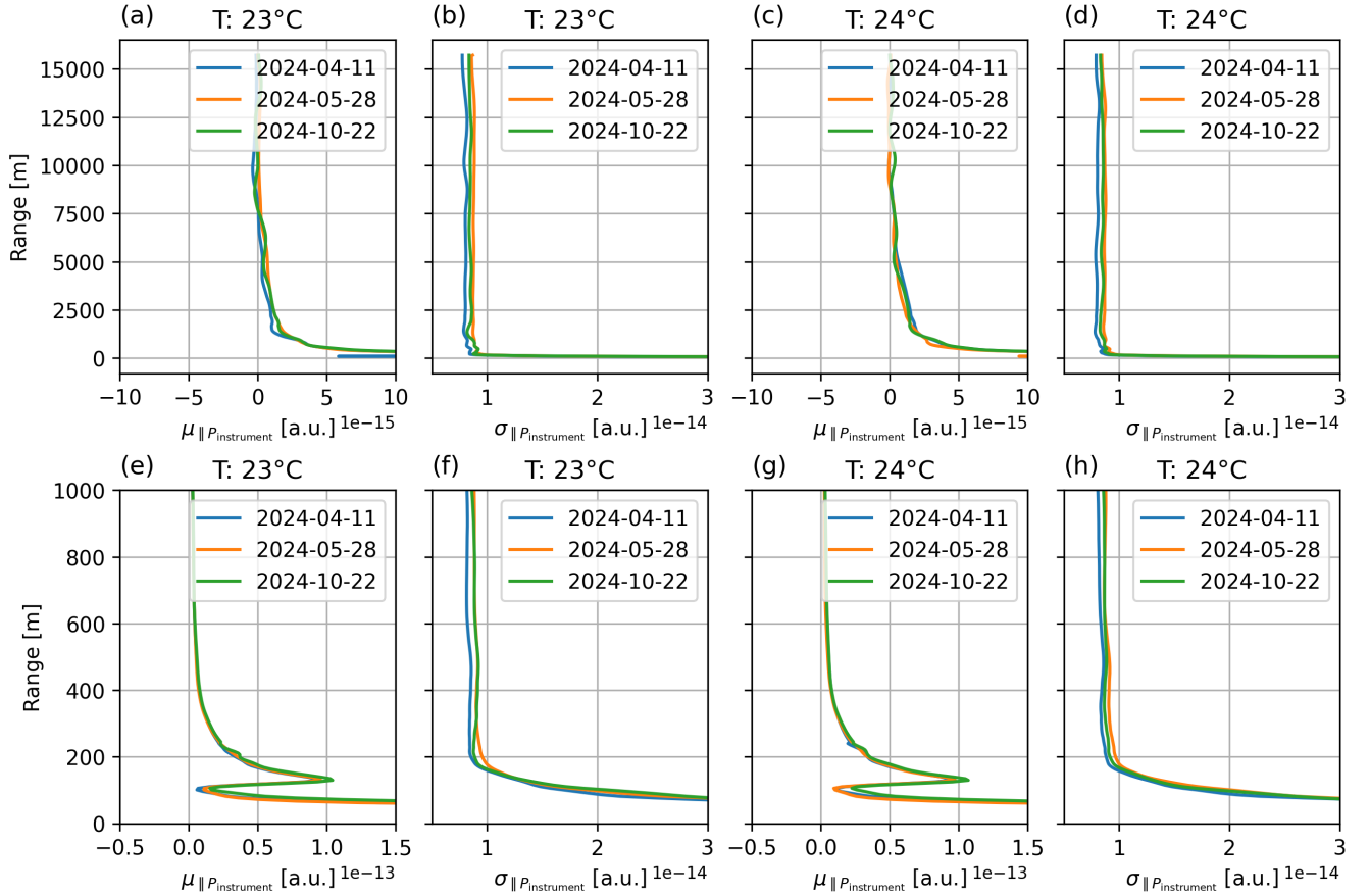
Figure 8. Termination hood profiles in Vehmassmäki at 23°C (panels (a), (b), (e), and (f)), and 24°C (panels (c), (d), (g), (h)). These measurements were recorded at three different time points over a six-month period in 2024. Panels (a), (c), (e), and (g) display \mu_{\parallel\beta'} , while panels (b), (d), (f), (h) display \sigma_{\parallel\beta'} .
