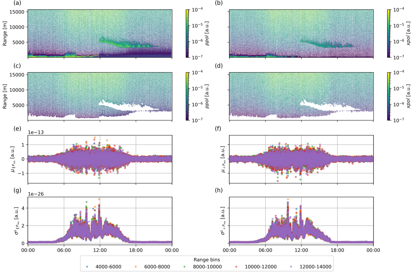
Figure 1. Time series from Kenttäröva on 2024-03-28 showing: a) ppol , b) xpol , c) background ppol , and d) background xpol . Subplots e–h display the background signals at different range bins from 4000 – 6000 m, 6000 – 8000 m, 8000 – 10000 m, 10000 – 12000 m, 12000 – 14000 m, with color indicating the range bin: e) \mu_{\parallel P_{res}} , f) \mu_{\perp P_{res}} , g) \sigma^2_{\parallel P_{res}} , and h) \sigma^2_{\perp P_{res}} . These parameters are computed at a 10-second temporal resolution using all data within each range bin.
