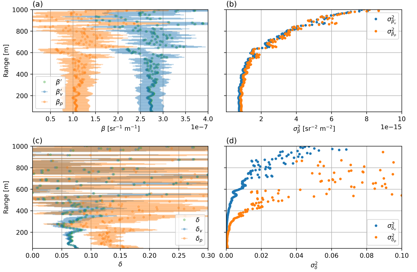
Figure 10. Example of uncorrected and corrected profiles in Kenttäröva measured at 2024-06-04 13:01 UTC. a) \beta' (instrument provided), \beta'_v (bias corrected and calibrated), \beta_p , b) \sigma_{\beta'_v}^2 , \sigma_{\beta_p}^2 , c) \delta (instrument provided), \delta_v (bias corrected and calibrated), \delta_p , d) \sigma_{\delta_v}^2 , \sigma_{\delta_p}^2 . Error bars represent one standard deviation ( \sigma ) of the measurements.
