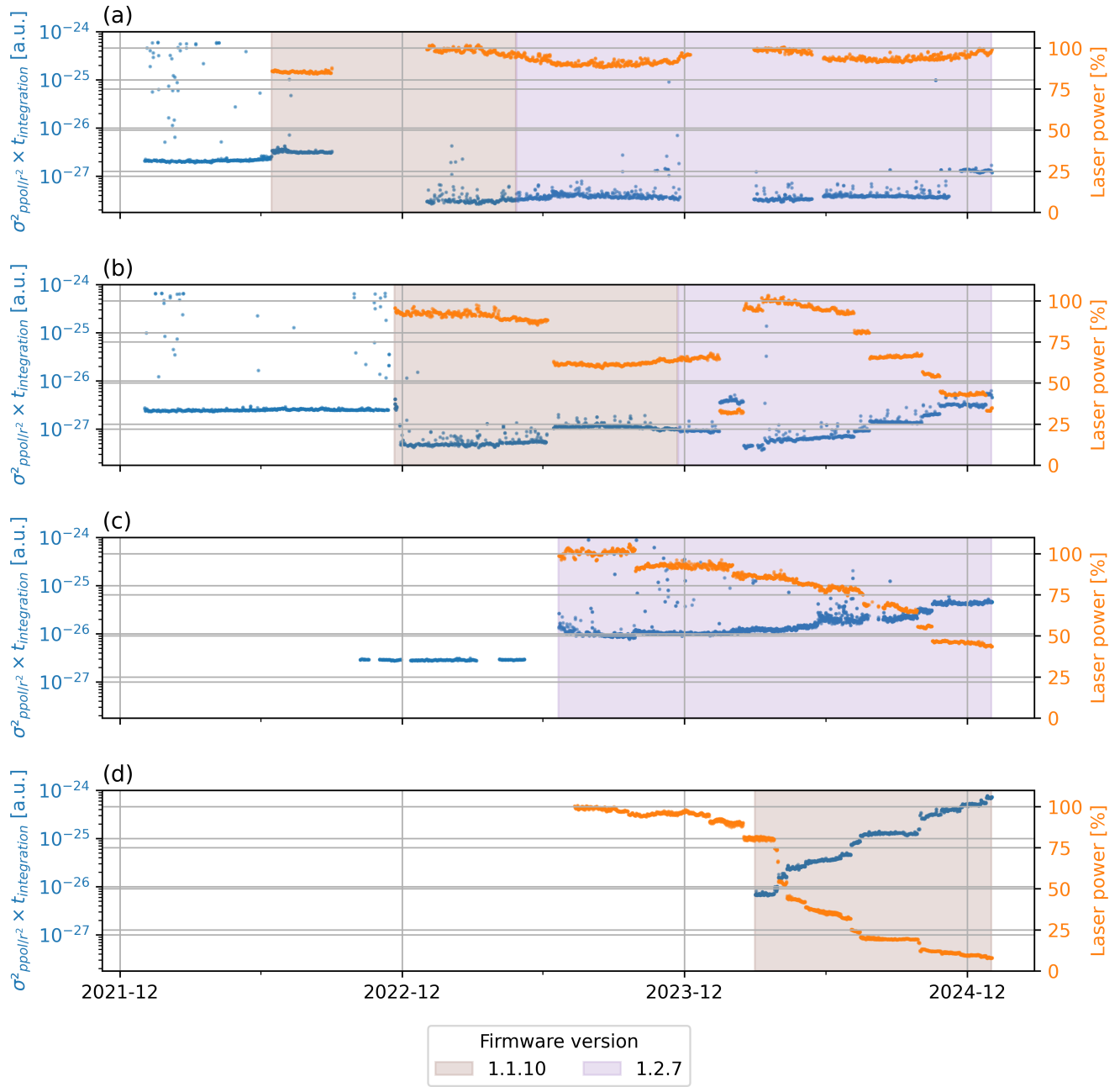
Figure 4. Time series of nighttime background signal variance normalized by the integration time ( \sigma_{ppol/r^2}^2 \times t_{integration} ), and the laser power are shown for (a) Vehmasmäki, (b) Hyytiälä, (c) Kenttäröva, and (d) Lindenberg. Shaded regions denote different firmware versions; unshaded areas represent periods with no recorded firmware version and laser power.
