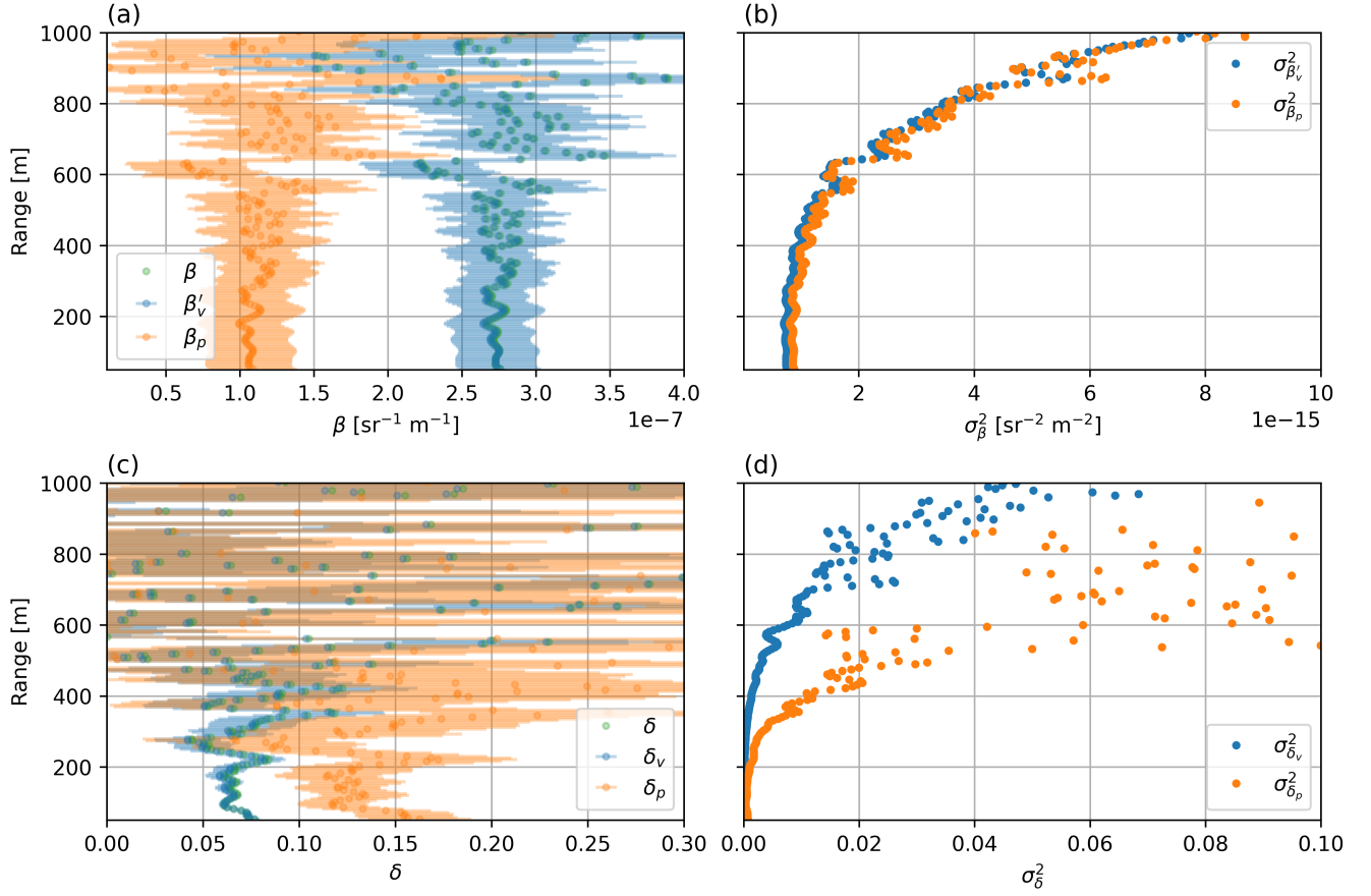
Figure 10. Example of uncorrected and corrected profiles in Kenttäröva measured at 2024-06-04 13:01 UTC. a) \beta (instrument provided), \beta'_v (bias corrected and calibrated), \beta_p , b) \sigma_{\beta'_v}^2 , \sigma_{\beta_p}^2 , c) \delta (instrument provided), \delta_v (bias corrected and calibrated), \delta_p , d) \sigma_{\delta_v}^2 , \sigma_{\delta_p}^2 .
