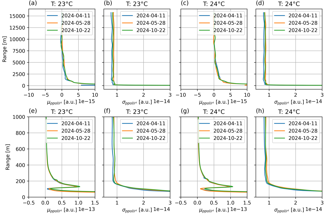
Figure 8. Calibration profiles in Vehmasmäki at 23°C and 24°C, recorded at three different time points over a six-month period in 2024.
