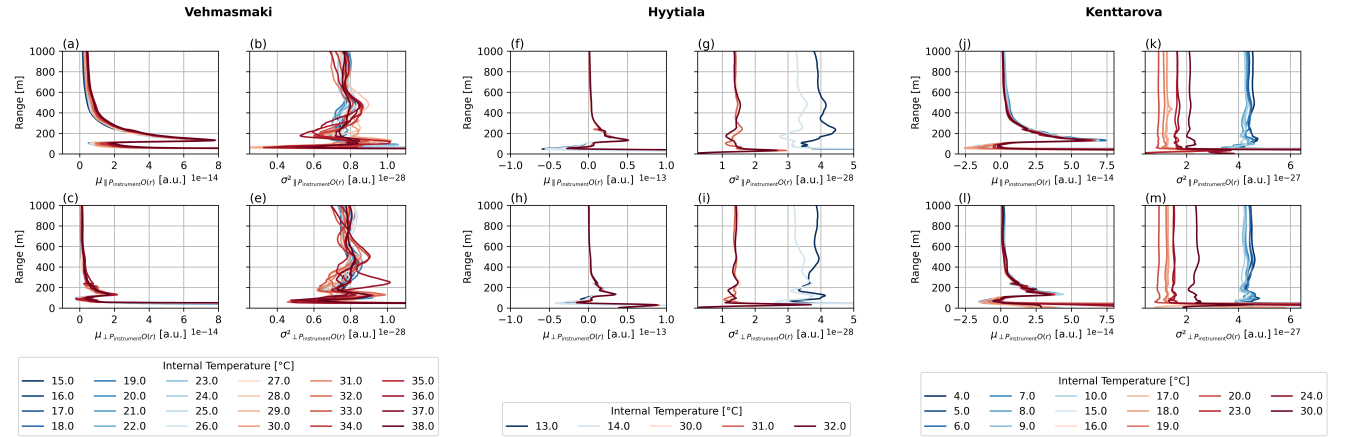
Figure 7. Termination hood profiles at various internal temperatures (color-coded) across different sites only up to 1000 m range. In Vehmasmaki: a) \mu_{\parallel P_{\text{instrument}}O(r)} , b) \sigma_{\parallel P_{\text{instrument}}O(r)}^2 , c) \mu_{\perp P_{\text{instrument}}O(r)} , and d) \sigma_{\perp P_{\text{instrument}}O(r)}^2 . In Hyttiala: f) \mu_{\parallel P_{\text{instrument}}O(r)} , g) \sigma_{\parallel P_{\text{instrument}}O(r)}^2 , h) \mu_{\perp P_{\text{instrument}}O(r)} , and i) \sigma_{\perp P_{\text{instrument}}O(r)}^2 . In Kenttaro: j) \mu_{\parallel P_{\text{instrument}}O(r)} , k) \sigma_{\parallel P_{\text{instrument}}O(r)}^2 , l) \mu_{\perp P_{\text{instrument}}O(r)} , and m) \sigma_{\perp P_{\text{instrument}}O(r)}^2 .
