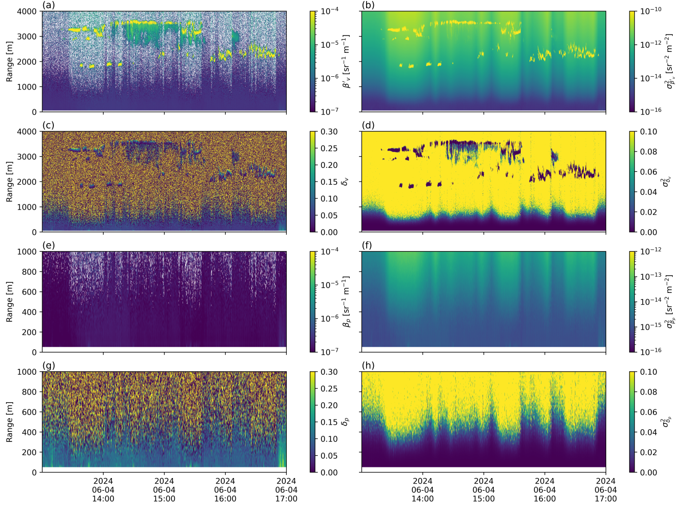
Figure 11. An example of corrected and calibrated profile in Kenttärova on 2024-06-04 13:00 - 17:00 UTC (same day as Fig. 10). a) \beta'_v , b) \sigma_{\beta'_v}^2 , c) \delta_v , d) \sigma_{\delta_v}^2 , e) \beta_p , f) \sigma_{\beta_p}^2 , g) \delta_p , and h) \sigma_{\delta_p}^2 . For particle properties in panels e-h, profiles are shown only up to 1 km range.
