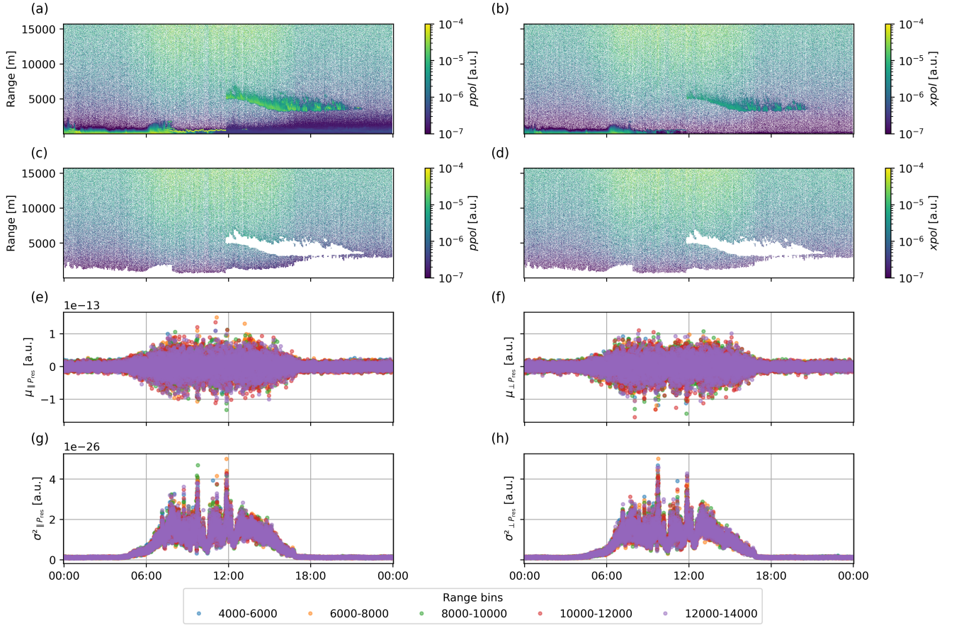
Figure 1. Time series from Kenttärova on 2024-03-28 showing: a) ppol , b) xpol , c) background ppol , and d) background xpol . Subplots e–h display the background signals at different range bins from 4000 – 6000 m, 6000 – 8000 m, 8000 – 10000 m, 10000 – 12000 m, 12000 – 14000 m, with color indicating the range bin: e) \mu_{\parallel P_{res}} , f) \mu_{\perp P_{res}} , g) \sigma^2_{\parallel P_{res}} , and h) \sigma^2_{\perp P_{res}} . These parameters are computed at a 10-second temporal resolution using all data within each range bin.
