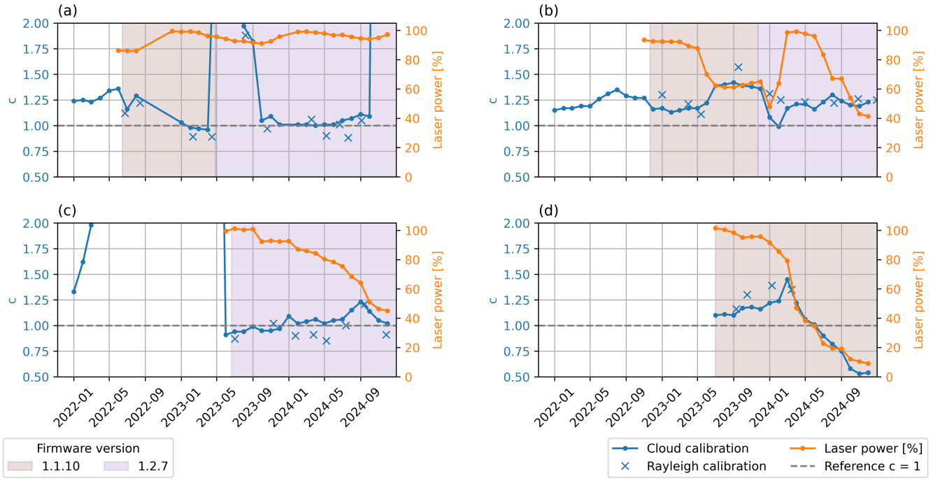
Figure 9. Time series of the calibration factor from cloud calibration, Rayleigh calibration and laser power at four sites: a) Vehmasmäki, b) Hyytiälä, c) Kenttäröva, and d) Lindenberg. The dashed line indicates a calibration factor of c = 1 . Periods corresponding to different firmware versions are highlighted with shaded areas.
