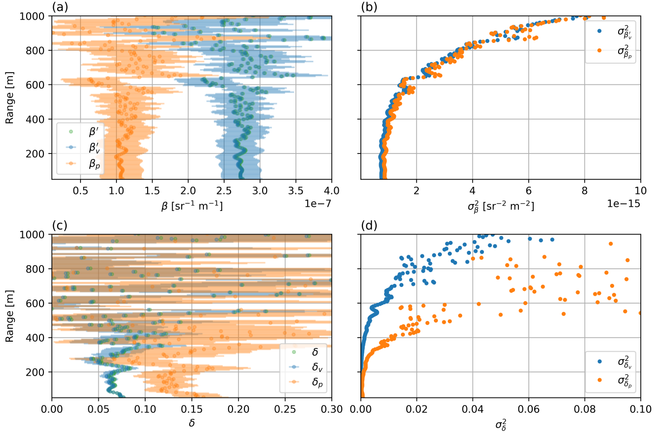
Figure 10. Example of uncorrected and corrected profiles in Kenttäröva measured at 2024-06-04 13:01 UTC. a) \beta , \beta' (instrument provided), \beta'_v (bias corrected and calibrated), \beta_p , b) \sigma_{\beta'_v}^2 , \sigma_{\beta_p}^2 , c) \delta (instrument provided), \delta_v (bias corrected and calibrated), \delta_p , d) \sigma_{\delta_v}^2 , \sigma_{\delta_p}^2 . Error bars represent one standard deviation ( \sigma ) of the measurements.
