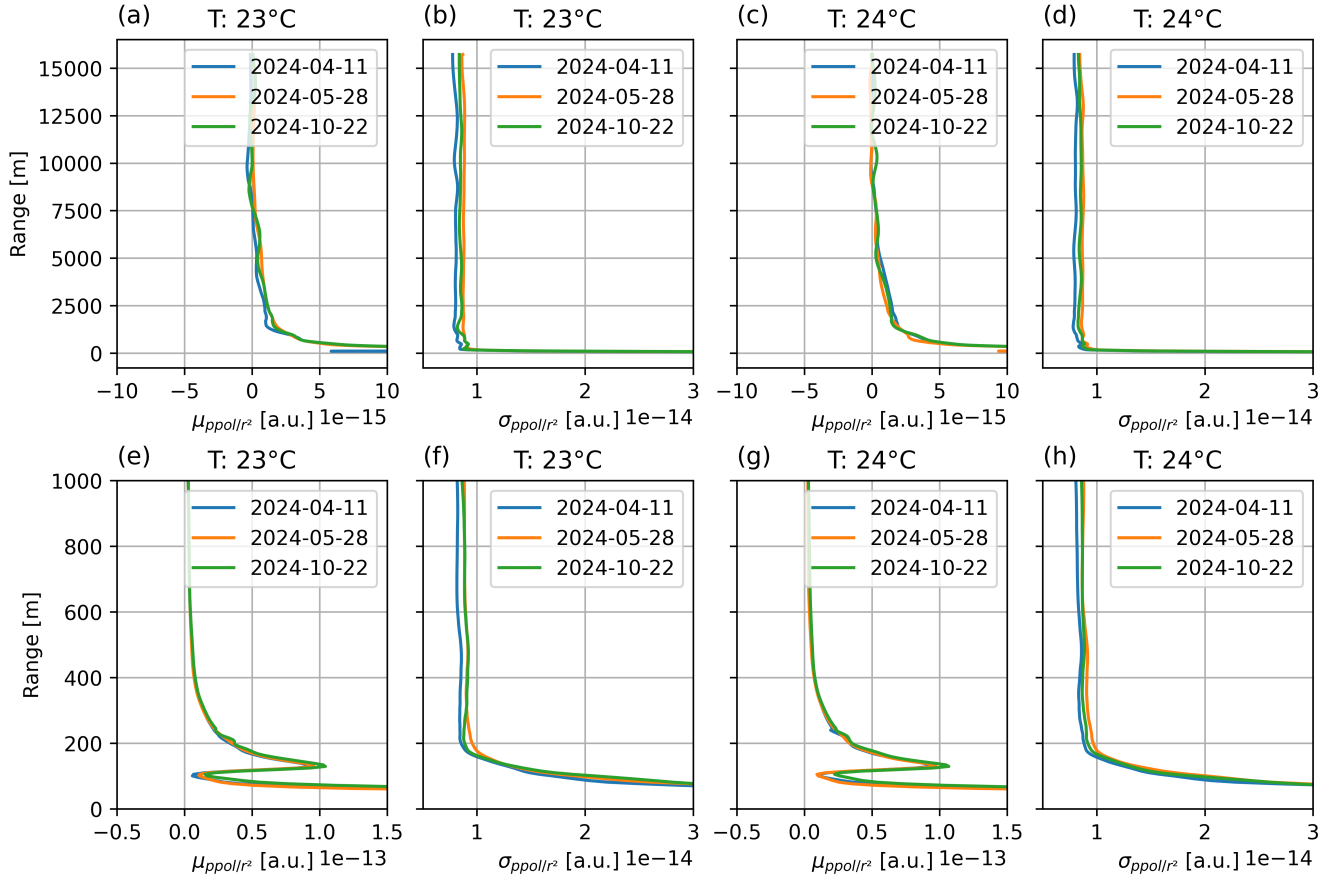
Figure 8. Calibration profiles in Vehmasmäki at 23°C and 24°C, recorded at three different time points over a six-month period in 2024.
