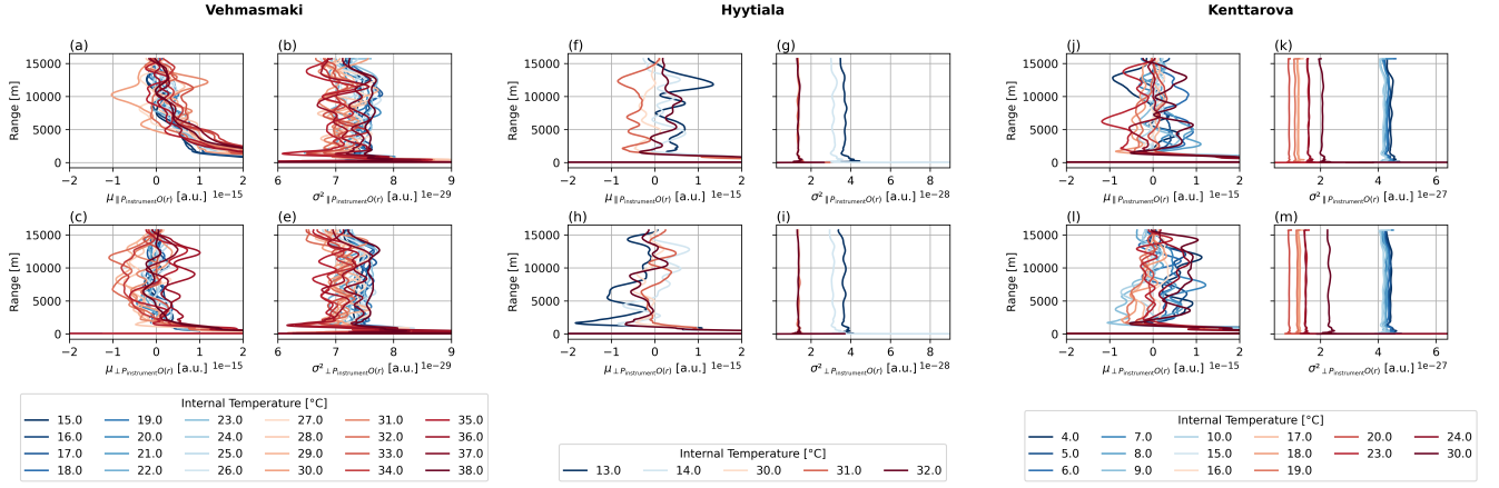
Figure 6. Termination hood profiles at various internal temperatures (color-coded) across different sites. In Vehmasmaki: a) \mu_{\perp} P_{\text{instrument}} Q(r) , b) \sigma_{\perp} P_{\text{instrument}} Q(r) , c) \mu_{\parallel} P_{\text{instrument}} Q(r) , and d) \sigma_{\parallel} P_{\text{instrument}} Q(r) . In Hyyttiala: f) \mu_{\perp} P_{\text{instrument}} Q(r) , g) \sigma_{\perp} P_{\text{instrument}} Q(r) , h) \mu_{\parallel} P_{\text{instrument}} Q(r) , and i) \sigma_{\parallel} P_{\text{instrument}} Q(r) . In Kenttaroava: j) \mu_{\perp} P_{\text{instrument}} Q(r) , k) \sigma_{\perp} P_{\text{instrument}} Q(r) , l) \mu_{\parallel} P_{\text{instrument}} Q(r) , and m) \sigma_{\parallel} P_{\text{instrument}} Q(r) .
