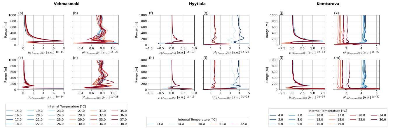
Figure 7. Termination hood profiles at various internal temperatures (color-coded) across different sites only up to 1000 m range. In Vehmasmaki: a) \mu_{\perp} P_{\text{instrument}} Q(r) , b) \sigma_{\perp} P_{\text{instrument}} Q(r) , c) \mu_{\parallel} P_{\text{instrument}} Q(r) , and d) \sigma_{\parallel} P_{\text{instrument}} Q(r) . In Hyyttiala: f) \mu_{\perp} P_{\text{instrument}} Q(r) , g) \sigma_{\perp} P_{\text{instrument}} Q(r) , h) \mu_{\parallel} P_{\text{instrument}} Q(r) , and i) \sigma_{\parallel} P_{\text{instrument}} Q(r) . In Kenttaroava: j) \mu_{\perp} P_{\text{instrument}} Q(r) , k) \sigma_{\perp} P_{\text{instrument}} Q(r) , l) \mu_{\parallel} P_{\text{instrument}} Q(r) , and m) \sigma_{\parallel} P_{\text{instrument}} Q(r) .
