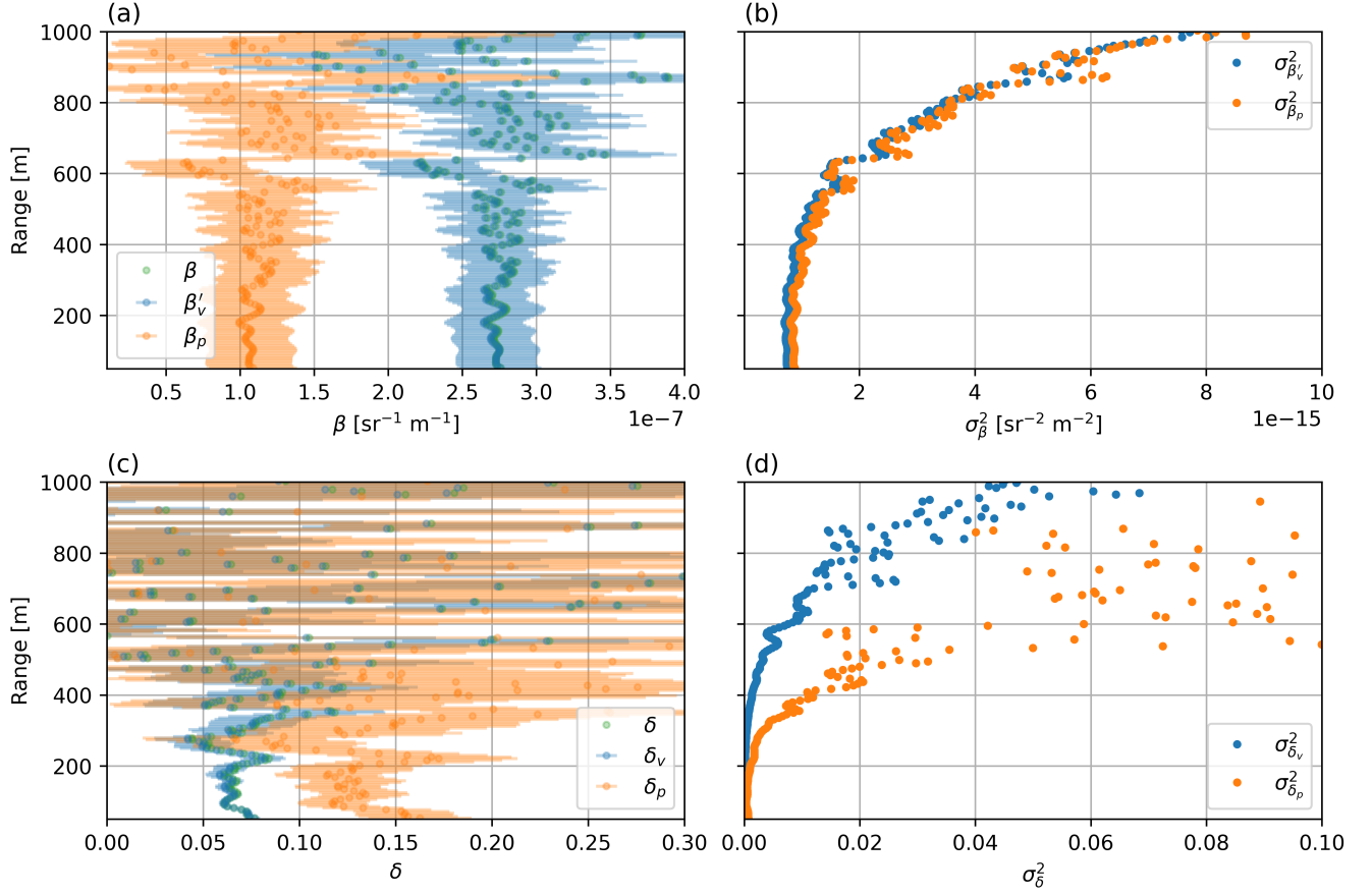
Figure 10. Example of uncorrected and corrected profiles in Kentärova-Kentärova measured at 2024-06-04 13:01 UTC. a) \beta ( instrument provided ), \beta_v ( bias corrected and calibrated ), \beta_p , b) \sigma_{\beta_v}^2 , \sigma_{\beta_p}^2 , c) \delta ( instrument provided ), \delta_v ( bias corrected and calibrated ), \delta_p , d) \sigma_{\delta_v}^2 , \sigma_{\delta_p}^2 .
