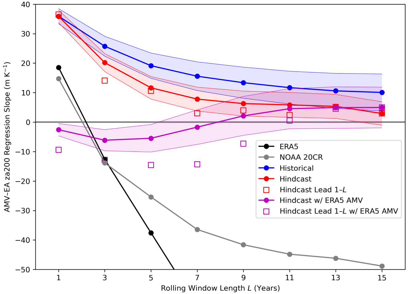
Figure 8. Regression slope between AMV and EA zonally anomalous 200 hPa geopotential height for different rolling window lengths L . Black: ERA5; Grey: NOAA 20CR with HadISST AMV; Blue: MPI-ESM-LR historical simulations; Red: MPI-ESM-LR hindcasts, for all leads (line and filled circles) and lead 1-L (squares); Purple: Hindcasts with ERA5 used for AMV, for all leads (line and filled circles) and lead 1-L (squares). Where the values are for all leads, values are computed individually for each lead, and then averaged. Shaded red and purple regions show the 5–95 confidence interval for the hindcasts at all leads with hindcast and ERA5 AMV respectively, computed as the mean value \pm the standard error of slopes from individual member timeseries scaled by 1.644. The shaded blue region shows the 5–95 confidence interval for the historical simulations, computed in the same manner. An alternative version showing the full curves for reanalyses can be found in the supplementary (Figure S2)
