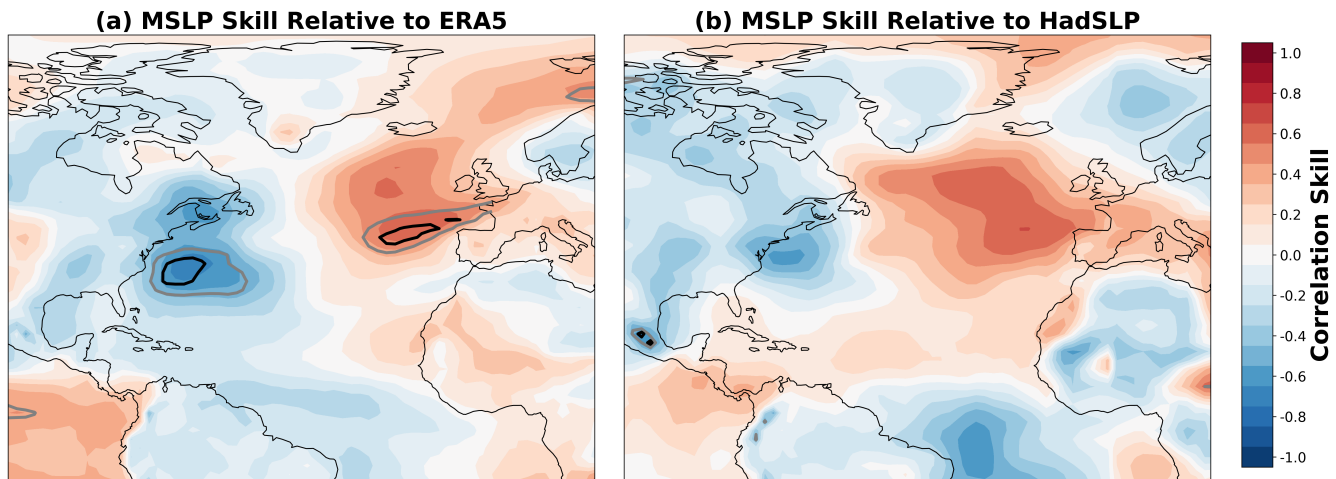
Figure 3. Decadal hindcast skill for MSLP. Temporal correlation between the decadal hindcast ensemble mean MSLP for lead years 1–7 and 7 year rolling mean MSLP from (a) ERA5 and (b) HadSLP. Grey and black contours enclose regions where zero correlation is outside of the 10–90 and 5–95 confidence interval for the correlation skill, respectively. Hindcasts initialised from 1960 to 2005 for HadSLP and to 2016 for ERA5 are considered to cover the respective common periods.
