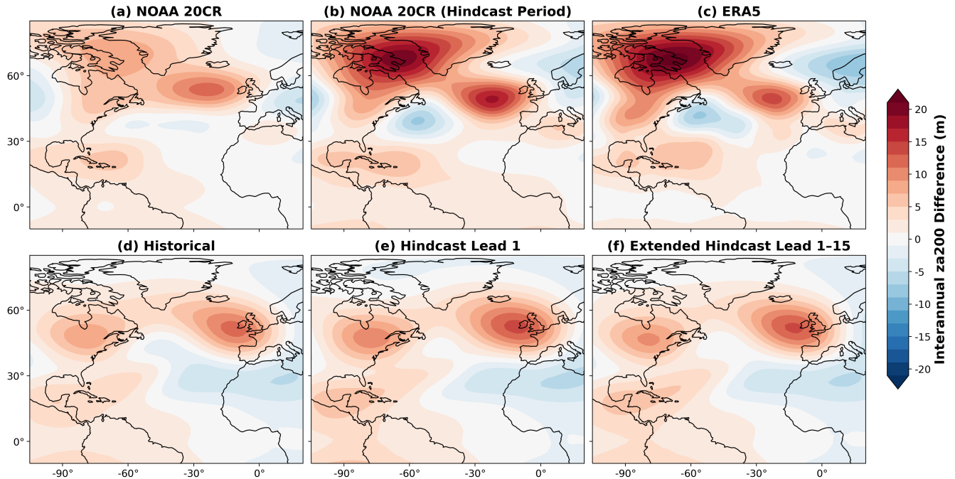
Figure 7. Year-on-year 200 hPa geopotential height response to year-on-year -AMV index variability in reanalysis and MPI-ESM-LR model experiments, where year-to-year - year-on-year variability is computed as half the difference between consecutive years ( see Section 2 for more details ). Composite difference in MSLP-200 hPa geopotential height during positive and negative interannual AMV index years using MSLP-geopotential height and SSTs from (a) NOAA 20CR/HadISST; (b) NOAA 20CR/HadISST during the common period of the decadal hindcasts and NOAA 20CR only; (c) ERA5 during the hindcast period; (d) historical runs using MPI-ESM-LR, (e) MPI-ESM-LR decadal hindcasts for lead year 1 and (f) single years for leads 1 to 15 in the 16 extended length members of the MPI-ESM-LR decadal hindcasts. Note that the zonal mean is removed in each case, as with the 7 year rolling mean results shown in Figure 5.
