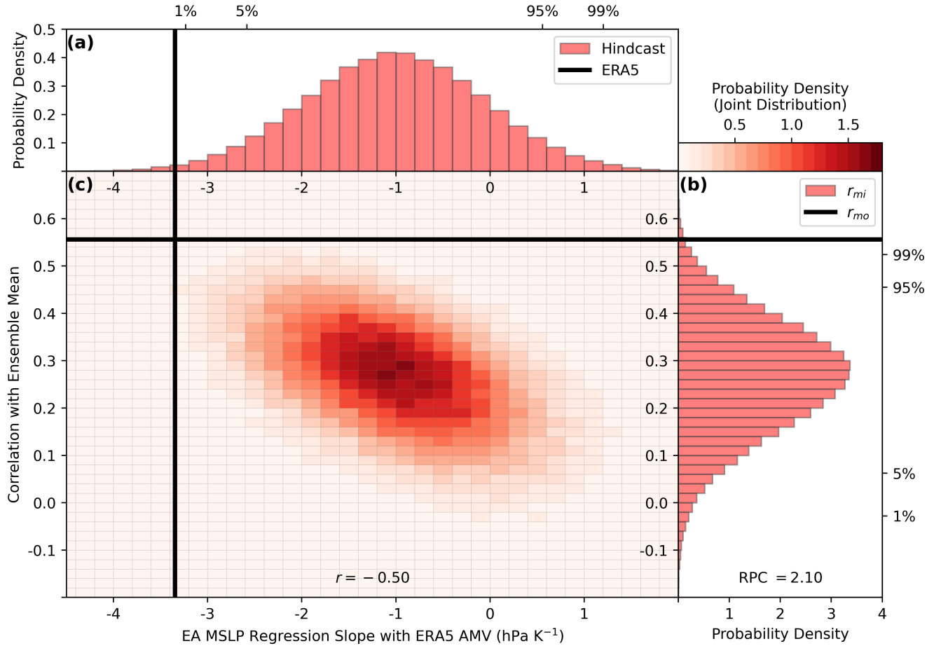
Figure 4. Teleconnection strength deficiencies lead to signal-to-noise errors. (a) (top) histogram of regression slopes for 100,000 samples of single member East Atlantic (EA) MSLP timeseries with the ERA5 AMV Index, along with the same slope but for ERA5 EA MSLP (black line). (b) (right) histogram of correlations r_{mi} of sampled hindcast member EA MSLP with ensemble mean EA MSLP, along with the correlation between ERA5 and the ensemble mean (black line). (c) (main) joint histogram for the sampled hindcast member statistics in (a) and (b). Black lines in (a) and (b) extend in to (c). In (a) and (b), cumulative 1, 5, 95 and 99% levels for the histograms are shown. All fields are 7 year JJA means, with hindcasts initialised from 1960 to 2016 inclusive considered to cover the full common period.
