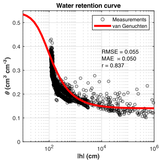
Figure 5 Volumetric water content ( \theta ) as a function of pressure head ( |h| ). Points represent measurements, while the solid red line denotes the optimized van Genuchten water retention function. Performance metrics (RMSE, MAE, and Pearson's correlation coefficient, r ) are reported.
