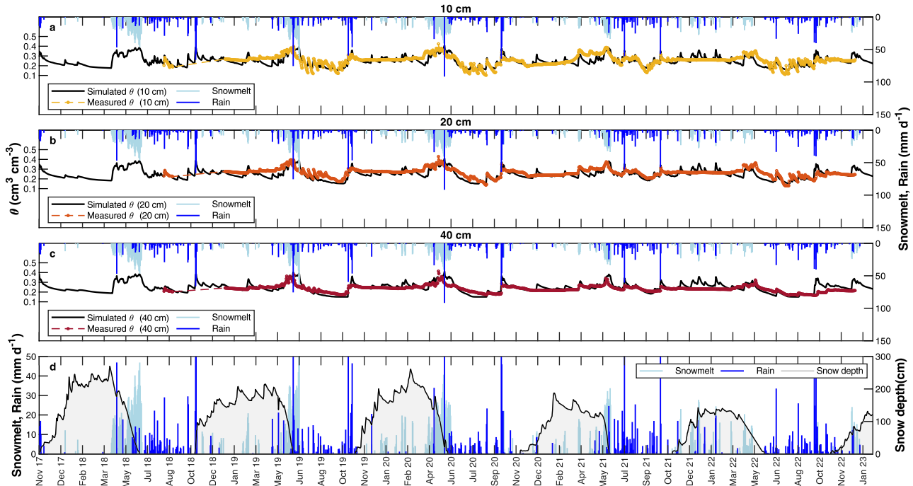
Figure 7 Measured (line with markers) and simulated (line) volumetric water content at (a) 10 cm, (b) 20 cm and (c) 40 cm. Snowmelt and rain have been also indicated. (d) Snow depth, snowmelt and rain. \theta indicates the volumetric water content.
