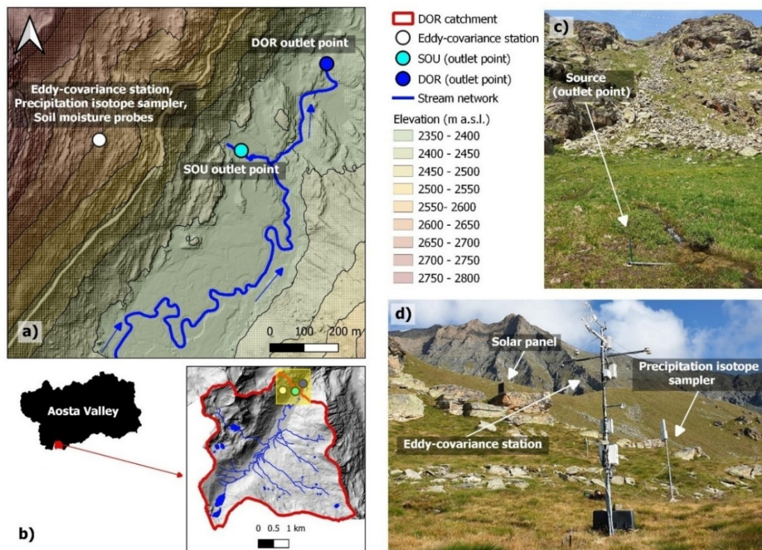
200 Figure 2 (a) Location of the study site within the Dora del Nivolet (DOR) catchment. Soil samples and lignified twigs/roots are collected nearby the eddy-covariance station where also volumetric water content and matric potential (10, 20, 40 cm depth) are measured. Blue arrows indicate the flow direction (b) Geographical framework of the DOR catchment (c) Photo (02-Jul-2019) of the monitored source (SOU) (d) Photo (23-Aug-2019) of the eddy-covariance station and of the precipitation isotope sampler. In the background it is possible to observe the solar panel that supplies the eddy-covariance station.
