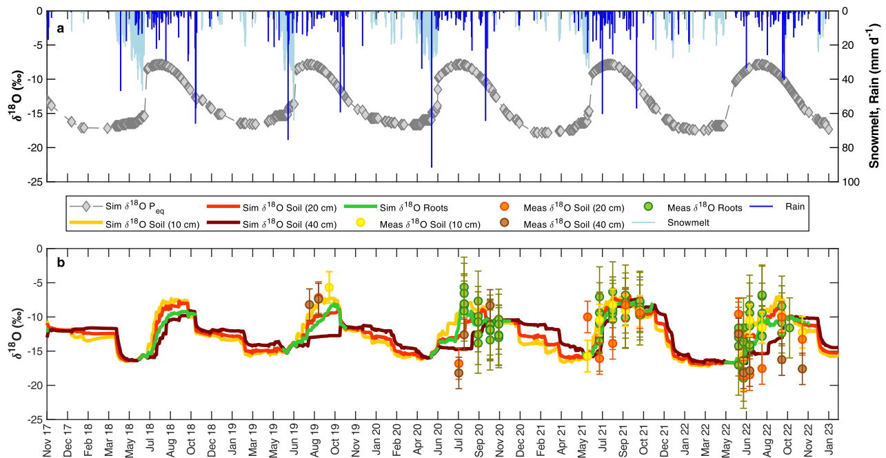
Figure 8 (a) Snowmelt, rain and isotopic composition of equivalent precipitation ( C_{Peq} ) (b) Comparison of simulated soil/plant water isotopic composition at the three observation nodes (10, 20 and 40 cm) and measured soil/plant water isotopic composition. The maximum standard deviation (SD) values reported by Millar et al. (2022) are displayed as error bars.
