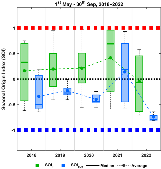
655 Figure 10 Seasonal Origin Index of transpiration (SOI T ) and bottom fluxes (SOI Bot ), simulated with HYDRUS-1D, during the growing seasons from 2018 to 2022.
