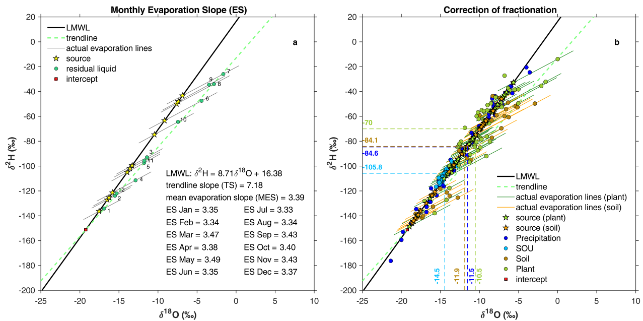
435 Figure 6 (a) Results of the monthly evaporation slopes (ES) obtained by applying the Craig and Gordon (1965) model being implemented by Benettin et al. (2018). The monthly ES have been used to reproject the fractionated water samples on the local meteoric water line (LMWL). The numbers next to the residual liquid points indicate the month (1: January; 12: December); (b) Isotopic fractionation correction for fractionated (line-conditioned excess* < 0) plant/soil water samples. Precipitation and Source (SOU) water samples have been also reported. The median isotopic composition of each reservoir is indicated by the dashed lines.
