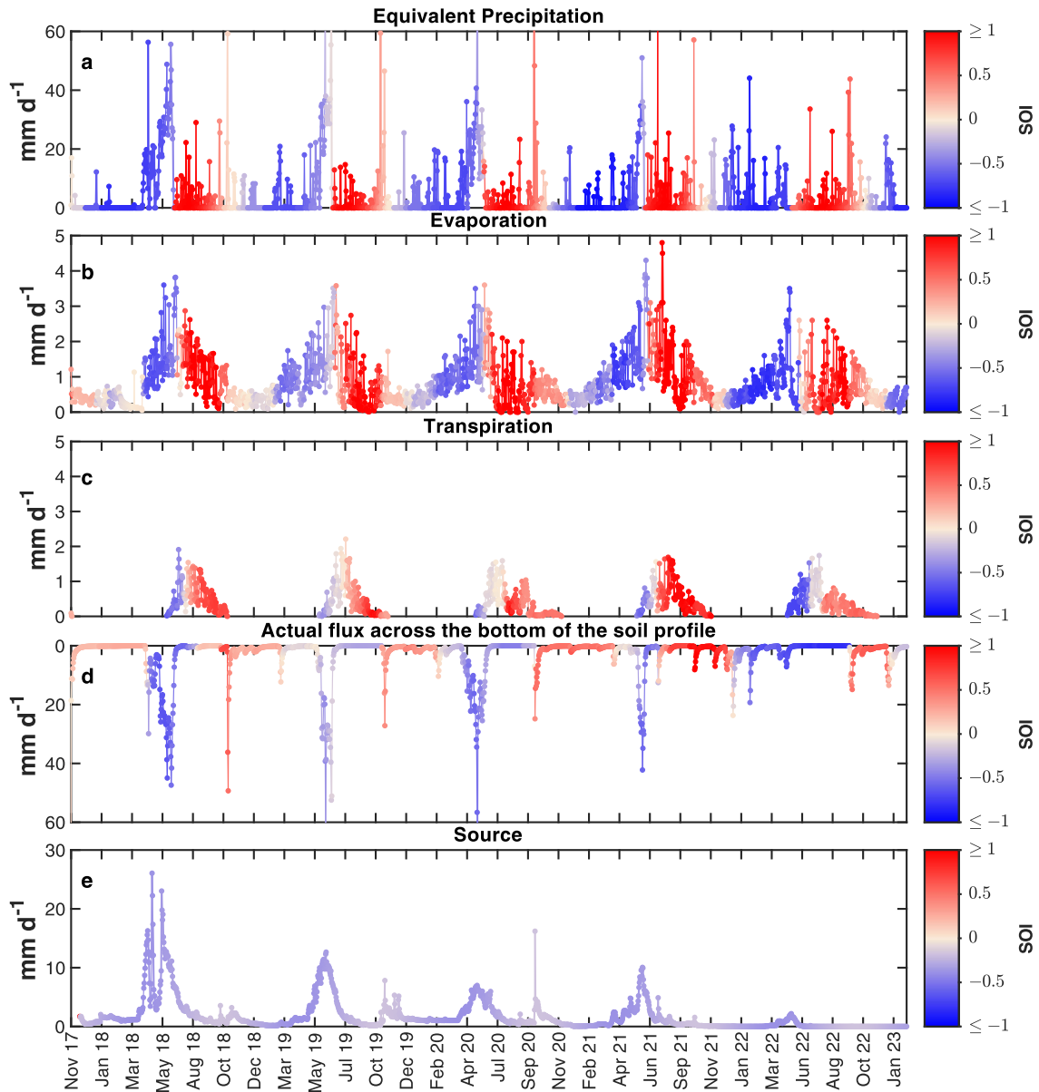
Figure 11 (a) Equivalent precipitation ( P_{eq} ) (b) Evaporation flux (c) Transpiration flux (d) Actual flux across the bottom of the soil profile. (e) Monitored spring (SOU) discharge. The red color indicates SOI > 0 (summer water is overrepresented in the flux), while the blue color indicates SOI < 0 (winter water is overrepresented in the flux). In panel (a) equivalent precipitation and the isotopic composition of equivalent precipitation ( C_{Peq} ), from which the SOI has been calculated, are obtained with the Ceperley et al. (2020) model. In panels (b), (c) and (d) the fluxes and their isotopic composition, used to retrieve the SOI, are simulated by using HYDRUS-1D. In panel (e) the SOU isotopic composition is derived from measurements: in order to have a continuous isotopic composition (and consequently continuous SOI) at all time-steps we fit a sine function on data as described in von Freyberg et al. (2018).
