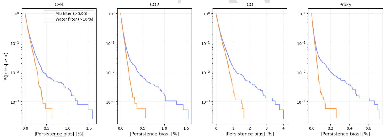
Figure 7. Each panel shows the complementary cumulative distribution function (CCDF) of the absolute persistence bias for CH 4 , CO 2 , CO, and for the CH 4 /CO 2 proxy ratio, combining data from the three Sentinel-2 scenes (the Nile Delta, California's Central Valley, and the Lusatian lignite district in Germany). Blue lines correspond to retrievals filtered with an albedo threshold of 0.05, consistent with the instrument sensitivity limit, while orange lines additionally include the water-land mask. The CCDFs represent the fraction of retrievals with an absolute bias exceeding a given threshold, allowing a direct comparison of the error-distribution tails for the two filter configurations.
