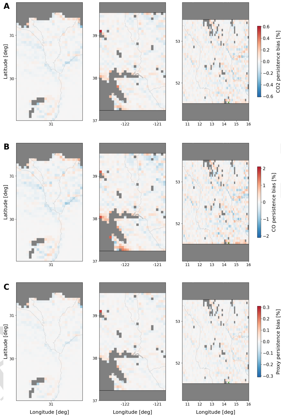
Figure B3. Spatial patterns of relative persistence bias for albedo threshold filtering equal to 0.05 and the water-land mask. Panels (A) and (B) show persistence bias maps for CO 2 and CO from the full-physics (scattering) retrievals, while plots in panel (C) presents the CH 4 /CO 2 ratio from the proxy (non-scattering) retrieval. The maps correspond, from left to right, to scenes over the Nile Delta, California's Central Valley, and the Lusatian lignite district in Germany. Coastlines, rivers, and lakes are overlaid using Cartopy's built-in Natural Earth features for contextual reference.
