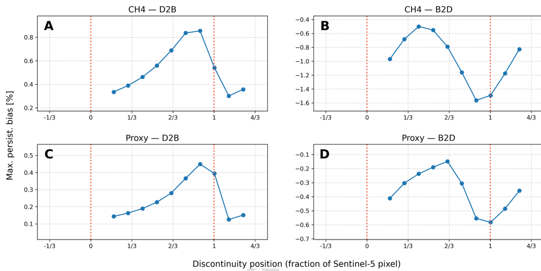
Figure B1. Panels (A) and (B) show the maximum persistence-induced \text{CH}_4 bias for the full-physics (scattering) retrieval as a function of the normalized position of the albedo discontinuity within the Sentinel-5 pixel, (0 = pixel start, 1 = pixel end). Panels (C) and (D) show the corresponding \text{CH}_4/\text{CO}_2 bias for the proxy (non-scattering) retrieval. Panels (A) and (C) refer to the dark-to-bright (D2B) albedo scenes; and panels (B) and (D), to the bright-to-dark (B2D) albedo scenes. Two dotted red lines mark the Sentinel-5 pixel boundaries.
