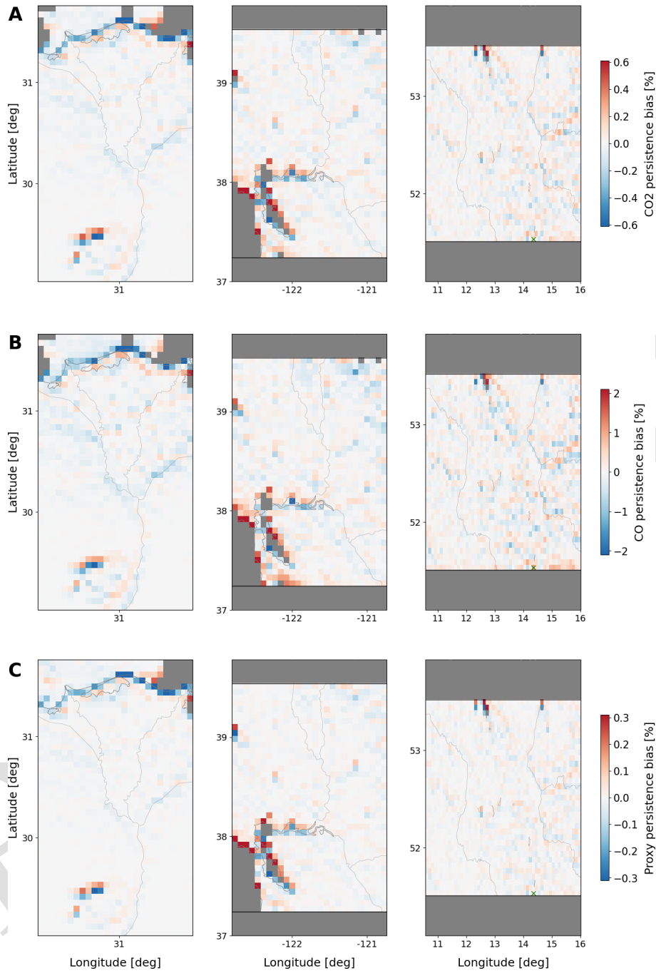
Figure B2. Spatial patterns of relative persistence bias for albedo threshold filtering equal to 0.05. Panels (A) and (B) show persistence bias maps for CO 2 and CO from the full-physics (scattering) retrievals, while plots in panel (C) presents the CH 4 /CO 2 ratio from the proxy (non-scattering) retrieval. The maps correspond, from left to right, to scenes over the Nile Delta, California's Central Valley, and the Lusatian lignite district in Germany. Coastlines, rivers, and lakes are overlaid using Cartopy's built-in Natural Earth features for contextual reference.
