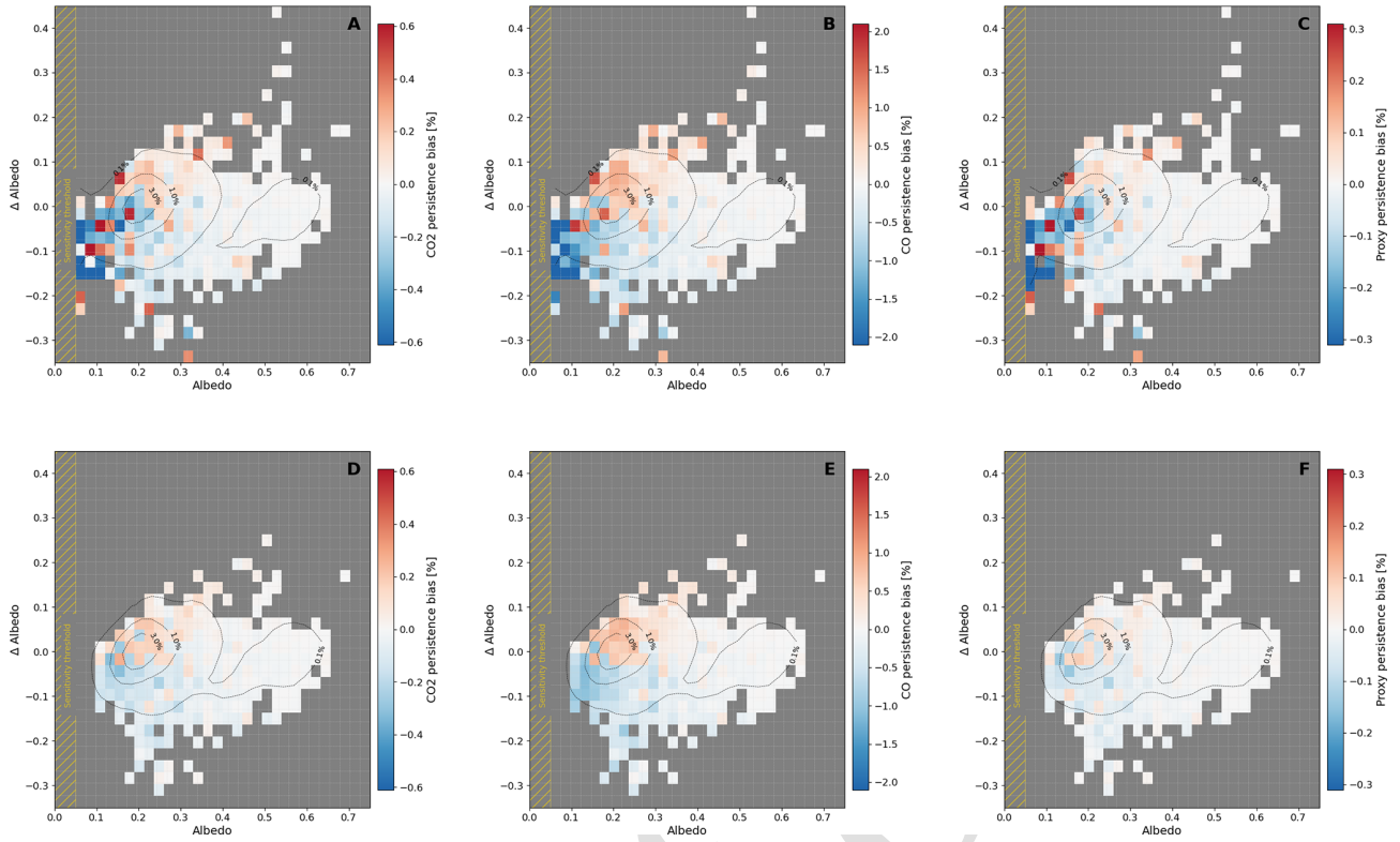
Figure B4. Panels (A)–(C) show heatmaps of the relative persistence bias with respect to SWIR-1 albedo and the corresponding \Delta SWIR-1 albedo, after applying an albedo threshold filter of 0.05 consistent with the instrument sensitivity threshold; panels (C)–(E) additionally applies a water-land mask. Panels (A)–(D) and (B)–(E) corresponds to CO 2 and CO from the full-physics retrievals respectively, while panels (C)–(F) presents the CH 4 /CO 2 ratio from the proxy retrieval. \Delta SWIR-1 albedo denotes the difference between the SWIR-1 albedo of a given pixel and that of the preceding pixel along the flight direction. Color indicates the corresponding maximum persistence bias across the three combined Sentinel-2 scenes. The gold-shaded region (albedo < 0.05) marks the sensitivity threshold of the UVNS spectrometer, where retrieval reliability is reduced. The dotted lines denote the contour plots showing the distribution density of data points within the same (Albedo, \Delta Albedo) parameter space.
