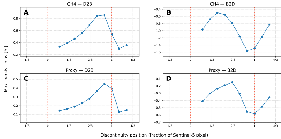
Figure A1. Panels (A) and (B) show the maximum persistence-induced \text{CH}_4 bias for the full-physics (scattering) retrieval as a function of the normalized position of the albedo discontinuity within the Sentinel-5 pixel, (0 = pixel start, 1 = pixel end). Panels (C) and (D) show the corresponding \text{CH}_4/\text{CO}_2 bias for the proxy (non-scattering) retrieval. Panels (A) and (C) refer to the dark-to-bright (D2B) albedo scenes; and panels (B) and (D), to the bright-to-dark (B2D) albedo scenes. Two dotted red lines mark the Sentinel-5 pixel boundaries.
