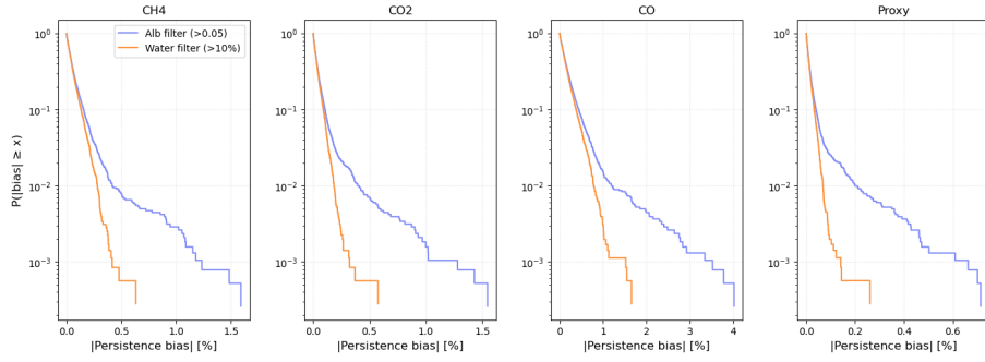
Figure 7. Each panel shows the complementary cumulative distribution function (CCDF) of the absolute persistence bias for \text{CH}_4 , \text{CO}_2 , \text{CO} , and for the \text{CH}_4/\text{CO}_2 proxy ratio, combining data from the three Sentinel-2 scenes (the Nile Delta, California’s Central Valley, and the Lusatian lignite district in Germany). Blue lines correspond to retrievals filtered with an albedo threshold of 0.05, consistent with the instrument sensitivity limit, while orange lines additionally include the water-land mask. The CCDFs represent the fraction of retrievals with an absolute bias exceeding a given threshold, allowing a direct comparison of the error-distribution tails for the two filter configurations.
