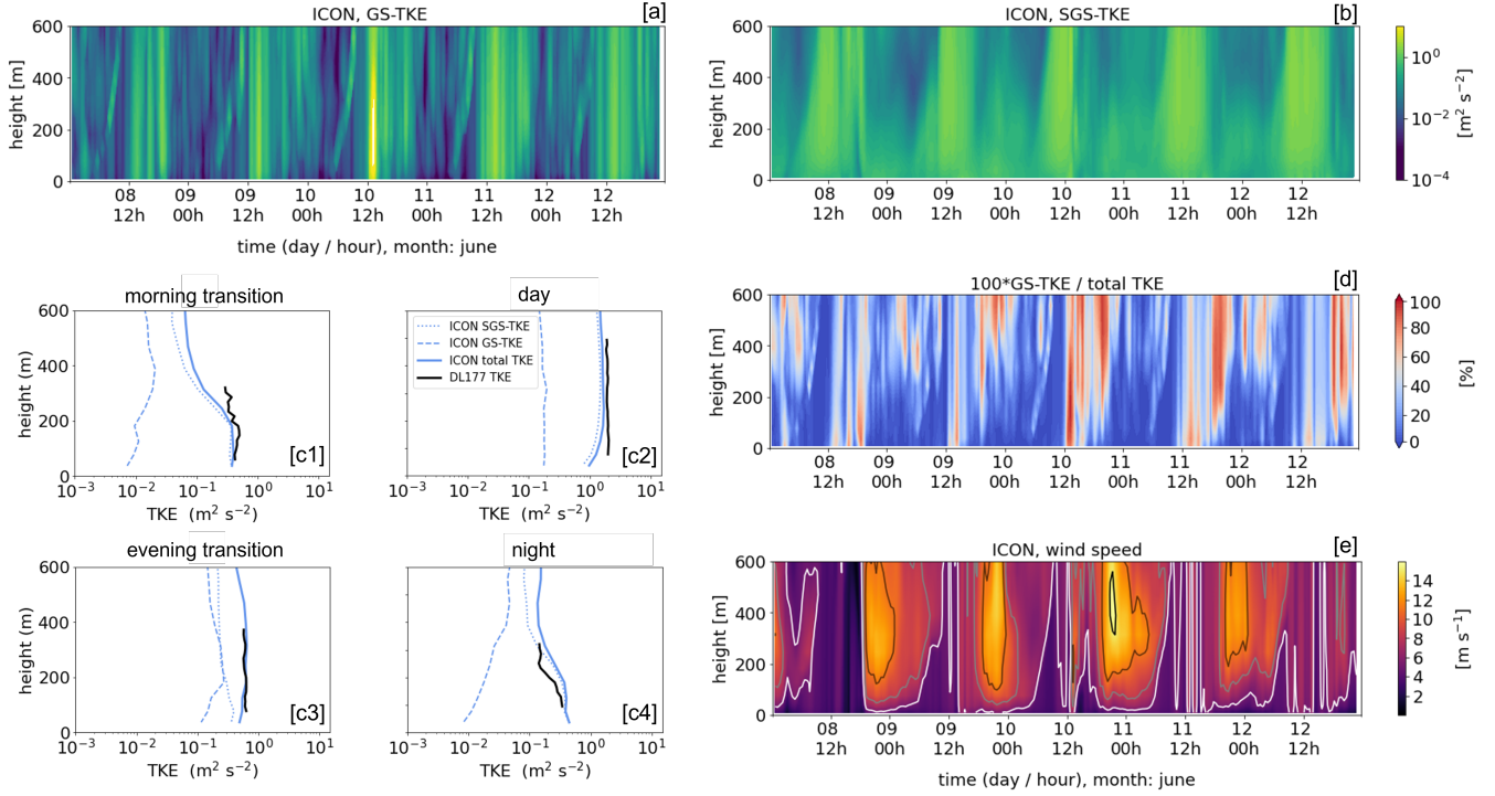
Figure 4. Time-height cross sections of [a] GS- and [b] SGS-TKE contributions, [d] fraction of GS-TKE relative to total TKE and [e] wind speed. Panels [c1] through [c4] show profiles of median (dashed) GS, (dotted) SGS and (solid) total TKE composited for the four phases of the day, as in Figure 3.
