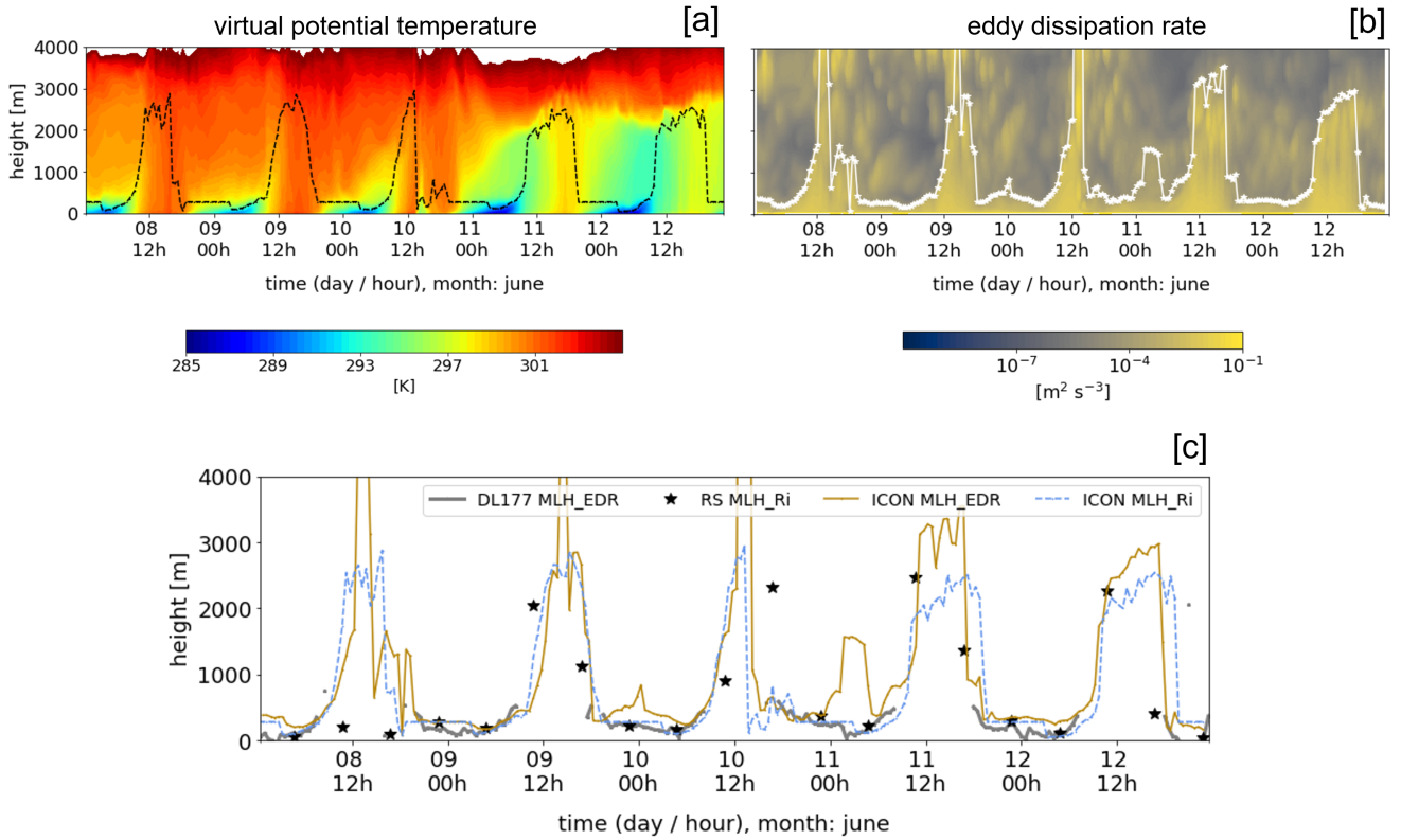
Figure 7. [a]: Time-height cross section of simulated virtual potential temperature. The black dashed contour marks the MLH determined using the (offline) MLH diagnostic based on the Ri threshold approach with Ri_{crit} = 0.2 . [b]: Simulated time-height cross section of EDR, with a white contour marking the MLH based on the threshold approach using EDR_{crit} = 10^{-4} m^2 s^{-3} (see Appendix A). [c]: Direct MLH comparison from the different threshold approaches against observations based on both radiosonde soundings and Doppler Lidar derived EDR profiles.
