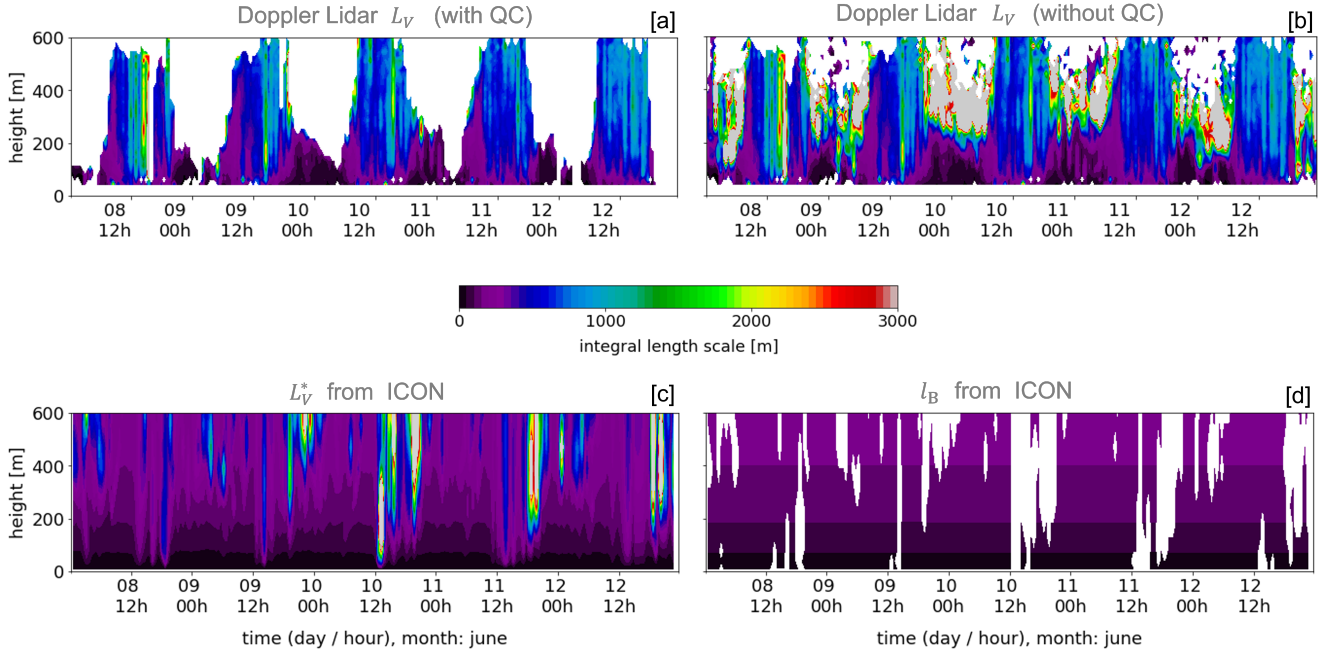
Figure 5. [a]: Time-height cross sections for Doppler Lidar derived integral length scales L_V with masked area where the data fail quality control (QC), i.e. where the application of Eq. (1) is no longer justified, [b]: same as in [a] but without QC, [c]: time-height cross sections for ICON derived L_V^* calculated based on Eq. (8), [d]: Blackadar’s integral length scale l_B , which is assumed to be constant in Turbdiff, with white areas in the panel indicating where the model conditions do not satisfy g < 1 in Eq. (8).
