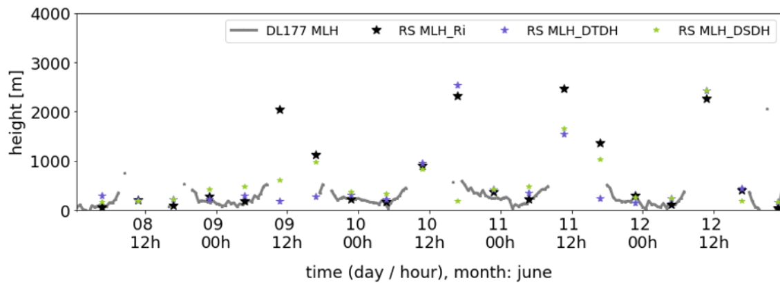
Figure A1. [a]: Comparison of the mixing layer height (MLH) obtained from Doppler lidar (DL) and radiosonde soundings (RS) for the 5-day time period 8-12 June 2023 at the MOL-RAO site. DL177 MLH denotes the MLH obtained from DL based EDR profiles. RS_MLH_DTDH, RS_MLH_DSDH and RS_MLH_Ri denote different RS based MLHs according to specific definitions (e.g. existence of temperature inversion, zones with significant wind shear or the height at which the Richardson number exceeds a critical level) applied to RS based temperature and wind profiles.
