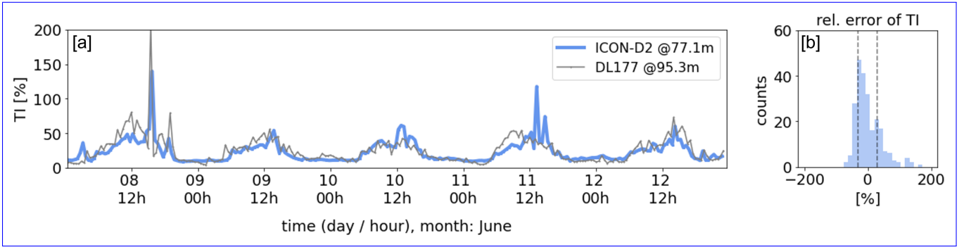
Figure 8. [a]: Comparison of diagnosed model TI between ICON simulations at 77 m height with DL-derived TI at 95 m height at the Falkenberg observation site. [b]: Histogram of relative errors for total TI between ICON and Doppler lidar. Vertical dashed lines indicate a relative error of \pm 30\% .
