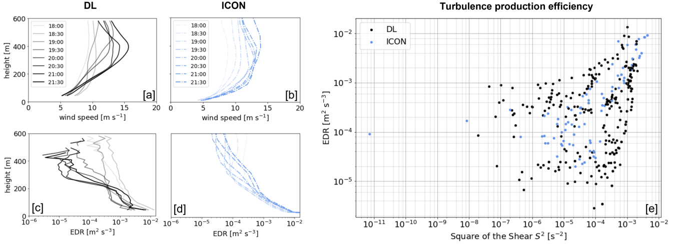
Figure 6. [a]-[d]: A comparison of the temporal evolution of 30-minute averaged DL- and ICON-based profiles for wind speed and eddy dissipation rate (EDR) during the transition period from afternoon to evening to the early nocturnal period on June 9th. [e]: Relationship between vertical wind shear ( S^2 ) and (EDR) to assess turbulence production efficiency.
