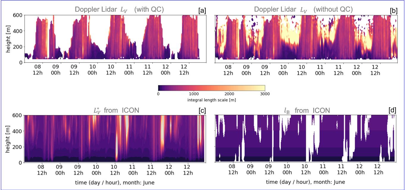
Figure 5. [a]: Time-height cross sections for Doppler Lidar derived integral length scales L_V with masked area where the data fail quality control (QC), i.e. where the application of Eq. (1) is no longer justified, [b]: same as in [a] but without QC, [c]: time-height cross sections for ICON derived L_V^* calculated based on Eq. (8), [d]: Blackadar’s integral length scale l_B , which is assumed to be constant in Turbdiff, with white areas in the panel indicating where the model conditions do not satisfy g < 1 in Eq. (8).
