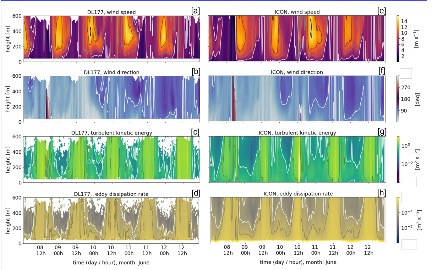
Figure 1. Comparison of time-height cross sections for [a],[e]: wind speed, [b],[f]: wind direction, [c],[g]: turbulent kinetic energy (TKE) and [d],[h]: eddy dissipation rate (EDR) from (left) DL retrieval ([a]-[d]) and from (right) ICON simulations ([e]-[h]). Each DL-derived dataset was subject to a specific quality flag (QC), resulting in differences in data availability.
