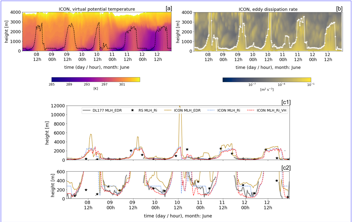
Figure 7. [a]: Time-height cross section of simulated virtual potential temperature. The black dashed contour marks the MLH determined using the (offline) MLH diagnostic based on the Ri threshold approach with Ri_{\text{crit}} = 0.2 . [b]: Simulated time-height cross section of EDR, with a white contour marking the MLH based on the threshold approach using EDR_{\text{crit}} = 10^{-4} \text{m}^2 \text{s}^{-3} (see Appendix A). [c1]: Direct MLH comparison from the different threshold approaches against observations based on both radiosonde soundings and Doppler Lidar derived EDR profiles. [c2]: Same as in [c1] but zoomed into a vertical range of 0–600 m to better resolve nighttime variations.
