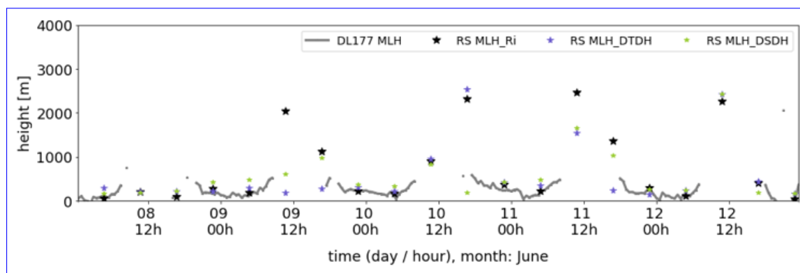
Figure A1. [a]: Comparison of the mixing layer height (MLH) obtained from Doppler lidar (DL) and radiosonde soundings (RS) for the 5-day time period 8-12 June 2023 at the MOL-RAO site. DL177 MLH denotes the MLH obtained from DL based EDR profiles. RS_MLH_DTDH, RS_MLH_DSDH and RS_MLH_Ri denote different RS based MLHs according to specific definitions (e.g. existence of temperature inversion, zones with significant wind shear or the height at which the Richardson number exceeds a critical level) applied to RS based temperature and wind profiles.
