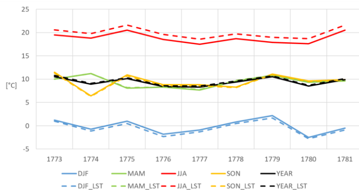
Fig. 5. Year-to-year changes in seasonal and annual mean air temperature in Wrocław, 1773–81
