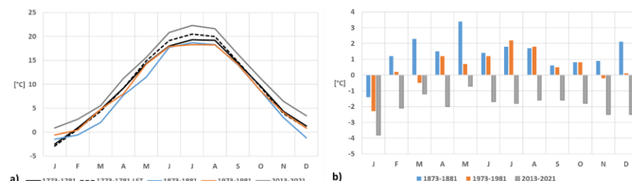
Fig. 9. Comparison of the annual cycle of air temperature in Wrocław (SW Poland) in historical time (1773–81) against other more modern periods (a) and their differences (b) Key: Means for the compared periods were calculated based on data from three measurement times: 1873–81 (unknown hours), 1973–81 and 2013–21 (6, 12, and 21). Air temperatures from the modern period were subtracted from those from the historical period.
