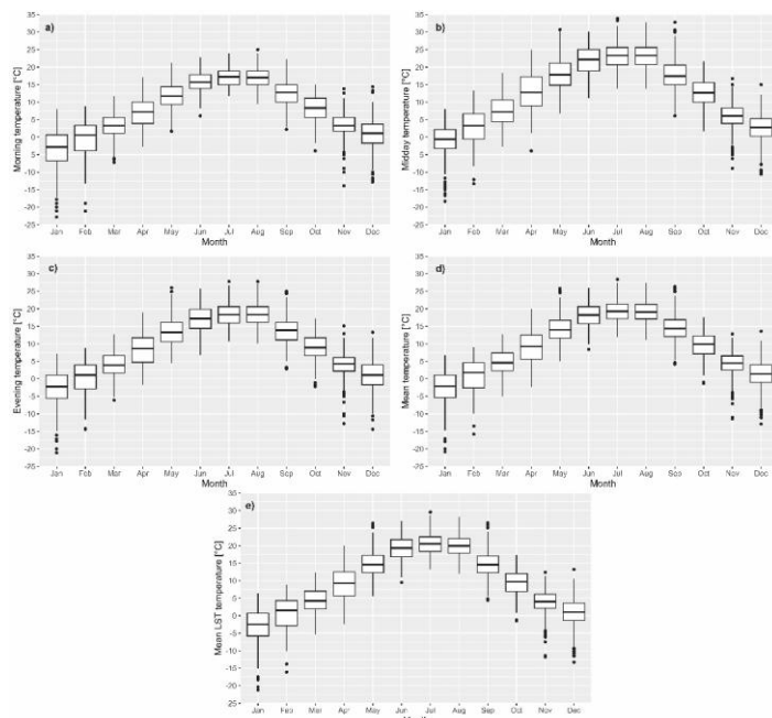
Fig. 7. Boxplots of the distribution of: morning (a) upper-left, midday (b) upper-right, evening (c) air temperatures; lower-left) and mean daily: (uncorrected (d), and corrected using LST (e)) lower-right) air temperatures in Wrocław, 1773–81
