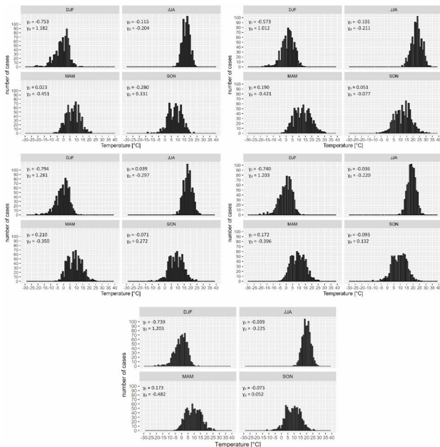
Fig. 8. Frequency of seasonal (DJF, MAM, etc.) occurrence of: morning (a)-upper left, midday (b)-upper right, evening (c)-lower left, air temperature, and mean daily: (uncorrected (d)), and corrected using LST (e)-lower right air temperature in Wrocław from 1773 to 1781 stratified according to 1-degree intervals
