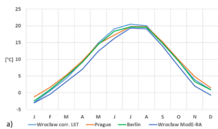
Fig. 10. Comparison of the annual cycle of air temperature in Wroclaw in historical time (1773–81) against other available series in central Europe (a), and their differences in relation to the 1961–90 reference period (b). Key: Air temperatures from the reference period were subtracted from those of the historical period.
