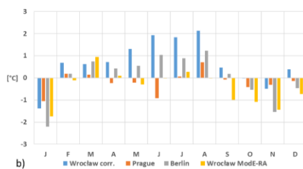
Fig. 10. Comparison of the annual cycle of air temperature in Wroclaw in historical time (1773–81) against other available series in central Europe (a), and their differences in relation to the 1961–90 reference period (b). Key: Air temperatures from the reference period were subtracted from those of the historical period.
