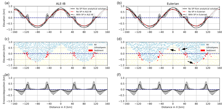
Figure 4. Topography, erosion and deposition of the relaxation model in ALE-IB and Eulerian scheme at Time = 0.15 Ma, the dark blue line indicates the sea level . (a) and (b) Topography: The grey zone indicates shaded area shows the range between the maximum and minimum topography values produced by the model with surface processes (SP), while the black line represents the average topography. (c) and (d) Material field: Distribution-distribution of material properties within the model, the arrows indicate particle fluctuations. (e) and (f) Erosion and deposition: quantification of surface processes over time, showing accumulated erosion and deposition. The grey shaded area denotes the range between maximum and minimum values, and the black line represents the average value.
