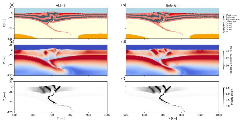
Figure 10. (a), (b) Material, (c), (d) viscosity, and (e), (f) accumulated plastic strain of the coupling model in ALE-IB and Eulerian scheme ( CM2-CC-CM2 and EMECC-CME ) at Time = 4.5 Ma.
