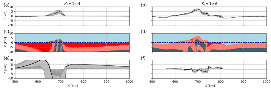
Figure 16. Topography, erosion and deposition of the coupling model in ALE-IB scheme ( CM1-CC-CM1 and CM3-CC-CM3 ) at Time = 4.5 Ma. the dark blue line indicates the sea level. (a) and (b) Topography: The the grey zone indicates shaded area shows the range between the maximum and minimum topography values produced by, while the model with surface processes black line represents the average topography. (c) and (d) Material field: Distribution-distribution of material properties within the model, the arrows indicate particle fluctuations. (e) and (f) Erosion and deposition: quantification of surface processes over time, showing accumulated erosion and deposition. The grey shaded area denotes the range between maximum and minimum values, and the black line represents the average value.
