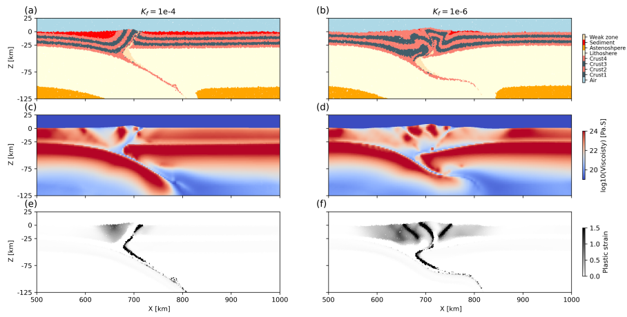
Figure 15. (a), (b) Material, (c), (d) viscosity, and (e), (f) accumulated plastic strain of the coupling model in ALE-IB scheme with different fluvial erosion parameters ( \text{CM1-CC-CM1} and \text{CM3-CC-CM3} ) at Time = 4.5 Ma.
