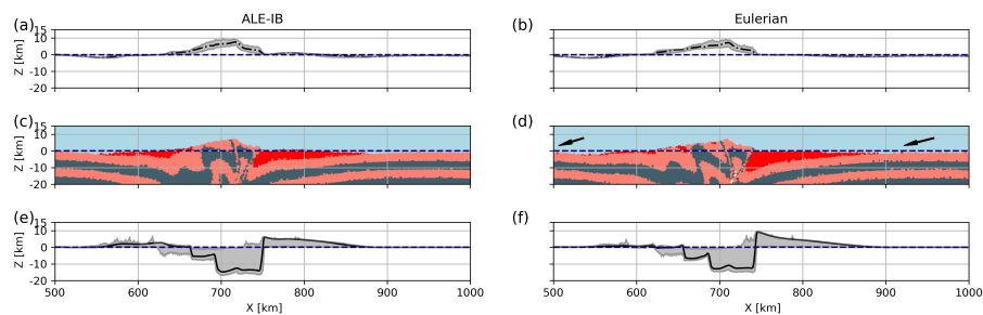
Figure 11. Topography, erosion and deposition at Time = 4.5 Ma of the coupling model in ALE-IB and Eulerian scheme (CM2-CC-CM2 and CMECC-CME), the dark blue line indicates the sea level. (a) and (b) Topography: The grey zone indicates shaded area shows the range between the maximum and minimum topography values produced by the model with surface processes, while the black line represents the average topography. (c) and (d) Material field: Distribution distribution of material properties within the model, the arrows indicate particle fluctuations. (e) and (f) Erosion and deposition: quantification of surface processes over time, showing accumulated erosion and deposition. The grey shaded area denotes the range between maximum and minimum values, and the black line represents the average value.
