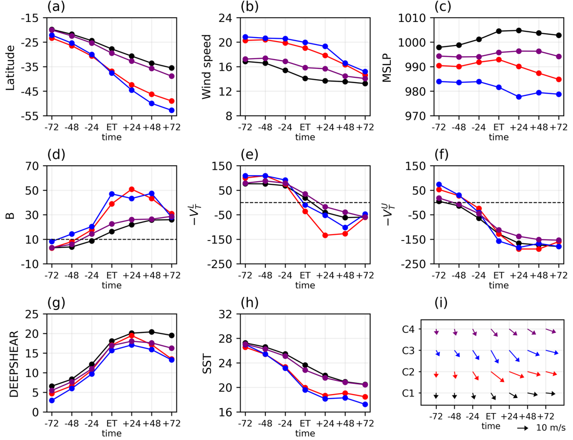
Figure 10. Evolution of (a) latitude, (b) wind speed (in m/s), (c) central pressure (MSLP, in hPa), (d) B , (e) -V_T^L , (f) -V_T^U , (g) vertical wind shear (DEEPSHEAR, in m/s), (h) SST (in ^{\circ}\text{C} ), and (i) cyclone speed (in m/s) and direction from 72 hours before to 72 hours after ET for individual clusters. Dashed horizontal lines in (d-f) mark the thresholds for ET in the CPS framework. Clusters 1, 2, 3, and 4 are marked by various colors (black, red, blue, and purple). The bottom (right) aligns with south (east) in (g).
