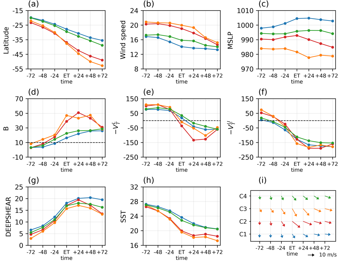
Figure 10. Evolution of (a) latitude, (b) wind speed (in m/s), (c) central pressure (MSLP, in hPa), (d) B , (e) -V_T^L , (f) -V_T^U , (g) vertical wind shear (DEEPSHEAR, in m/s), (h) SST (in °C), and (i) cyclone speed (in m/s) and direction from 72 hours before to 72 hours after ET for individual clusters. Dashed horizontal lines in (d-f) mark the thresholds for ET in the CPS framework. Clusters 1, 2, 3, and 4 are marked by various colors (blue, red, orange, and green). The bottom (right) aligns with south (east) in (g).
