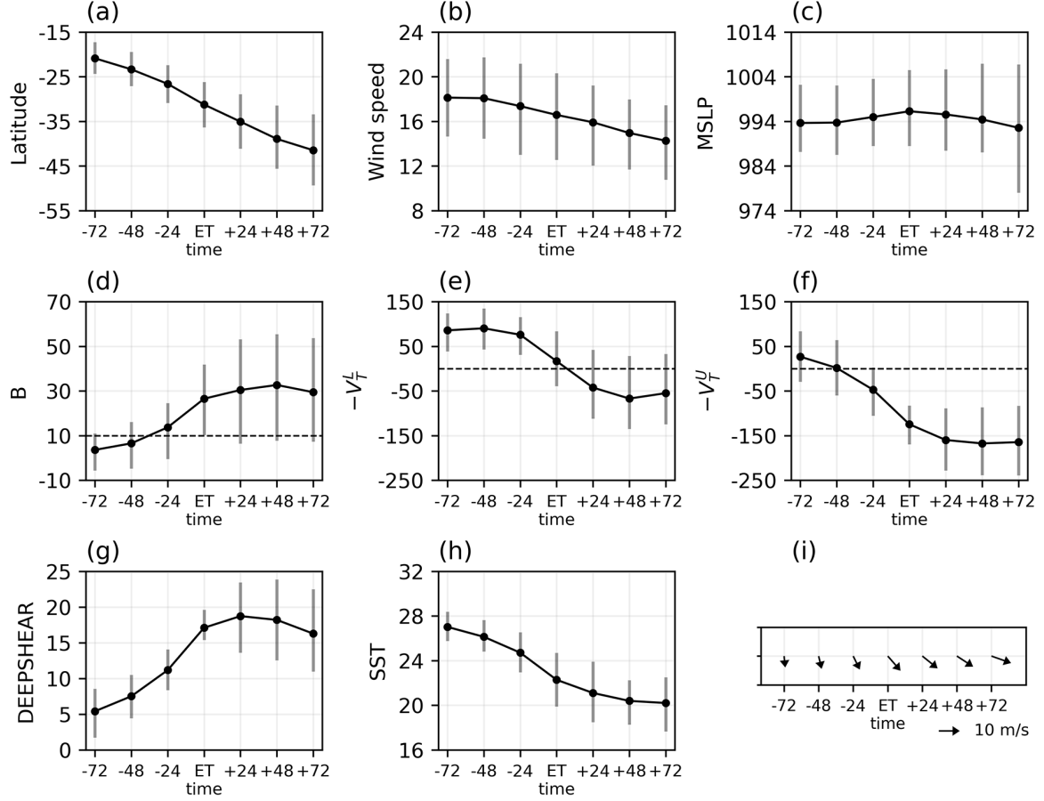
Figure 5. Evolution of (a) latitude, (b) wind speed (in m/s), (c) central pressure (MSLP, in hPa), (d) B , (e) -V_T^L , (f) -V_T^U , (g) vertical wind shear (DEEPSHEAR, in m/s), (h) SST (in ^{\circ}\text{C} ), and (i) cyclone speed (in m/s) and direction from 72 hours before to 72 hours after ET. Dots denote the mean, and whiskers mark the 25th and 75th percentiles. Dashed horizontal lines in (d-f) mark the thresholds for ET definition in the CPS framework. The bottom (right) aligns with south (east) in (i).
