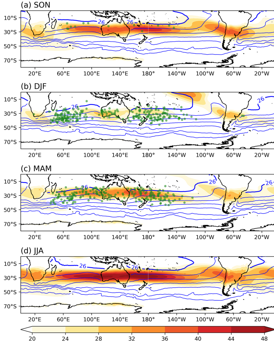
Figure 4. Seasonal climatologies of vertical wind shear (in m/s; shaded as per the colourbar) and SST (in °C; blue contours every 4 °C starting from 2 °C) for (a) September-October-November (SON), (b) December-January-February (DJF), (c) March-April-May (MAM), and (d) June-July-August (JJA) over the Southern Hemisphere. Green dots mark the positions of ET. A thick blue line highlights the 26 °C contour. The seasonal climatologies are based on the period 1979-2021.
