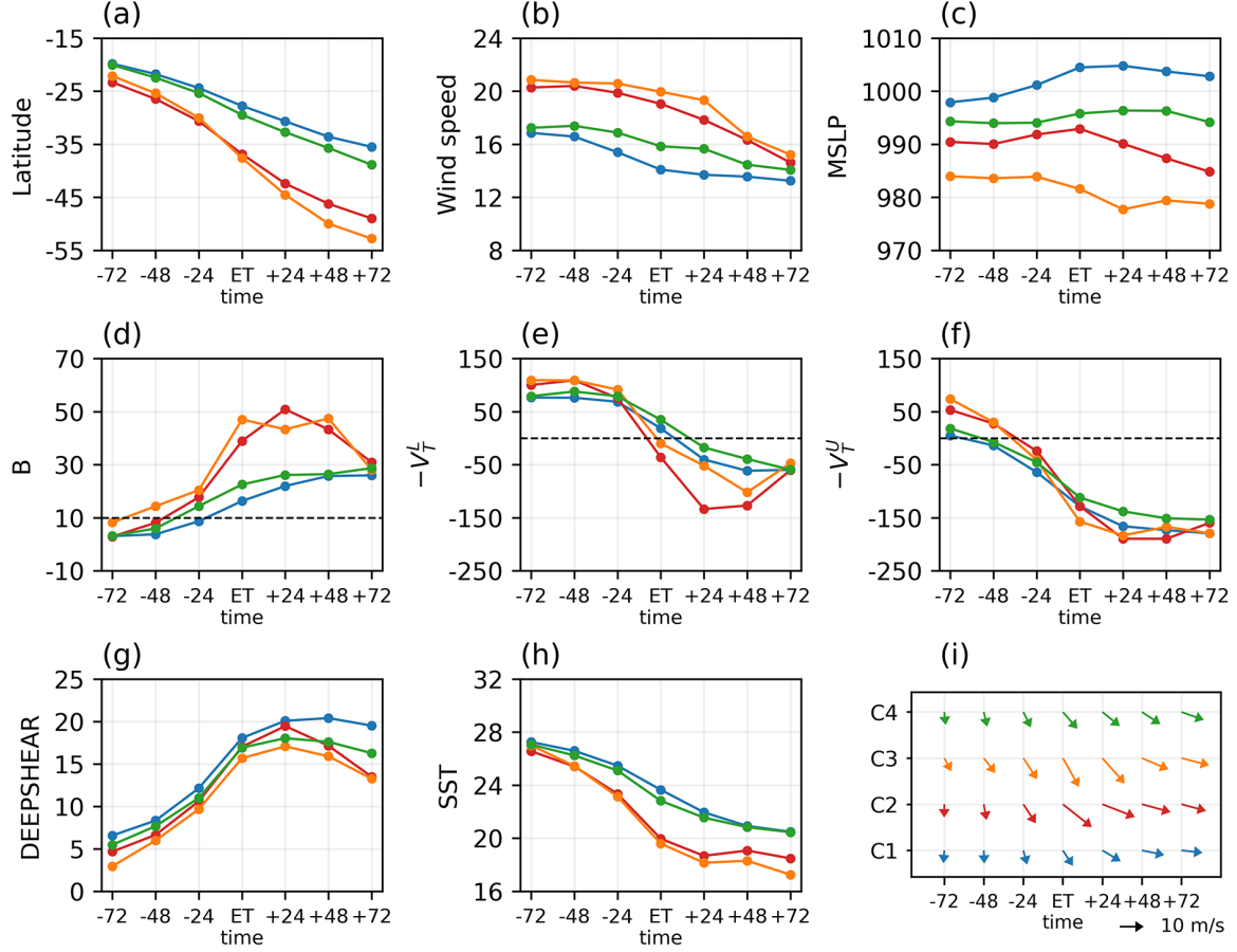
Figure 10. Evolution of mean (a) latitude, (b) wind speed (in m/s), (c) central pressure (MSLP, in hPa), (d) B , (e) -V_T^L , (f) -V_T^U , (g) vertical wind shear (DEEPSHEAR, in m/s) , (h) SST (in ^{\circ}\text{C} ), and (i) cyclone speed (in m/s) and direction from 72 hours before to 72 hours after ET for individual clusters. Dashed horizontal lines in (d-f) mark the thresholds for ET in the CPS framework. Clusters 1, 2, 3, and 4 are marked by various colors (blue, red, orange, and green). The bottom (right) aligns with south (east) in (g).
