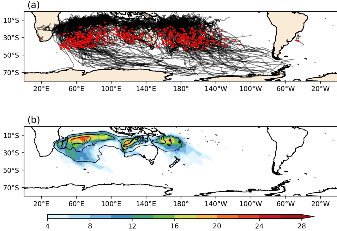
Figure 2. (a) TC tracks that undergo ET, with red dots marking the position of ET. (b) The densities of all TC tracks (black contour every 20) and those that undergo ET (shaded as per the colourbar). Track density is represented by the total number of tracks passing each 1.25^\circ \times 1.25^\circ grid cell in the period 1979-2021. All track densities are smoothed by a Gaussian filter with \sigma = 2 .
