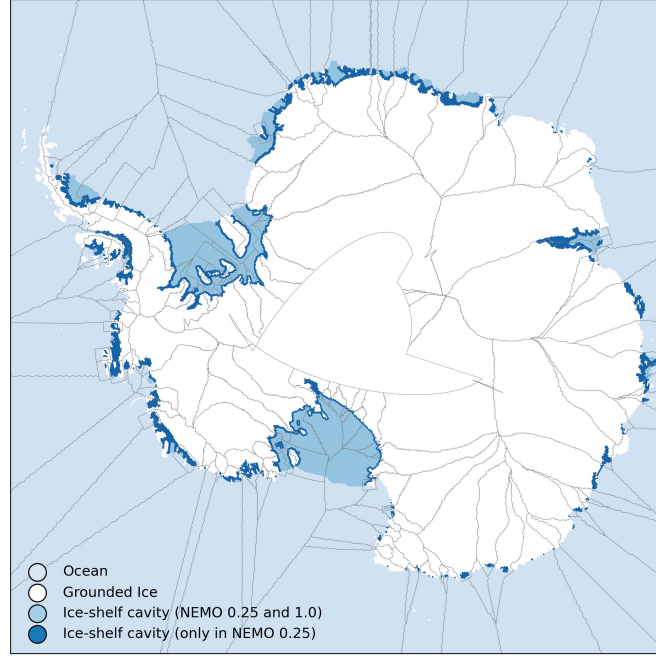
Figure A3. The outlines of the 155 partial ice-shelf basins, based on the locations of the individual outlet glaciers and ice streams (?), are shown by the light grey lines.
