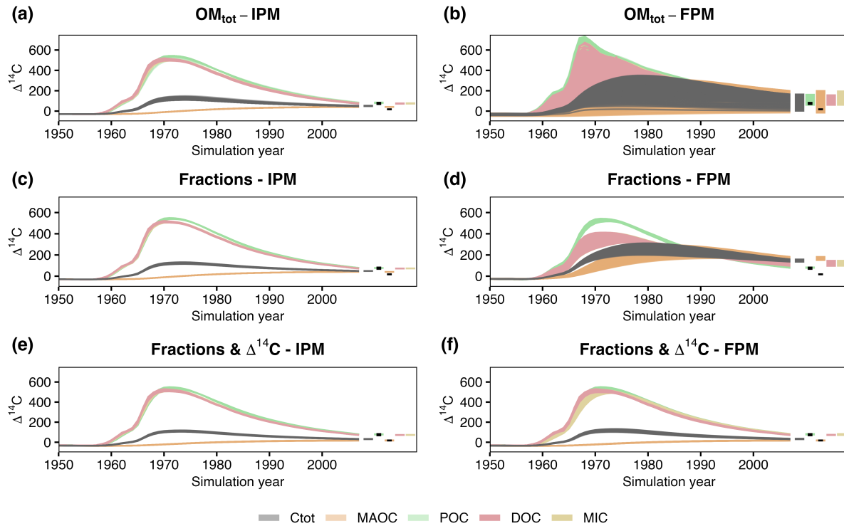
Figure 6. Simulated \Delta^{14}\text{C} values of the model pools shown in Fig. 5, for the period of the 'bomb spike' in atmospheric \Delta^{14}\text{CO}_2 that occurred in the second half of the 20 th century. The bars on the right of each graph show the range in simulated \Delta^{14}\text{C} in the year 2007, together with the average \pm standard deviation of assumed measurements for the POC and MAOC pools in black.
