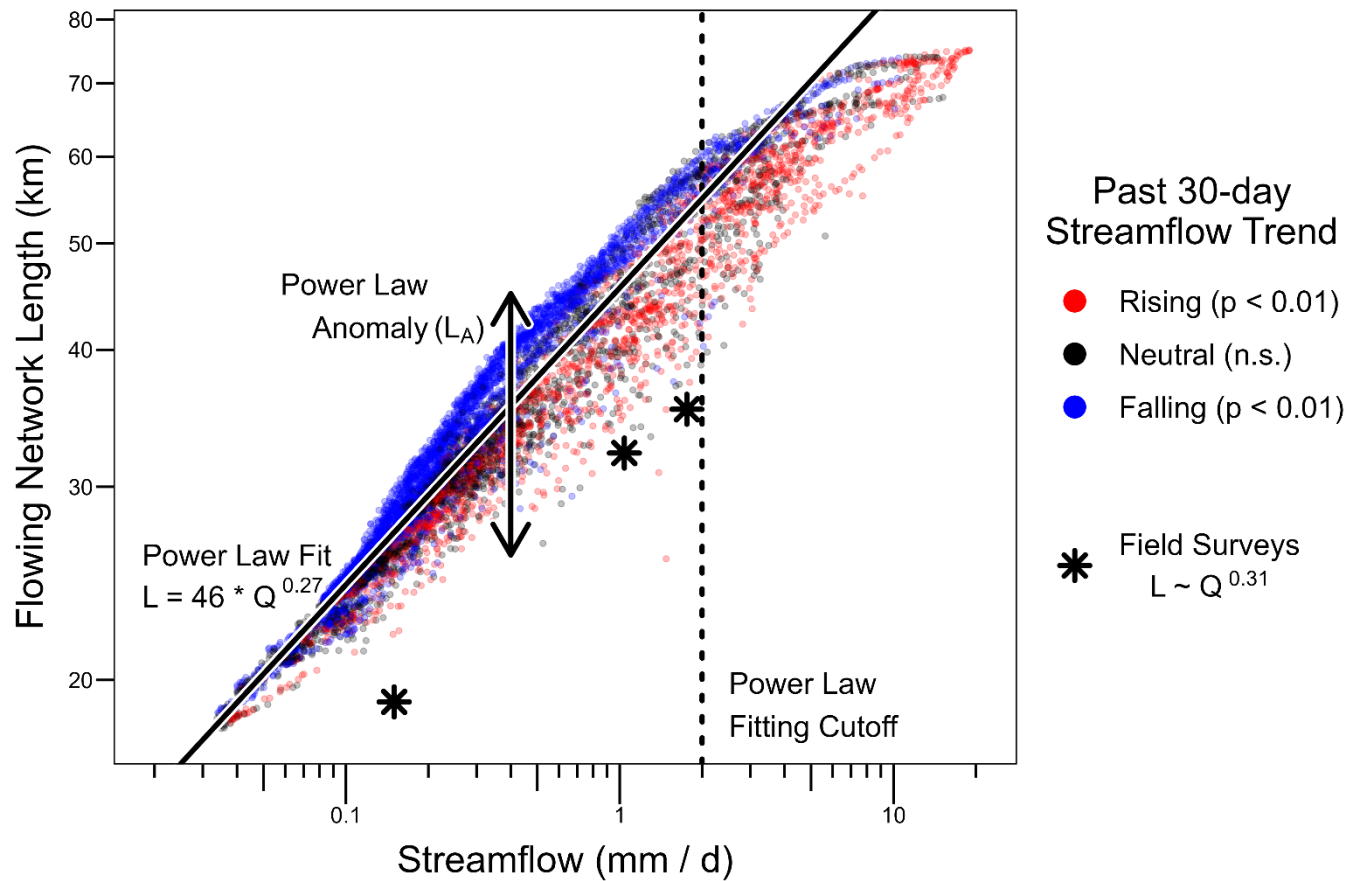
640 Figure 4. Logarithmically scaled scatterplot between simulated daily streamflow ( Q ) and flowing stream network length ( L ). Each point represents one day over water years 2001-2024. Red (blue) colors indicate a rising (falling) streamflow trend over the 30 days prior to each point (Mann-Kendall test). Three field surveys are shown, and a fourth survey falls below the lower vertical axis limit ( Q = 0.24 mm/d, L = 15.4 km), which Godsey and Kirchner (2014) identify as a potential outlier because of practical difficulties in following the entire network on the first field survey.
