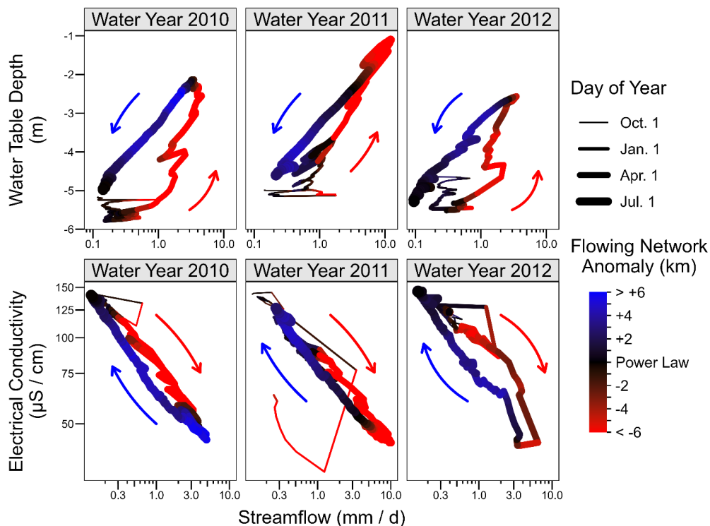
Figure 56. Hysteresis relationships in three example years, showing (top panels) simulated water table depth and simulated streamflow, (bottom panels) measured stream electrical conductivity, reflecting total dissolved ion content (correlated to groundwater age, Rademacher et al. 2001), and measured streamflow. Each line traces a path beginning on October 1 st of a given water year, and line width is scaled proportionally to the day of year. Color indicates whether the simulated flowing stream network is larger (blue) or smaller (red) than predicted by a power law relationship with streamflow on a given day.
