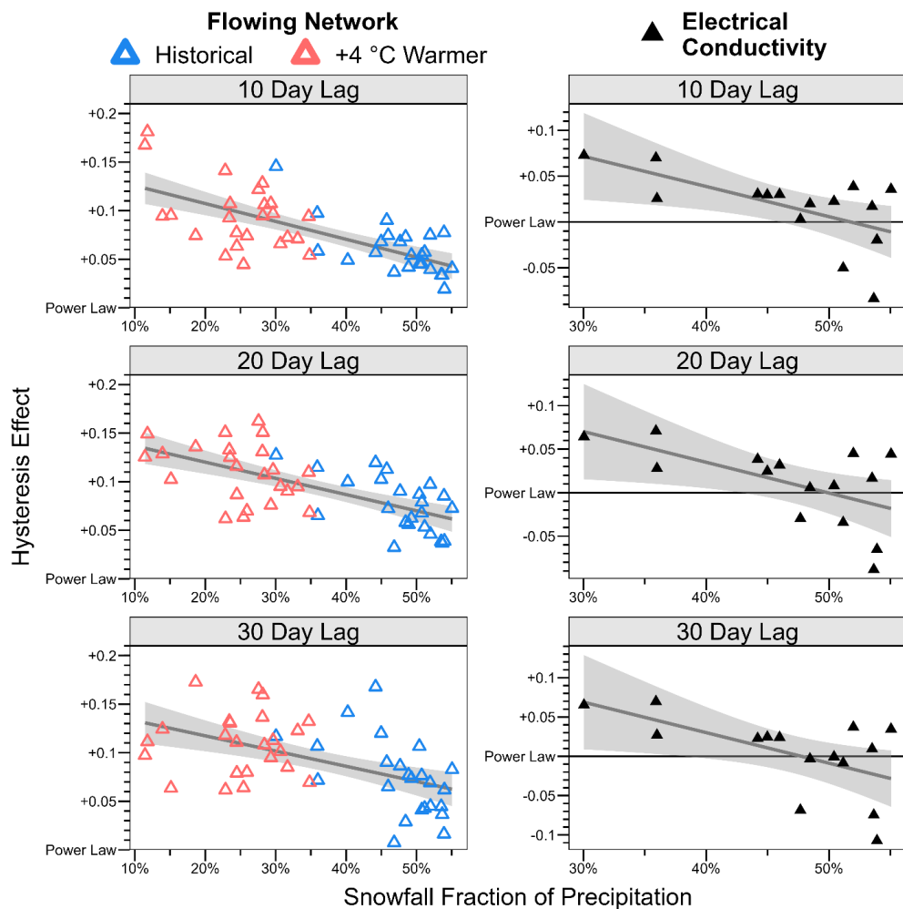
Figure 89. A stronger flowing network hysteresis effect (difference in simulated autocorrelation relative to a power law assumption) is associated with a smaller fraction of precipitation falling as snow. A similar relationship is detected in timeseries of measured stream electrical conductivity, which is related to groundwater age. Shaded gray regions show the 95% confidence range for the best-fit linear trendline.
