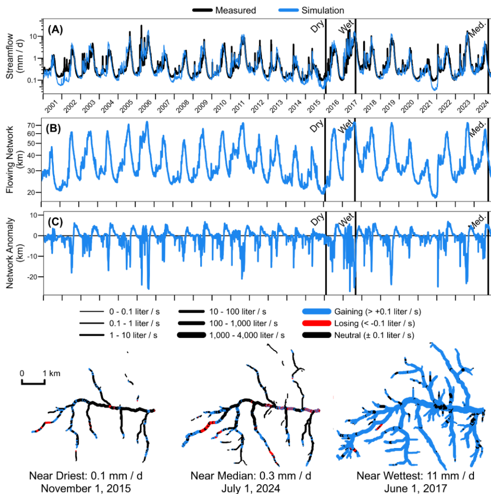
Figure 42. Daily timeseries over the 24-year study period: (A) measured and modeled streamflow, Q , (B) modeled flowing stream network length, L , and (C) modeled anomaly in L relative to a power law scaling assumption. Example maps of the modeled flowing network show the spatial arrangement and variable Q (line width) of flowing stream reaches at 1 st , 50 th , and 99 th -percentile flows. Stream reaches that are gaining Q from GW are illustrated in blue, reaches that are recharging Q back to GW (losing) are illustrated in red, and reaches with an approximately neutral balance of inflows and outflows are illustrated in black.
