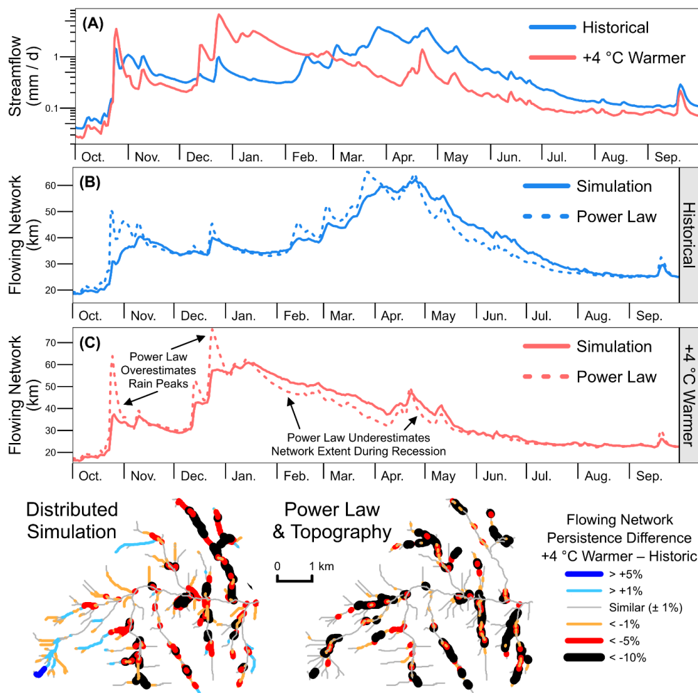
Figure 78. Example timeseries for one year of the simulation under historical or +4 °C warmer climate scenarios, showing (A) simulated streamflow and (B-C) flowing network length simulated directly or estimated from a power law in the historical (B) or warmer (C) scenarios. Maps show the change in streamflow persistence (fraction of flowing days across 24 years) between warmer and historical model simulations (left) or inferred from the combination of a power law and static topographic flow routing assumptions (right).
