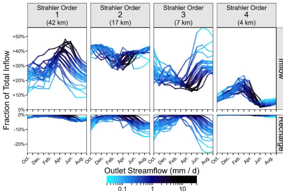
Figure 23. Seasonal variation in the inflow and groundwater recharge from stream reaches organized according to Strahler order (Fig. S7, S6 in the Supplement). Each line represents a single water year, and all values are aggregated to the monthly median. Lines are colored according to the log-scaled outlet streamflow, and the vertical axes are scaled in proportion to the total network inflow. First-order streams contribute relatively more inflow during the snowmelt period, and third-order streams contribute disproportionately in the late summer. Most recharge from streams to groundwater occurs in second- and third-order streams. Relative seasonal network dynamics are partially decoupled from the absolute magnitude of outlet streamflow.
