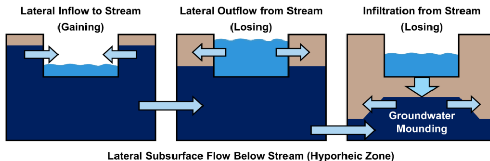
Figure 1. Cross-sectional view of the new dynamic surface-groundwater coupling mechanism in DHSVM. Lateral and vertical exchanges between the channel and groundwater are determined by the hydraulic gradient between the channel water level and the local water table. Channels can switch between gaining or losing water to the subsurface over both time and space.
