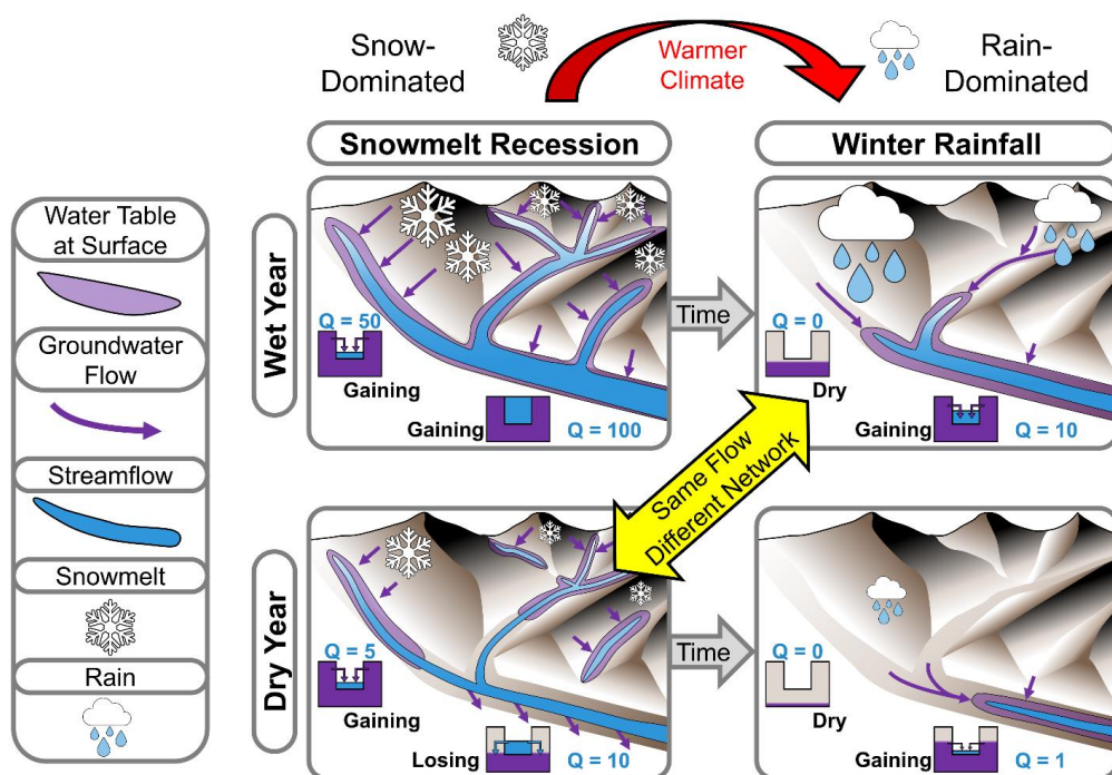
Figure 910. Revised conceptual model of stream-groundwater interactions in a mountain catchment, illustrating the emergence of stream network hysteresis caused by transient groundwater flow between hillslopes and riparian zones. Contrast with conceptual model illustrated in Fig. 7 of Godsey and Kirchner (2014), which assumes equilibrium groundwater flow. Channel cross-sections show how this conceptual model is simulated at the grid scale (cf. schematic in Fig. S41). Antecedent groundwater priming from snowmelt and rain activates a relatively large flowing stream network during the seasonal recession period, but rainfall during periods with a low antecedent water table can cause a rapid increase in streamflow even though the flowing network remains small. In a warmer climate, winter rainfall becomes more dominant than spring snowmelt, altering the spatial configuration of streamflow generation and flowing network connectivity. Note: figure is not to scale (streams and hyporheic zones are enlarged for visual clarity); overall stream network is on the order of kilometer-scale.
