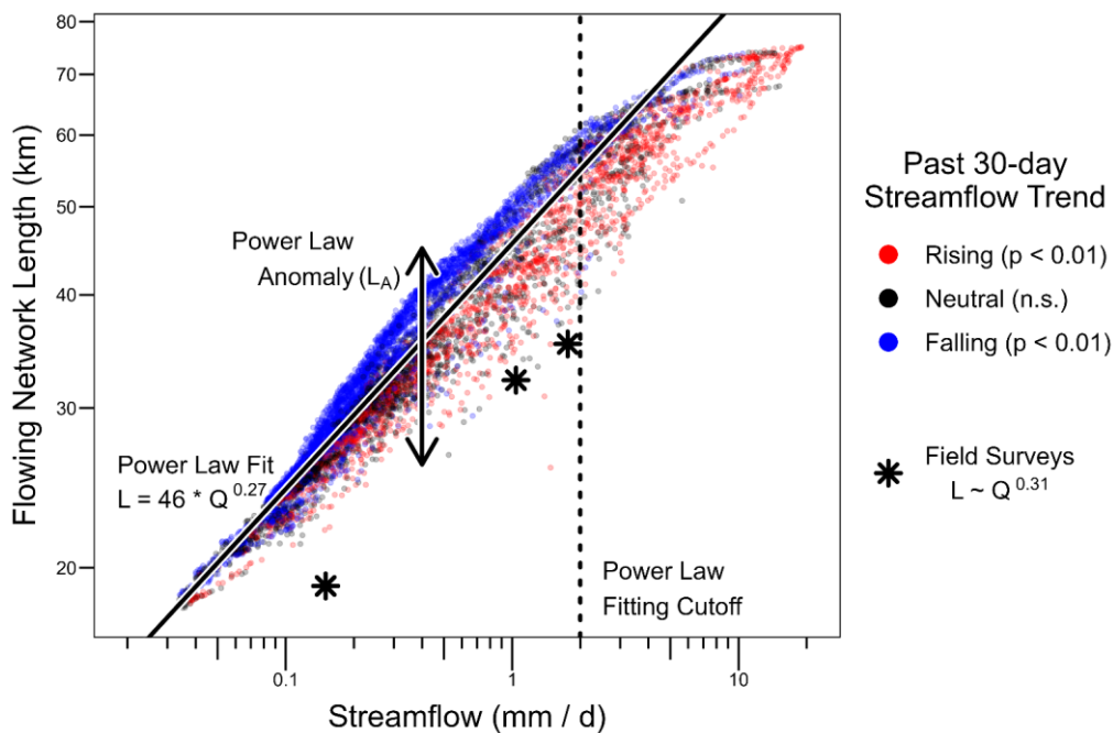
Figure 34. Logarithmically scaled scatterplot between simulated daily streamflow ( Q ) and flowing stream network length ( L ). Each point represents one day over water years 2001–2024. Red (blue) colors indicate a rising (falling) streamflow trend over the 30 days prior to each point; (Mann–Kendall test). Three field surveys are shown, and a fourth survey falls below the lower vertical axis limit ( Q = 0.24 mm/d, L = 15.4 km), which Godsey and Kirchner (2014) identify as a potential outlier because of practical difficulties in following the entire network on the first field survey.
