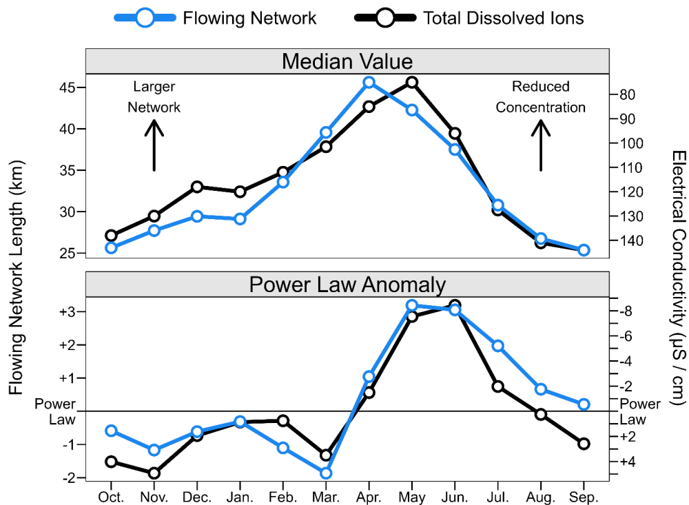
Figure 67. Comparison of monthly median simulated stream network dynamics with measured stream water electrical conductivity (EC), a proxy for total dissolved ion concentrations. Note that the vertical axis is reversed for EC (positive down) to highlight the similar shape of the seasonal signals. The seasonality of anomalously large flowing networks matches the seasonality of anomalously low EC, indicative of a greater fractional contribution from relatively fast, chemically dilute subsurface flowpaths during the snowmelt season.
