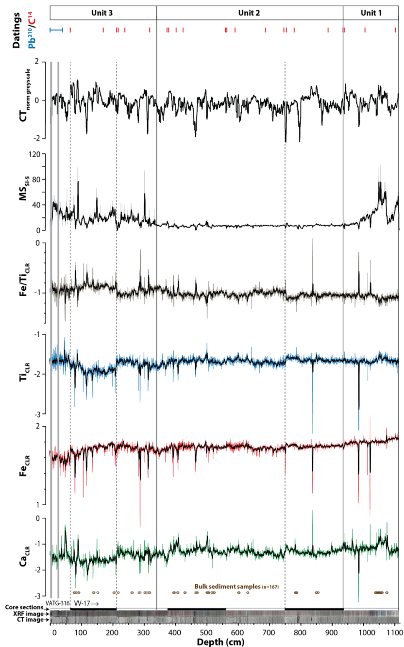
320 Figure 5: Results and overview of selected core analyses from Vangsvatnet. CT- and XRF image, log-transformed XRF data (Ca, Fe, Ti, Fe/Ti), Magnetic susceptibility (MS) measurements, and normalised CT-grey scale values. The subdivisions (Units 1–3) are based on the variations in MS. Brown open circles indicate where bulk sediments (n=167) were retrieved. Red lines indicate radiocarbon samples (n=22). The upper part of VATG-316 was sampled for Pb 210 dating (blue line) (n=44). Dotted lines indicate 325 areas of rapid shifts in XRF-values, while the grey shaded areas in the uppermost section are missing data related to cracks/air in the core.
