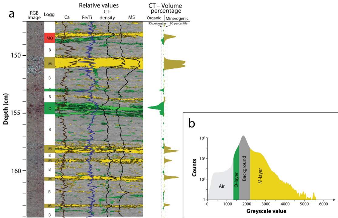
340 Figure 7: (a) RGB- and CT-image with relative values of XRF-parameters (Ca and Fe/Ti) and CT-density and MS. A threshold analysis has been performed on the CT data, identifying the volume percentages of minerogenic (yellow) and organic (green) content related to the sediment layers in the image (B-, M-, and O- and MO-layers). (b) Histogram of CT-data showing the thresholding of the layers in Fig 7a.
