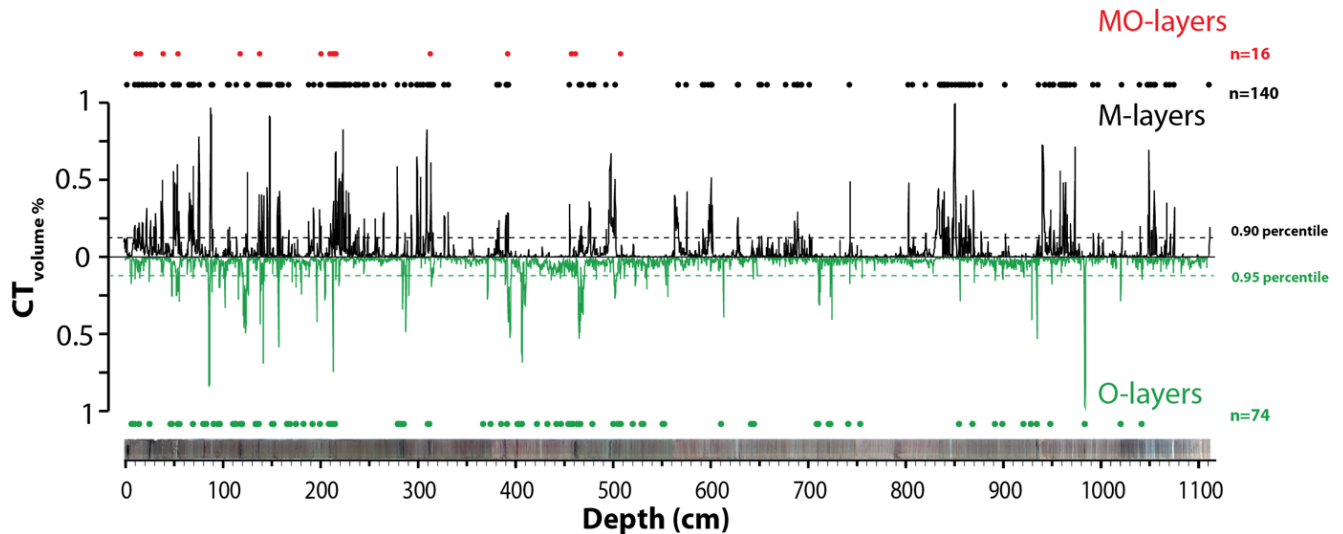
345 Figure 8: Volume percent measurement of thresholded CT-data for the composite core showing organic content (green) and minerogenic content (black). The 90th percentile for the minerogenic content and the 95th percentile for the organic content is used to separate event layers from background sedimentation. MO layers (red) are events in which both organic and minerogenic material are present.
