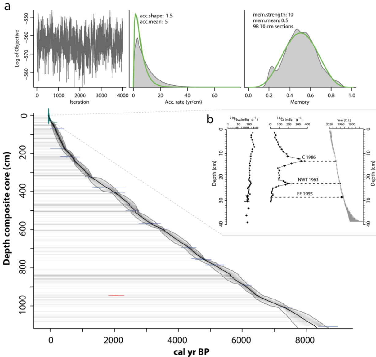
365 Figure 9: (a) Age–depth relationship for the composite core obtained with the package Bacon (Blaauw and Christen, 2011) in R based on ^{14}\text{C} -dating and the short-lived radionuclides ( ^{137}\text{Cs} and ^{210}\text{Pb} ). The black line shows the best age–depth estimates with a 95% confidence interval in grey shading. Red coloured date is left out of the model due to a likely disturbance/redeposition (see text). All the recorded event layers are treated as instantaneous events and are marked as slumps in the model (grey horizontal lines). (b) 370 A piecewise CRS model produced with the R-based Serac package (Bruel and Sabatier, 2020) based on the short-lived radionuclides from the upper 39.5 cm of VATG316 ( ^{137}\text{Cs} and ^{210}\text{Pb} ).
