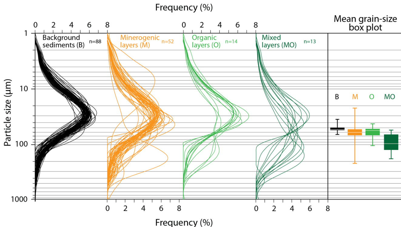
325 Figure 6: Grain-size distribution and mean grain-size box plot of the different sediment layers (B-, M-, O- and MO) from the composite core. Most of the samples are poorly sorted with unimodal distribution. A few samples in M- (n=3) and MO-layers (n=1) are poorly sorted bimodal.
