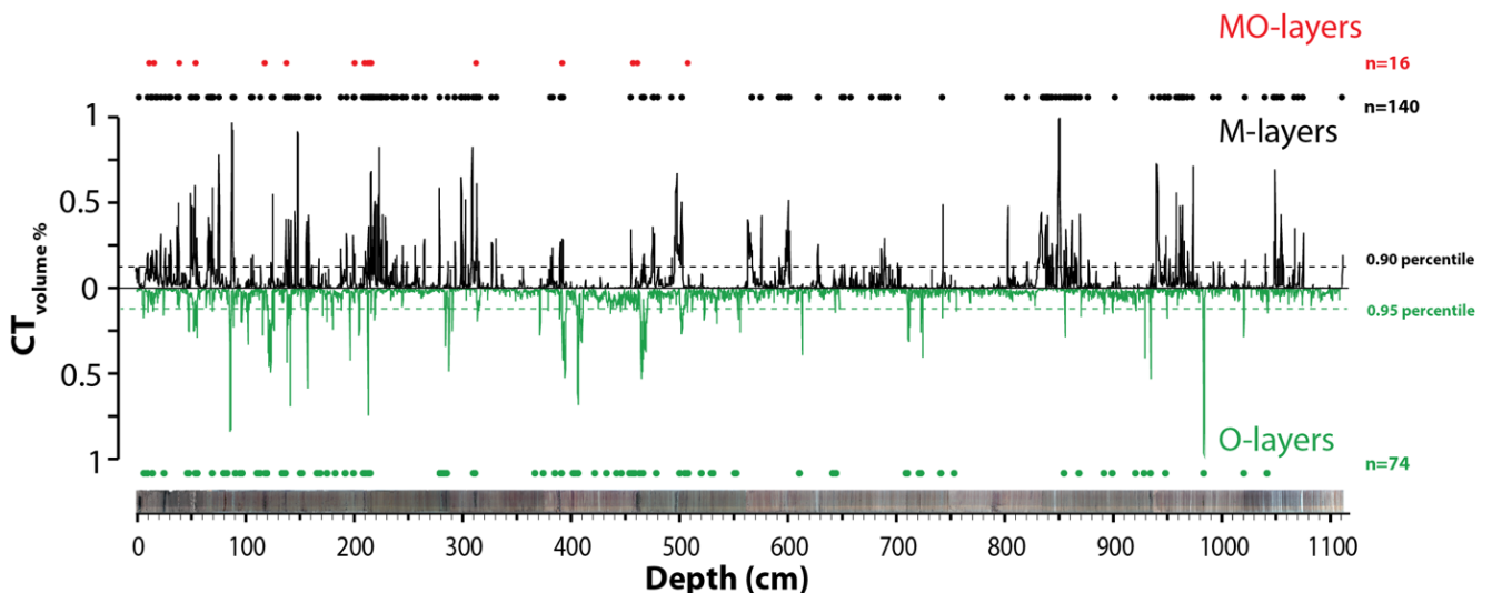
340 Figure 8: Volume percent measurement of thresholded CT-data for the composite core showing organic content (green) and minerogenic content (black). The 90th percentile for the minerogenic content and the 95th percentile for the organic content is used to separate event layers from background sedimentation. MO layers (red) are events in which both organic and minerogenic material are present.
