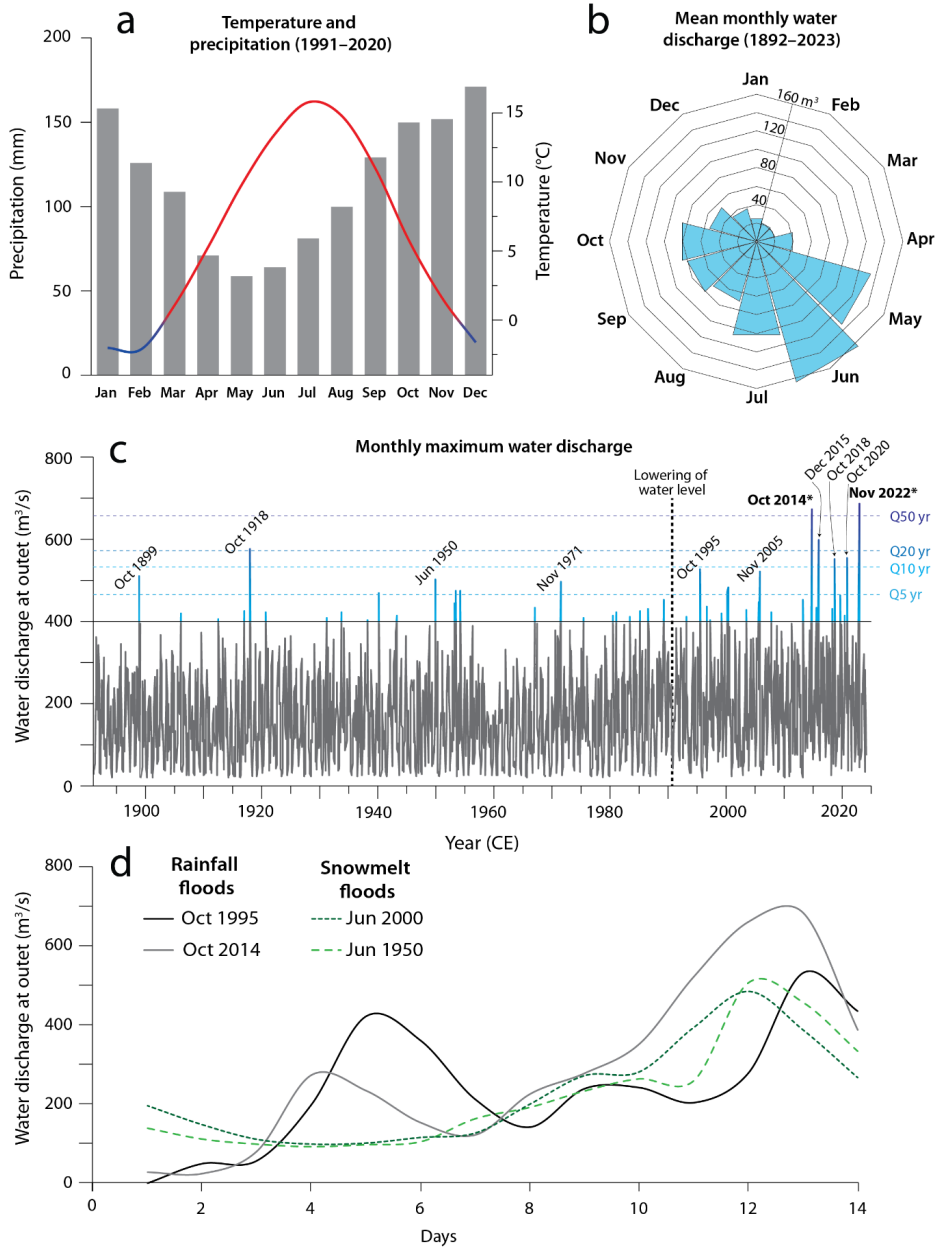
Figure 3: (a) Temperature and precipitation at Voss for the 1991-2020 CE climate normal and mean (b) and maximum (c) monthly water discharge at Bulken (1892-2023 CE) (DNMI, 2024; NVE, 2024). The floods in Oct 2014 and Nov 2022 (both in bold) have the highest discharge values since the start of the measurements in 1892 CE. (d) 14 days of discharge data before four different floods.
