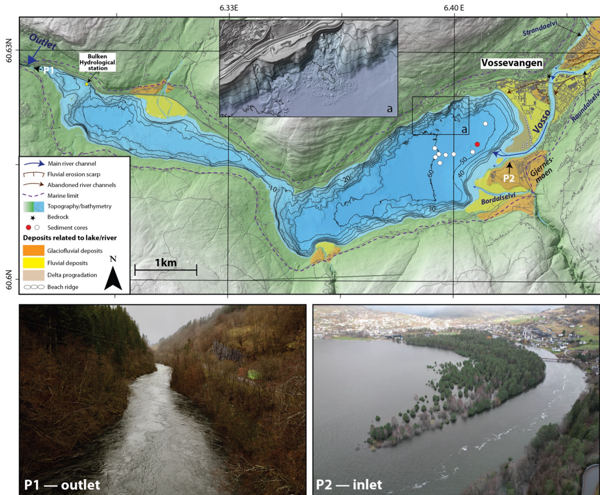
140 Figure 2: Lake Vangsvatnet (7.6 km 2 , 44 m a.s.l.) has two main basins. Sediment cores for the Hordafloam project were retrieved in 145 the eastern basin close to the main inlet (the Vosso R -river) (photo P2) and shown as white and red circles in the map. The red circle shows the coring location used in this study. Fluvial and glaciofluvial sediments dominate along the rivers, especially near the inlets. The marine limit at Voss is around 94 m a.s.l (purple line dotted line). The outlet in the west is a narrow gorge (photo P1), obstructing water drainage during flooding. The photos (P1 and P2) show the inlet and the outlet during the November 2024 flooding, reaching a discharge of 580 m 3 /s at Bulken. Inset Figure (a) shows two examples of large landslides along the northern slope, as seen in the bathymetric data.
