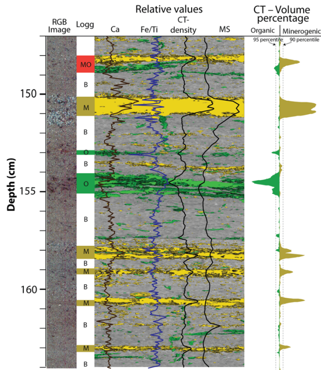
335 Figure 7: RGB- and CT-image with relative values of XRF-parameters (Ca and Fe/Ti), and CT-density and MS . A threshold analysis has been performed on the CT data, identifying the volume percentages of minerogenic (yellow) and organic (green) content related to the sediment layers in the image (B-, M-, and O- and MO-layers ).
