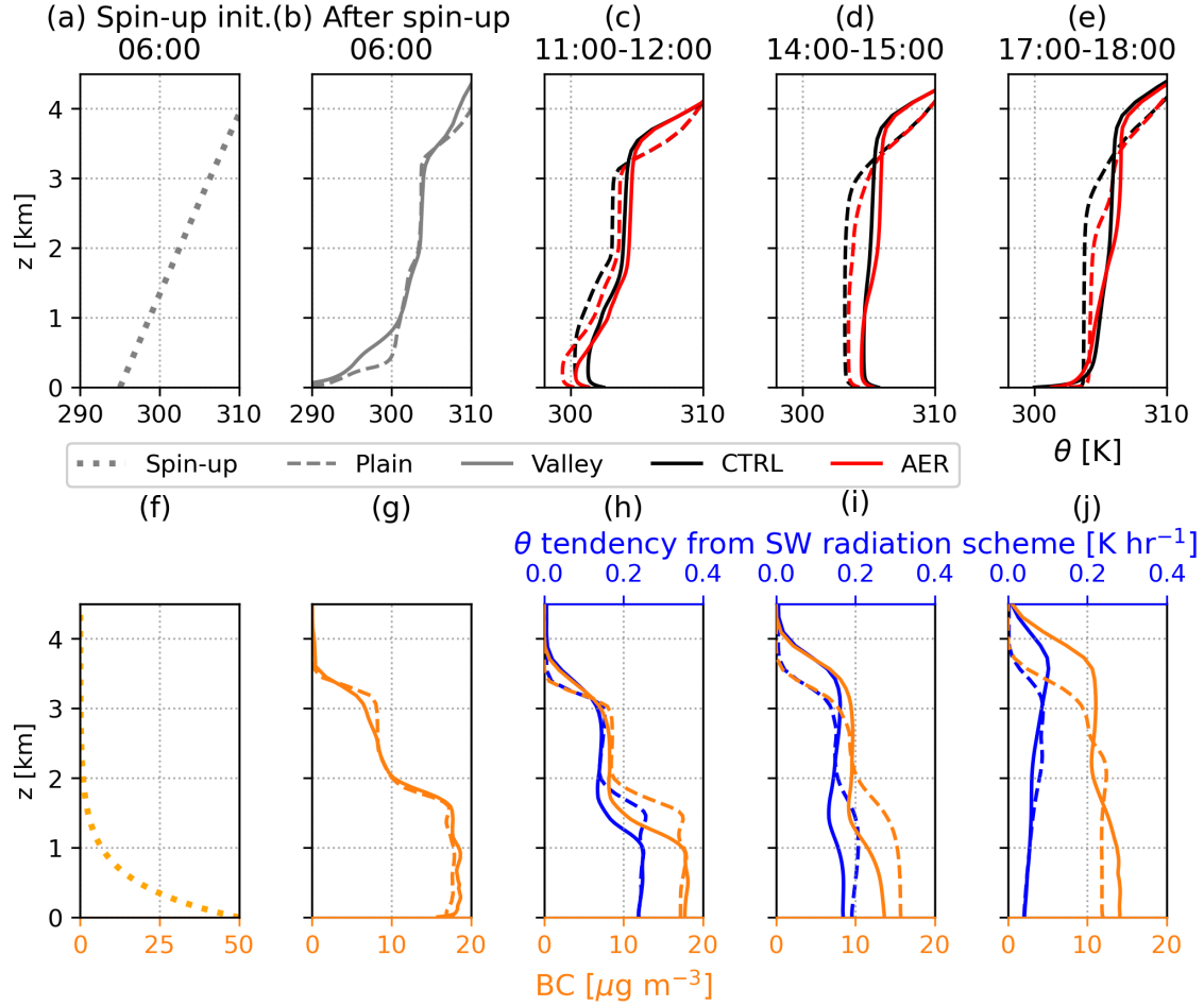
Figure 2. Top row: Vertical profile of (a-d) potential temperature in both cases AER and CTRL (e-h) Bottom row: Vertical profile of black carbon and potential temperature tendency from the shortwave radiation scheme in case AER. The marked time is (a,f) Horizontally uniform initial conditions of the end-time spin-up run. (b,g) Initial condition of the hourly-average cases AER and CTRL after the 24-hour spin-up. Hourly averages between (c,h) 11:00-12:00 (d,i) 14:00-15:00 and (e,j) 17:00-18:00. Solid lines show the vertical profile averaged over the valley centre line ( y > 0 km, x = 0 km) and dashed lines above the plain ( y < 0 km, x = 0 km). Note the different temperature scale and black carbon concentration scales between (a) the panels and (b-d) and that both cases AER-AER and CTRL-CTRL have the same spin-up and initial state shown in (a)(a-b) .
