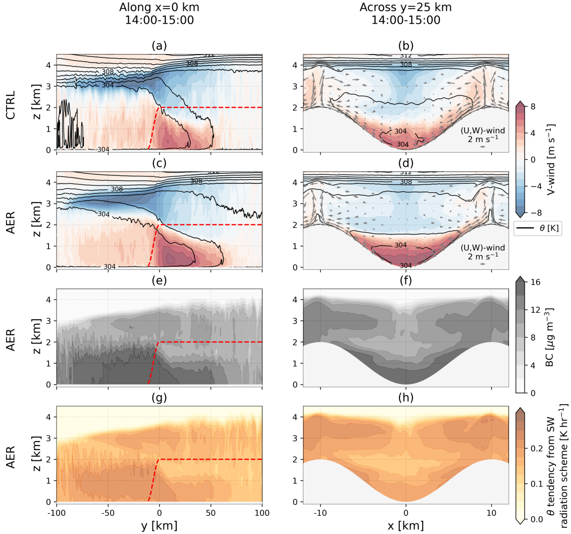
Figure 3. Cross-sections (a,c,e) (a,c,e,g) along the valley centre line and (b,d,f) (b,d,f,h) across the valley at y = 25 km averaged between 14:00 and 15:00. Panels (a-b) are from the case CTRL and panels (c-f) (c-h) are from the case AER. (a-d) Along-valley wind speed (shaded) and potential temperature (black solid lines). Positive along-valley wind speed refers to up-valley hence right-ward wind in (a,c) . (e-f) Black carbon concentration . (g-h) Potential temperature tendency from shortwave radiation scheme (shaded) and black carbon concentration (red solid lines, 2-interval). Grey-Red dashed line in (a,e,e) (a,c,e,g) show the ridge height at x = \pm 10 km.
