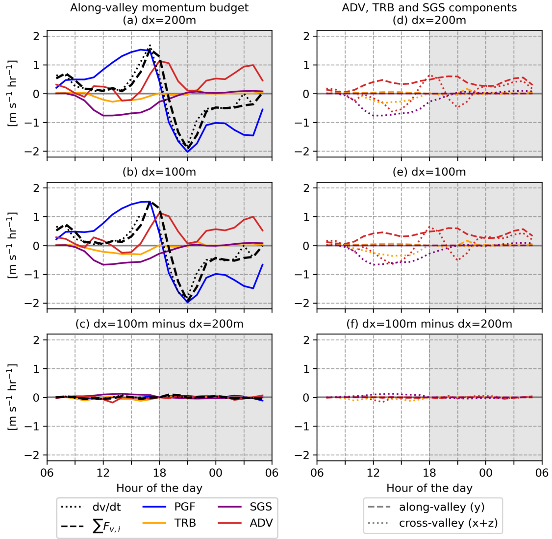
Figure S7. Along-valley momentum budget for the valley volume in (a) original CTRL and (b) sensitivity run with horizontal grid spacing of 100 m and (c) difference between the two cases. Left-hand-side of the Equation 3 in the manuscript for along-valley momentum is shown on black dotted line and the sum of the terms on the right-hand-side as black dashed line, respectively. (d-f) Same as (a-c) but for the tendency due to mean advection, resolved turbulence and sub-grid-scale diffusion decomposed into along and cross-valley components. The cross-valley component includes the vertical one.
