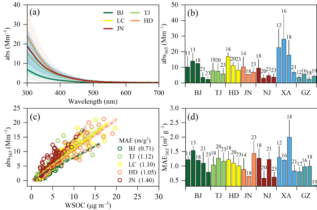
Figure 2 Optical properties of BrC at each sampling site. (a and c) Average absorption
