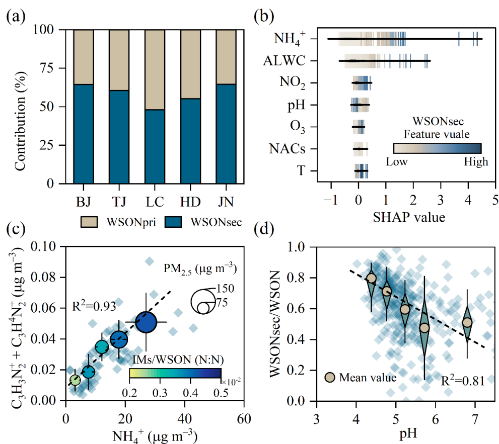
Figure 5 Aqueous formation of N-containing compounds in the NCP. Fractional
