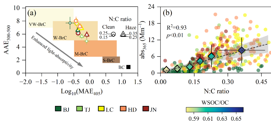
Figure 4 Graphical representation of optical-based BrC classes in log 10 (MAE 405 )-AAE space (a). The shaded regions represent very weakly light-absorbing BrC (VW-BrC), weakly light-absorbing BrC (W-BrC), moderately light-absorbing BrC (M-BrC), strongly light-absorbing BrC (S-BrC), and absorbing BC, respectively. (b) shows the linear fit regressions for abs 365 with N:C ratio (Diamonds indicate the averaged abs 365 and N:C ratio of all sites in each binned N:C interval, with bars representing standard deviations).
