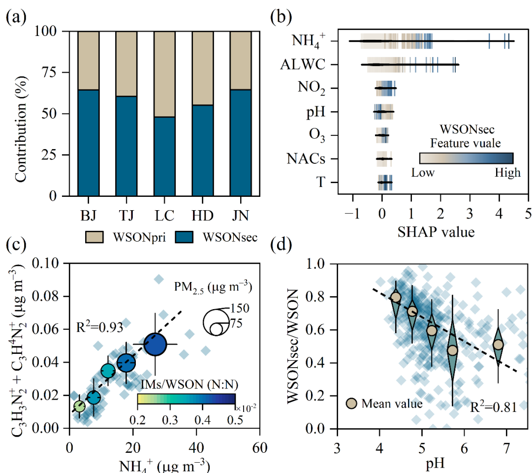
Figure 5 Aqueous formation of N-containing compounds in the NCP. Fractional contribution of primary water-soluble organic nitrogen (WSONpri) and secondary WSON (WSONsec) to the total (a); SHAP feature importance assessment for the key factors affecting WSONsec (b); Linear correlation between IMs-related fragments and \text{NH}_4^+ with different \text{PM}_{2.5} loads (The fragment signals do not represent absolute molecular abundances) (c); (d) show the linear fit regressions for \text{WSON}_{\text{sec}}/\text{WSON} with pH value across the NCP. (Circles in (c) and (d) show grouped mean statistics over all sampling site)
